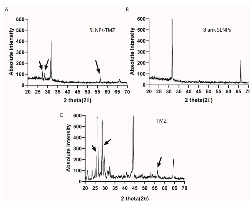
Figure 6. X-ray dispersive spectroscopy (XRD), (A) SLNP-TMZ, (B) Blank SLNP, (C) X-ray Patterns of TMZ. The sharp peak between 26^\circ and 28^\circ of SLNP-TMZ suggests the amorphous nature of TMZ after conjugation with SLNPs.
