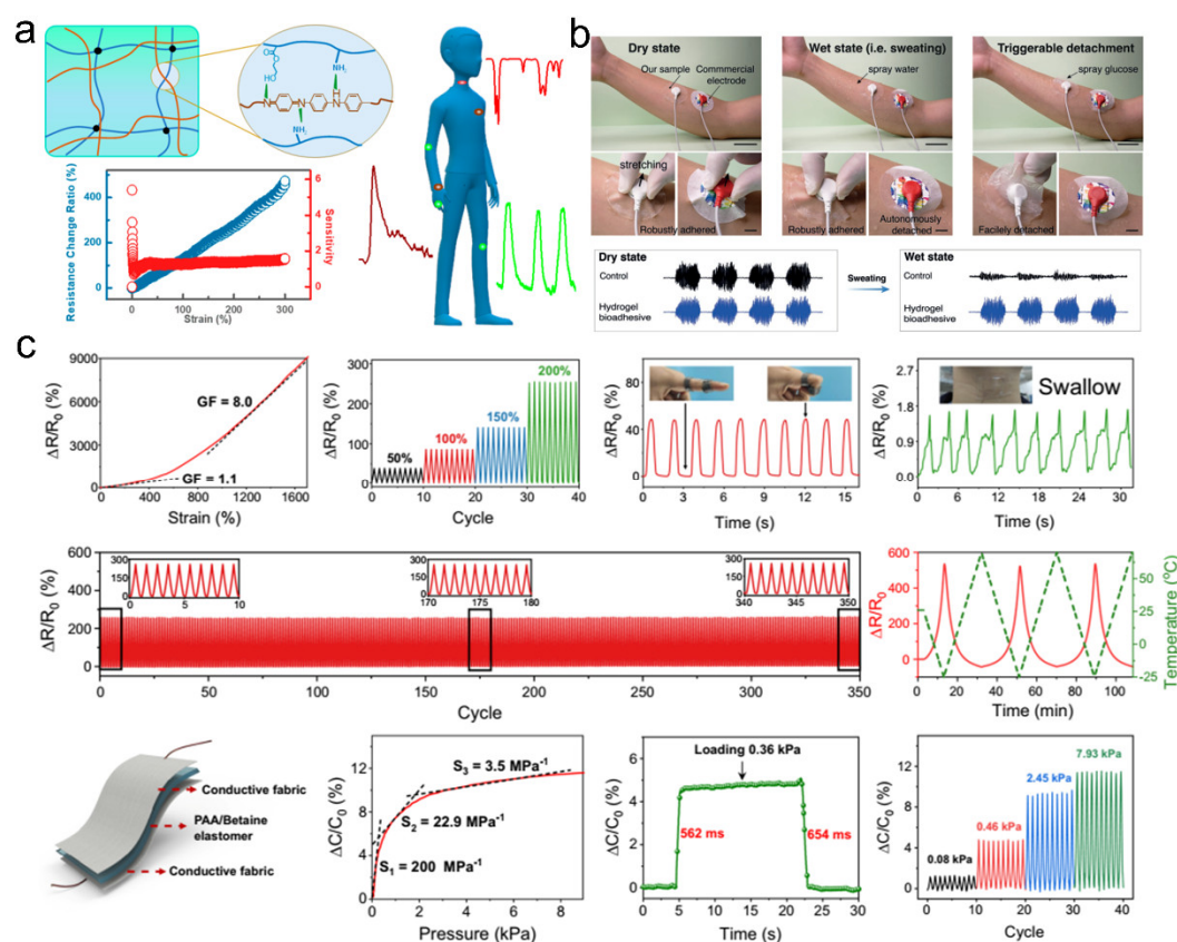
Figure 9. (a) The strain sensor for reliable detection of human activities by a tough and electrically conductive hydrogel, which comprised hydrogen-bonding-crosslinked PANI and P-(AAm-co-HEMA). Reproduced with permission [127]. Copyright 2018, American Chemical Society. (b) The physiological signal EMG was measured through a hydrogel adhesive with tough and reversible adhesion. Reproduced with permission [128]. Copyright 2021, John Wiley and Sons. (c) Multifunctional electronic devices for the detection of strain, pressure, and temperature signals on the human body.
