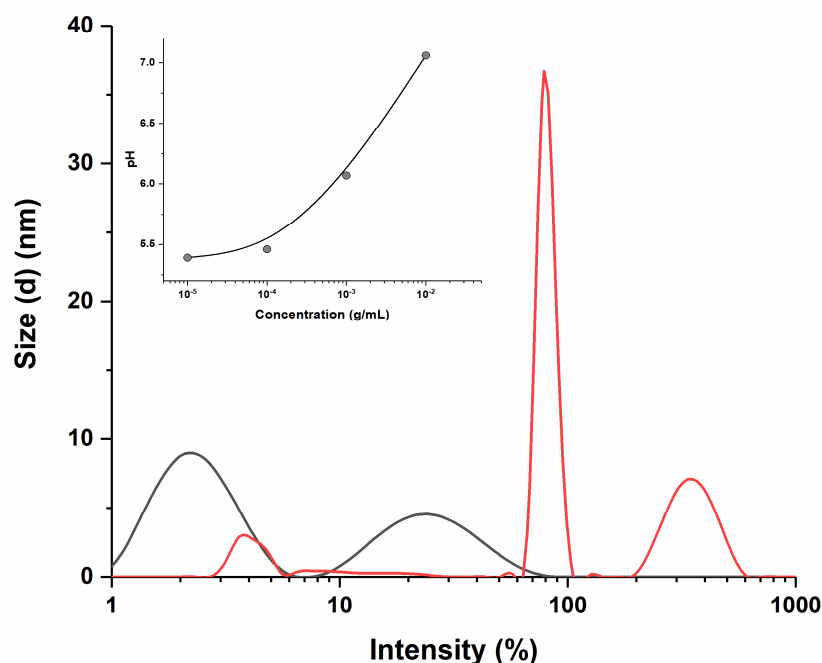
Figure 2. Particle size distribution in BSA colloid system depending on protein concentration (g/mL): red line— 1 \times 10^{-5} (0.15 \mu M), black line— 1 \times 10^{-2} (150 \mu M); pH dependance on concentration (g/mL) is shown in the insert.
