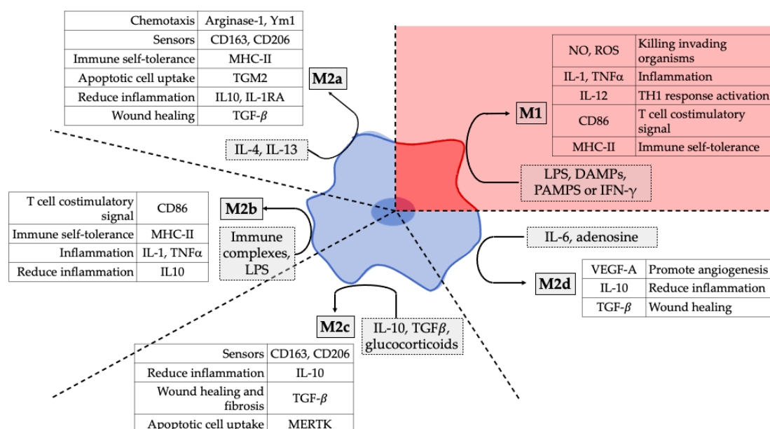
Figure 1. Overview of macrophage phenotypes. The figure shows the phenotypical division of macrophages in M1 and M2 phenotype and the subcategories of M2 macrophages (M2a, M2b, M2c, M2c). It also shows the markers expressed by the different macrophage phenotypes upon activation by different stimuli and their functions. CD: Cluster of differentiation; LPS: lipopolysaccharide; MHC-II: Major histocompatibility complex—II; TGM2: Transglutaminase 2 (TGM2); IL: Interleukin; IL-1RA: interleukin 1 receptor antagonist; TGF- \beta : tumor growth factor beta; TNF \alpha : tumor necrosis factor alpha; ECM: extracellular matrix; MERTK: MER Proto-Oncogene Tyrosine Kinase; NOS: Nitrogen oxide species; ROS: Reactive oxygen species; DAMP: damage-associated molecular patterns; PAMP: pathogen molecular patterns; IFN- \gamma : Interferon gamma; VEGF-A: Vascular endothelial growth factor.
