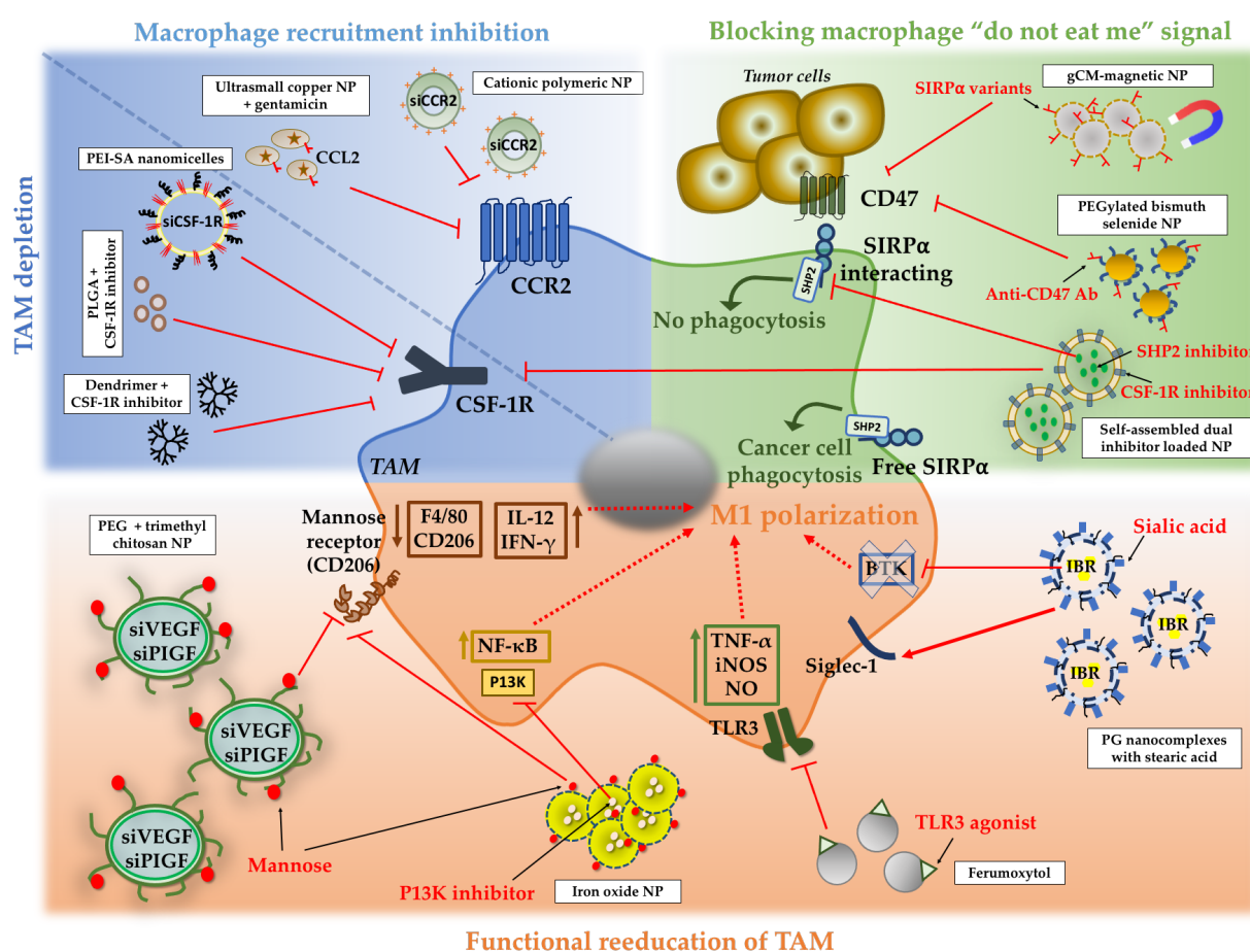
Figure 6. Strategies for the targeting of TAM using NPs. Four main strategies have been described for TAM-targeted therapies: (1) inhibition of macrophage recruitment to the tumor (blue); (2) TAM depletion in the tumor microenvironment (blue); (3) blockade of macrophage immune checkpoint (“do not eat me” signal) (green); and (4) functional re-education of TAM to a M1 phenotype (orange). The image illustrates different molecular targets and different types of NPs that have been described to treat TAM. NP: nanoparticles; PEI-SA: polyethylenimine and stearic acid; PLGA: poly (lactic-co-glycolic acid); CSF-1R: Colony stimulating factor 1 receptor; TAM: tumor-associated macrophages; CCR2: C-C Motif Chemokine Receptor 2; SHP2: Src homology region 2 phosphatases; SIRPα: macrophage signal-regulatory protein alpha; Ab: antibody; gCM: genetically engineered cell membrane; PEG: polyethylene glycol; VEGF: vascular endothelial growth factor; PIGF: placental growth factor; IFNγ: interferon γ; NF-κB: nuclear factor kappa-light-chain-enhancer of activated B cells; P13K: Phosphoinositide 3-kinases; TNF-α: tumor necrosis factor; iNOS: nitric oxide synthases; NO: nitric oxide; TLR: toll-like receptor; IBR: Ibrutinib; BTK: Bruton’s tyrosine kinase.
