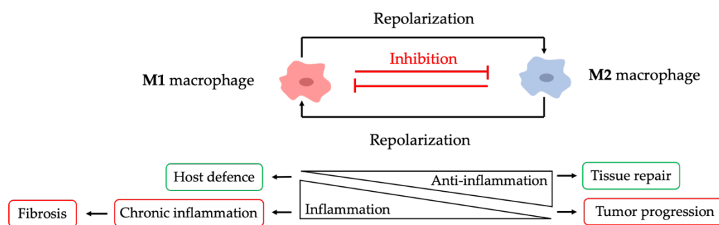
Figure 3. Macrophage roles on host defense. Macrophages are commonly divided into two phenotypes: M1 and M2 macrophages. These phenotypes are reversible, and macrophages can be re-programmed depending on the local stimuli. The inflammatory and anti-inflammatory responses carried out by macrophages need to be well balanced to prevent disease. Uncontrolled M1 macrophage activation can lead to chronic inflammation and un-controlled M2 macrophage activation can lead to tumour progression.
