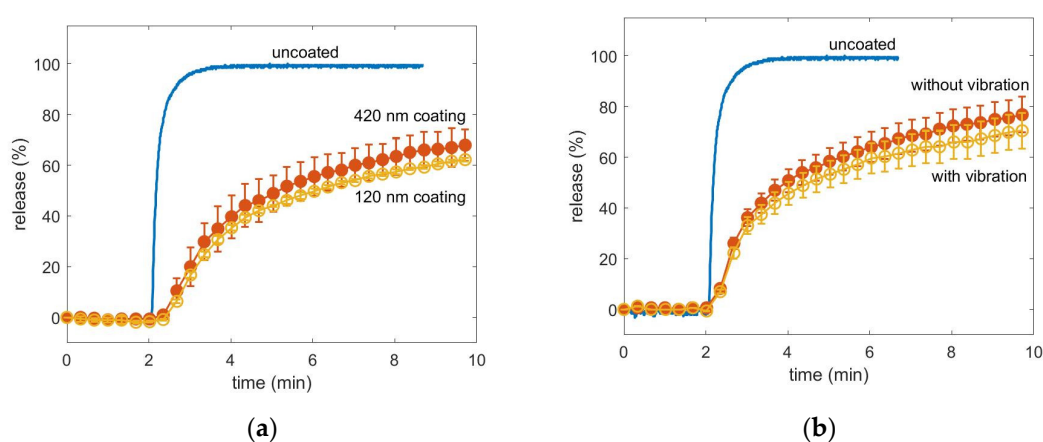
Figure 5. (a) Release curve of magnesium citrate coated with a nominal coating thickness of 420 nm and a nominal coating thickness of 120 nm polymer of p-EGDMA. Samples were placed on the reactor bottom as in Figure 1b. (b) release curve of magnesium powder coated with and without vibration both with a nominal thickness of 210 nm. Samples were placed on speakers as in Figure 1c.
