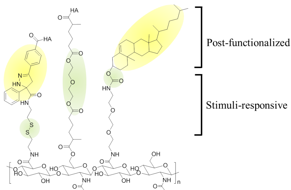
Figure 6. Chemical modification of hyaluronic acid (HA) with (1) functionality groups and (2) stimuli-responsive moieties. Photo-crosslinking between tetrazole and methacrylate generates a durable nanogel structure, while disulfide bonds endows degradability to nanogels under reductive condition (Left). A crosslinker functions as not only the precursor of the nanogel, but also enzyme-responsive moiety, such as ester group (Middle). To make the nanogels using hydrophilic HA, a hydrophobic moiety can be post-functionalized on the backbone. (i.e., cholesterol) (Right).
