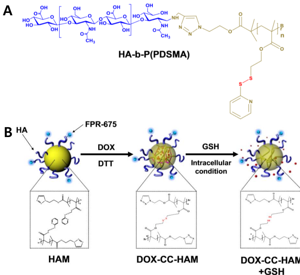
Figure 3. Redox-responsive hydrophobic polymer grafted hyaluronic acid (HA) polymeric micelles. (A) Chemical structure of HA-poly(pyridyl disulfide methacrylate (HA-b-P(PDSMA))), and (B) schematic illustration of crosslinked HA polymeric micelles with doxorubicin (Dox). GSH: Glutathione; CC-HAM; core-crosslinked polymeric micelles based on HA. Reproduced from [27] with permission. Copyright 2015 Elsevier Ltd.
