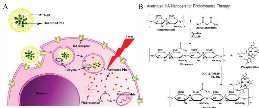
Figure 10. (A) Schematic representation of photosensitizer, pheophorbide (Pba), quenchable hyaluronic acid (HA)-based nanogels and single oxygen generation induced by Pba activation under UV irradiation. (B) Synthetic scheme of acetylated HA nanogels further conjugated with Pba. Reproduced from [59] with permission. Copyright (2010) American Chemical Society. DCC: N,N'-Dicyclohexylcarbodiimide; DMAP: 4-Dimethylaminopyridine.
