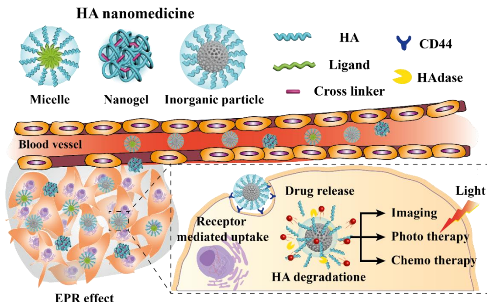
Figure 1. Schematic representation of the advantages and applications of hyaluronic acid (HA). EPR: Enhanced Permeability and Retention; CD44: Cluster Determinant 44.
