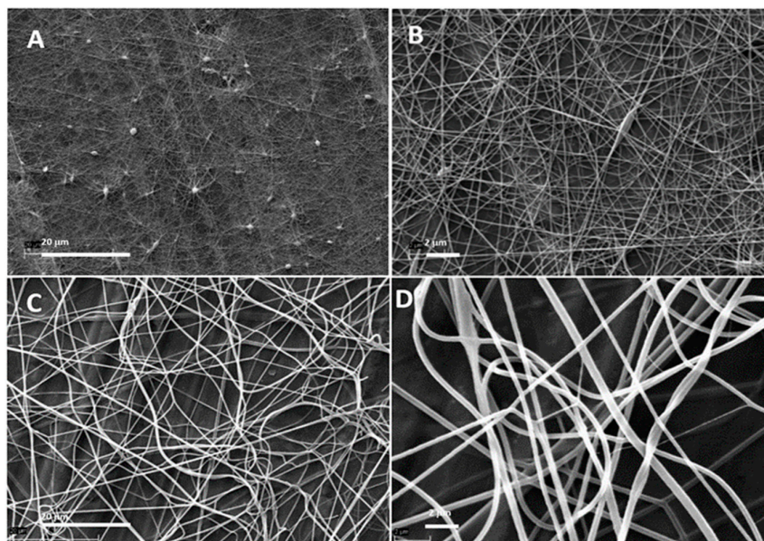
Figure 2. Scanning electron microscopy (SEM) images of traditional electrospun (TES) and ultrasound-enhanced electrospun (USES) nanofibers. (A, B) TES nanofibers (magnification 2500× and 10,000×); (C, D) USES nanofibers (2500× and 10,000×).
