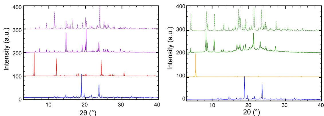
Figure 1. Powder X-ray diffraction (PXRD) patterns of benexate hydrochloride (BEX-HCl) (blue), sodium saccharinate (red), benexate-saccharinate (BEX-SAC) (purple), sodium cyclamate (yellow), and benexate-cyclamate (BEX-CYM) (green). The solid and dashed lines represent the experimental and simulated PXRD patterns, respectively.
