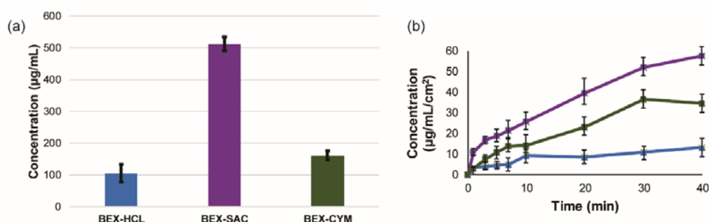
Figure 7. (a) The solubility and (b) intrinsic dissolution rate of BEX–HCL (blue), BEX–SAC (purple), and BEX–CYM (green). Solubility and dissolution rate experiments were conducted in triplicate.
