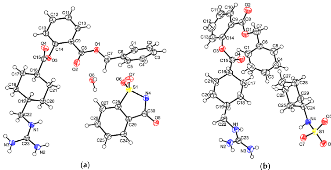
Figure 3. Thermal ellipsoid figures of (a) BEX-SAC and (b) BEX-CYM are drawn at the 50% probability level. The asymmetric unit of BEX-SAC contained a cationic benexate, an anionic saccharinate, and a water molecule. The asymmetric unit of BEX-CYM contained one cationic benexate molecule and one anionic cyclamate molecule.
