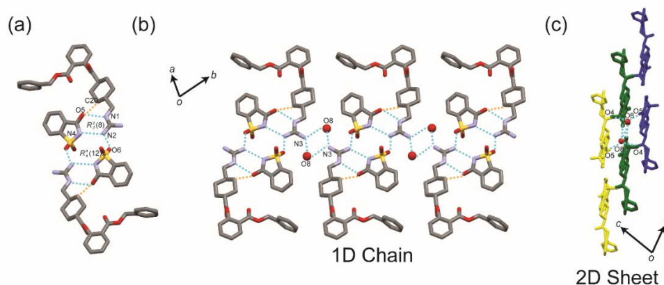
Figure 4. The hydrogen bond architecture in the BEX–SAC crystal. (a) The interaction involving two sets of cationic benexate and anionic saccharinate molecules and water constructs. (b) 1D chain structures parallel to the (110) plane. Each 1D chain (represented by different colors) interacts with each other to form (c) a 2D sheet structure. Conventional and non-conventional hydrogen bonds are drawn by dashed blue and orange lines, respectively. Hydrogen atoms have been omitted for clarity. The oxygen atoms from water molecules are drawn in ball-setting.
