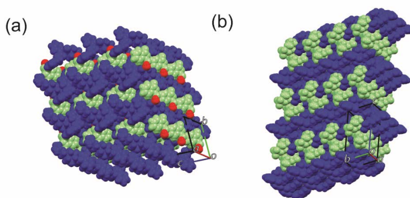
Figure 6. Packing view of (a) BEX–SAC and (b) BEX–CYM. All molecules are drawn in a space-fill setting. Cationic benexate, anionic salt co-former, and water molecules are represented by dark blue, light green, and red molecules, respectively.
