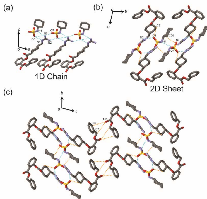
Figure 5. (a) 1D chain and (b) 2D sheet structures in the BEX–CYM crystal. (c) The 2D sheet structure is stacked along the a -axis through C5–H...O2 and C7–H...O2 hydrogen bonds. Conventional and non-conventional hydrogen bonds are drawn by dashed blue and orange lines, respectively. Hydrogen atoms have been omitted for clarity.
