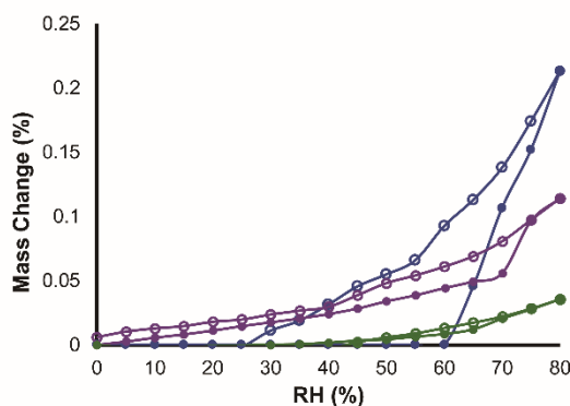
Figure 8. Water sorption–desorption of BEX–HCl (blue), BEX–SAC (purple), and BEX–CYM (green). The closed and open symbols represent sorption and desorption, respectively.
