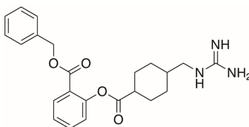
Scheme 1. The molecular structure of benexate (BEX).
