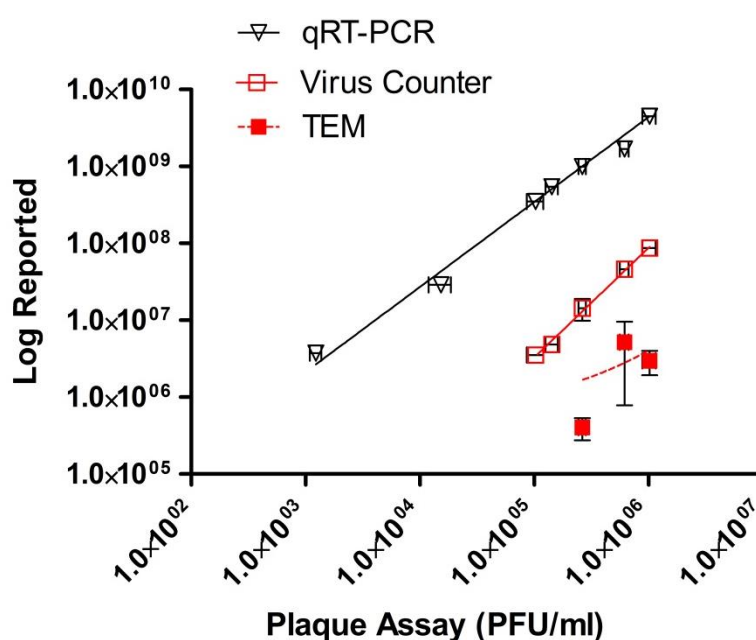
Figure 2. Log-log plot of dilution versus reported concentration for a series of Ebola virus (EBOV), Kikwit variant, samples produced by diluting the stock virus. Infectious virus was quantified for each sample using six well plates of confluent Vero E-6 cells and an agarose-based plaque assay (PFU/mL). All samples were tested in six replicates; bars represent standard deviation. Genomic equivalents were quantified for each sample using an EBOV-specific qRT-PCR (GE/mL). All samples were tested in triplicate; bars represent standard deviation. Virus particles concentration (VP/mL) was quantified from each sample using transmission electron microscopy (TEM). All samples were tested in triplicate. Bars represent standard deviation. Virus particle concentration was also quantified for each sample using the ViroCyt ® Virus Counter 2100 instrument. All samples were tested in triplicate; bars represent standard deviation.
