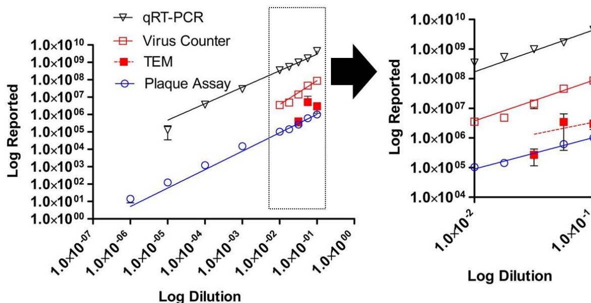
Figure 2. Log-log plot of dilution versus reported concentration for a series of Ebola virus (EBOV), Kikwit variant, samples produced by diluting the stock virus. Infectious virus was quantified for each sample using six well plates of confluent Vero E-6 cells and an agarose-based plaque assay (PFU/mL). All samples were tested in six replicates; bars represent standard deviation. Genomic equivalents were quantified for each sample using an EBOV-specific qRT-PCR (GE/mL). All samples were tested in triplicate; bars represent standard deviation. Virus particles concentration (VP/mL) was quantified from each sample using transmission electron microscopy (TEM). All samples were tested in triplicate. Bars represent standard deviation. Virus particle concentration was also quantified for each sample using the ViroCyt ® Virus Counter 2100 instrument. All samples were tested in triplicate; bars represent standard deviation.
