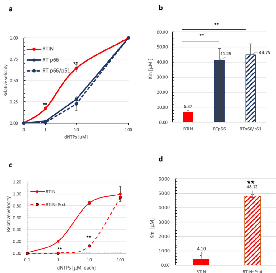
Figure 4. Impact of IN fusion on affinity of RT to dNTPs. (a) A reaction was performed in the presence of different doses of dNTPs (0.1, 1, 10, 100 \mu\text{M} ) with a fixed vRNA dose (100 ng/reaction) and RTIN or RTs. The R/u5 copy number generated during 60 min incubation was measured, and the value at each dose was plotted as a velocity relative to the reaction with 100 \mu\text{M} of dNTPs as 1.0. The value at each dNTP dose is shown as means \pm SD ( n = 3 ). (b) The K_m for dNTPs was estimated by calculating velocity at 100 \mu\text{M} dNTPs as the maximum velocity in the assay condition. The K_m value of each protein is indicated on the top of each bar. Student's t analysis showed significant differences between RTIN and either RTp66 or RTp66/p51 (** p > 0.01 , n = 4 ). (c) Effect of protease cleavage of RTIN. rRTIN with or without digestion with HIV-1 protease was subjected to reaction, and data are plotted as described for a. (d) The K_m for dNTPs was estimated by calculating velocity at 100 \mu\text{M} dNTPs as the maximum of velocity in the assay condition. The K_m value of each protein is indicated on the top of each bar. Student's t analysis showed significant differences between rRTIN with and without protease treatment (** p > 0.01 , n = 4 ).
