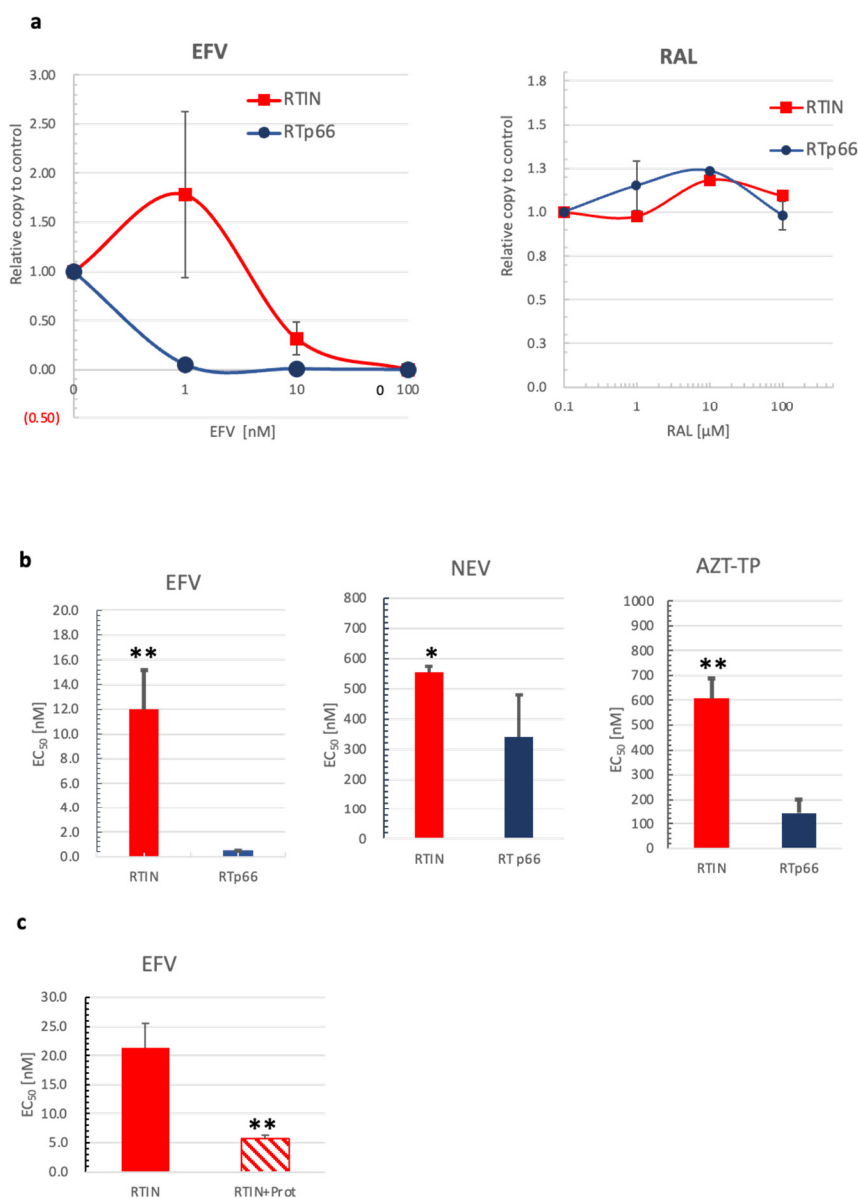
Figure 5. Effect of IN fusion on sensitivity to RT inhibitors. (a) An in vitro reverse transcription assay was performed in the presence of different concentrations of efavirenz (EFV) or raltegravir (RAL). Levels of R/u5 products were measured and are shown as values relative to the level with solvent (DMSO) only as 1.0. (b) The effective concentration 50 (EC 50 ) of EFV, nevirapine (NEV), or 3′-Azido-2′,3′-dideoxythymidine-5′-triphosphate (AZT-TP) for RTIN or RTp66 was determined by calculating the drug concentration to inhibit 50% of RDDP activity relative to control. Student’s t analysis showed significant differences between rRTIN and RTp66 (** p > 0.01, * p > 0.05, n = 3). (c) The effect of cleavage by HIV-1 protease on the EFV sensitivity of RTIN was examined as described in a. The EC 50 of EFV for rRTIN with or without pretreatment with HIV-1 protease is shown. Student’s t analysis showed that rRTIN had significant effect on EC 50 by pretreatment with HIV-1 protease (** p > 0.01, n = 3).
