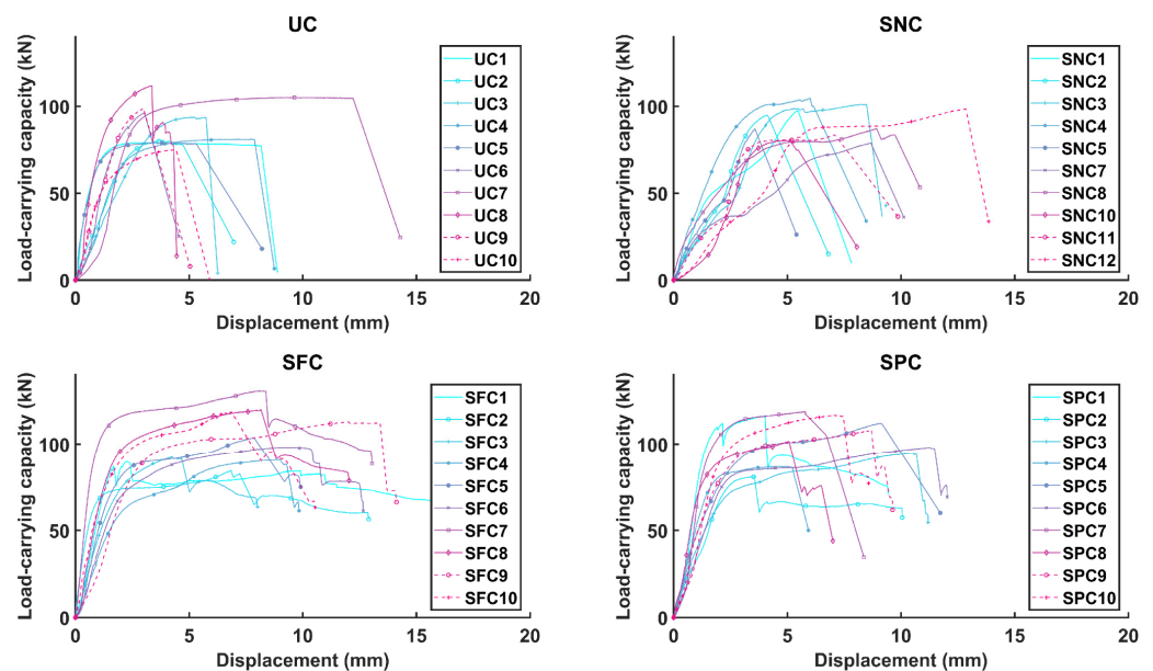
Figure 10. Load-displacement curves for each group in this study.
