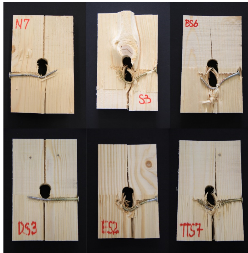
Figure 8. Specimens from each reinforced group after the embedment-strength test: high level of deformation of screw and embedment of screw head can be seen in groups S, BS, ES and TTS [31].
