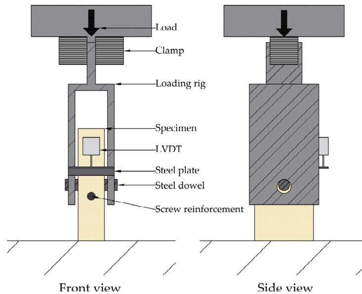
Figure 2. Embedment-strength test set-up.
