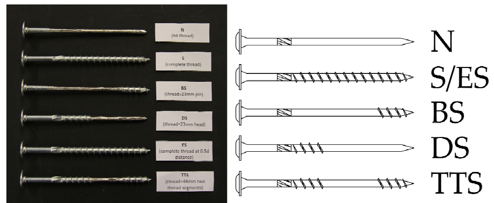
Figure 3. Screws with different thread lengths.
