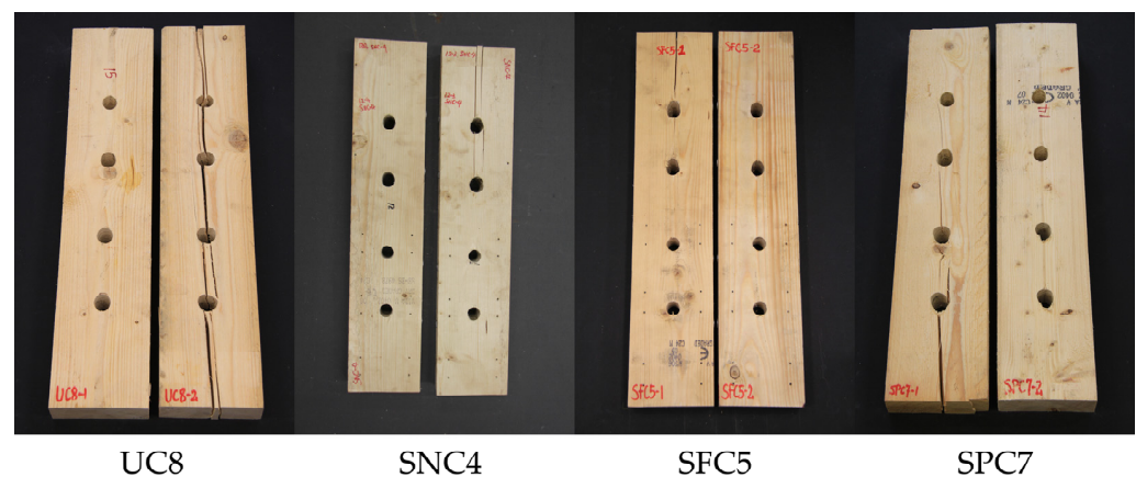
Figure 12. Demonstration of specimen failures in each group.
