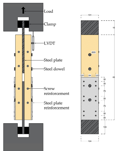
Figure 4. Specimen set-up (left) and dimensions for the specimen (right).
