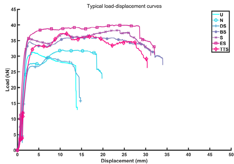
Figure 9. Load-displacement curves for embedment-strength tests.
