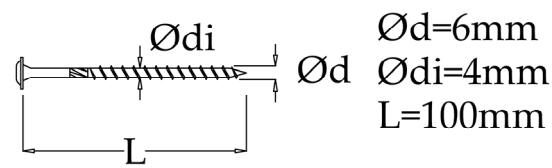
Figure 1. Flange-head partially threaded self-tapping screw used in this study.
