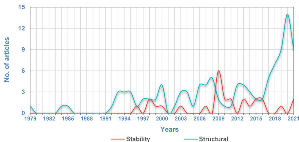
Figure 2. Trend in the annual distribution of literature related to the structure and stability of agroforestry ecosystems.
