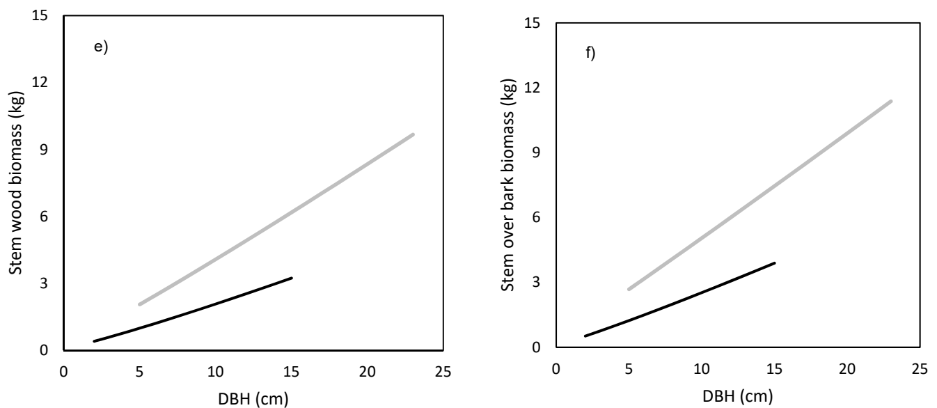
Figure 7. Comparison of modeled annual production of aboveground tree biomass (a), foliage biomass (b) branches (c), stem bark (d), stem wood (e) and stem over bark (f) between silver birch and Norway spruce. We considered real values of mean annual diameter increment for each species, i.e., 1.4 and 1.0 cm for birch and spruce, respectively.
