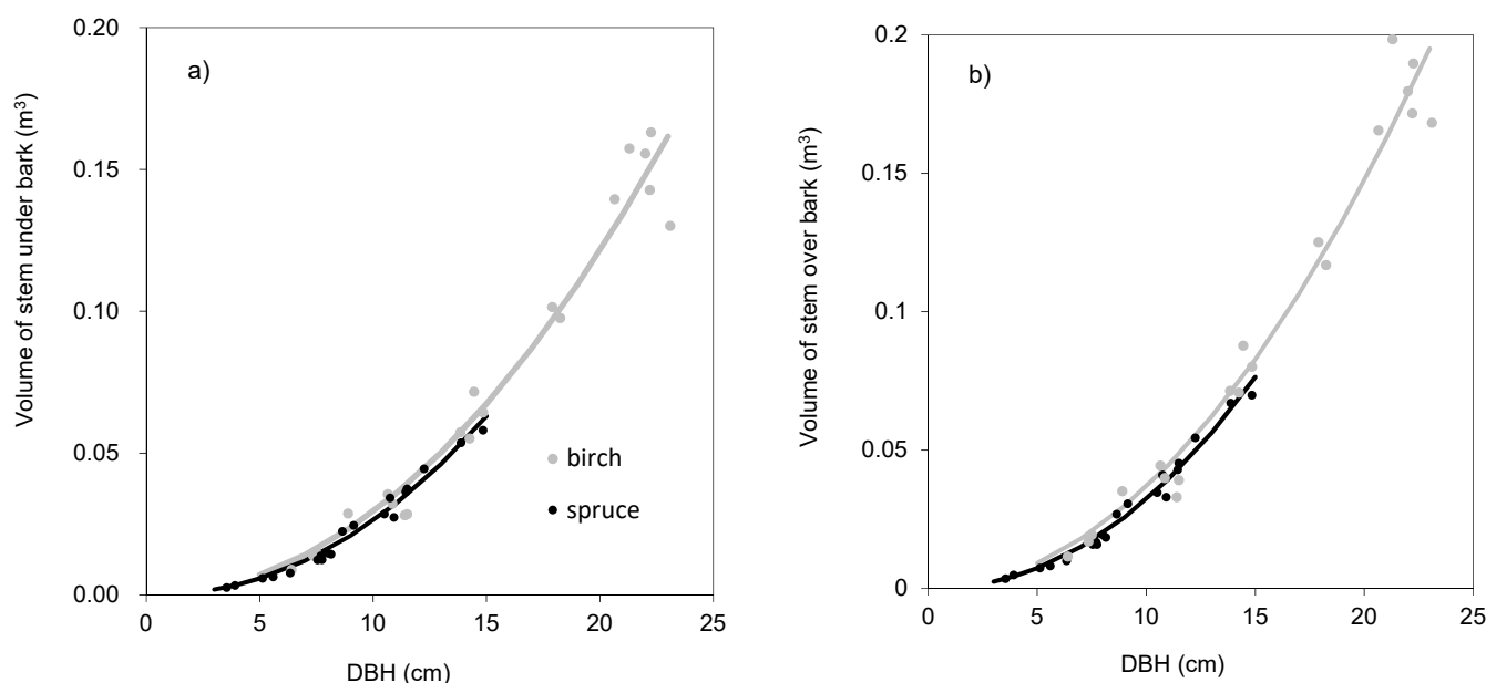
Figure 2. Relationship between DBH and stem volume under bark (a) and stem volume over bark (b) for silver birch and Norway spruce. See also Tables 5 and 6 for more details on the models.
