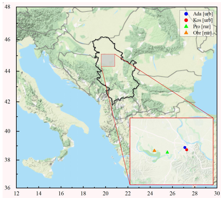
Figure S1. Map of the investigated localities.
