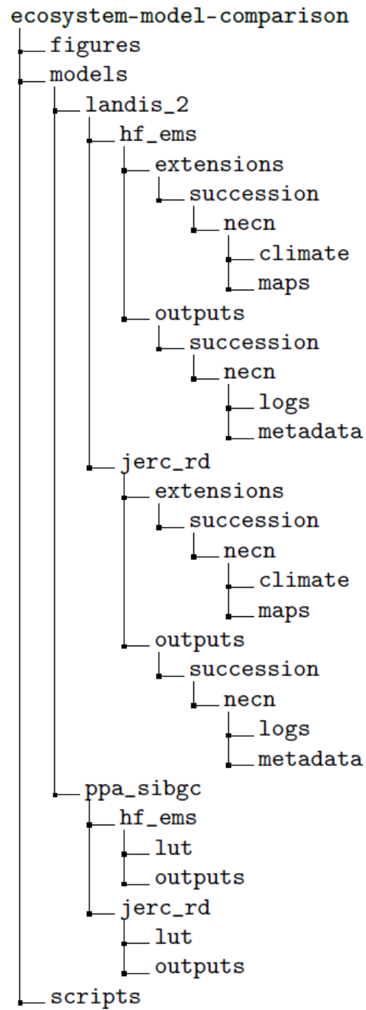
Figure S1. Directory structure of the GitHub repository.
