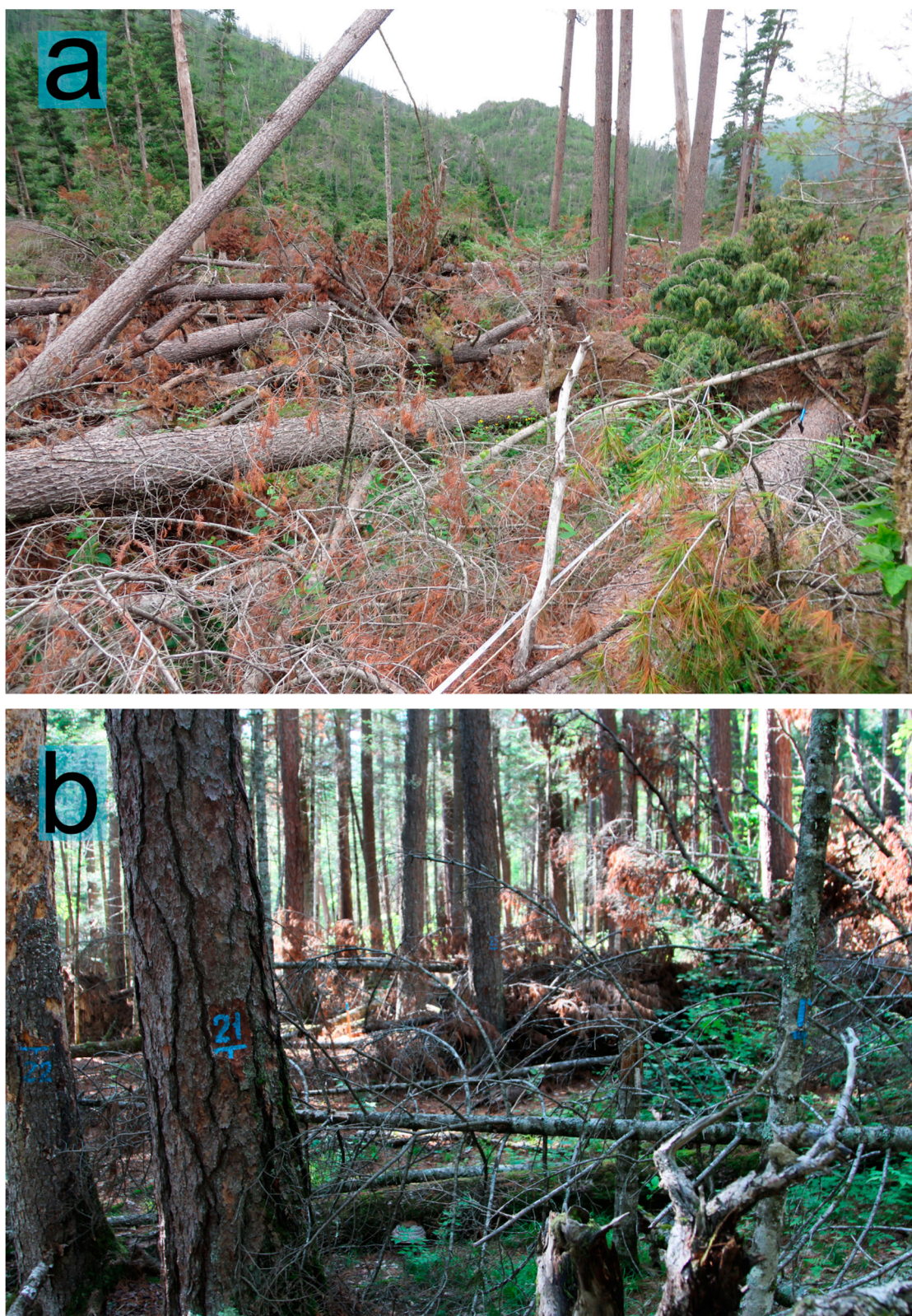
Figure S2. The character of wind-caused tree damage at PP1 (a) and PP2 (b).
