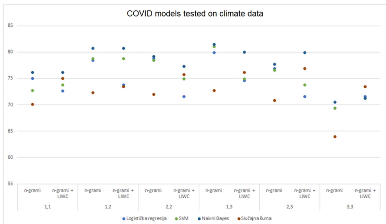
Figure 8. Models trained on DS2 (COVID-19 dataset) and tested on DS1 (climate dataset).
