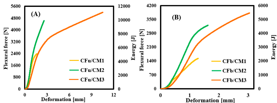
Figure 8. Total flexural energy–deformation profiles of (A) CFu/CM and (B) CFb/CM specimens.
