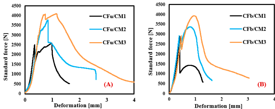
Figure 7. Flexural load–deformation profiles of (A) CFu/CM, and (B) CFb/CM specimens.
