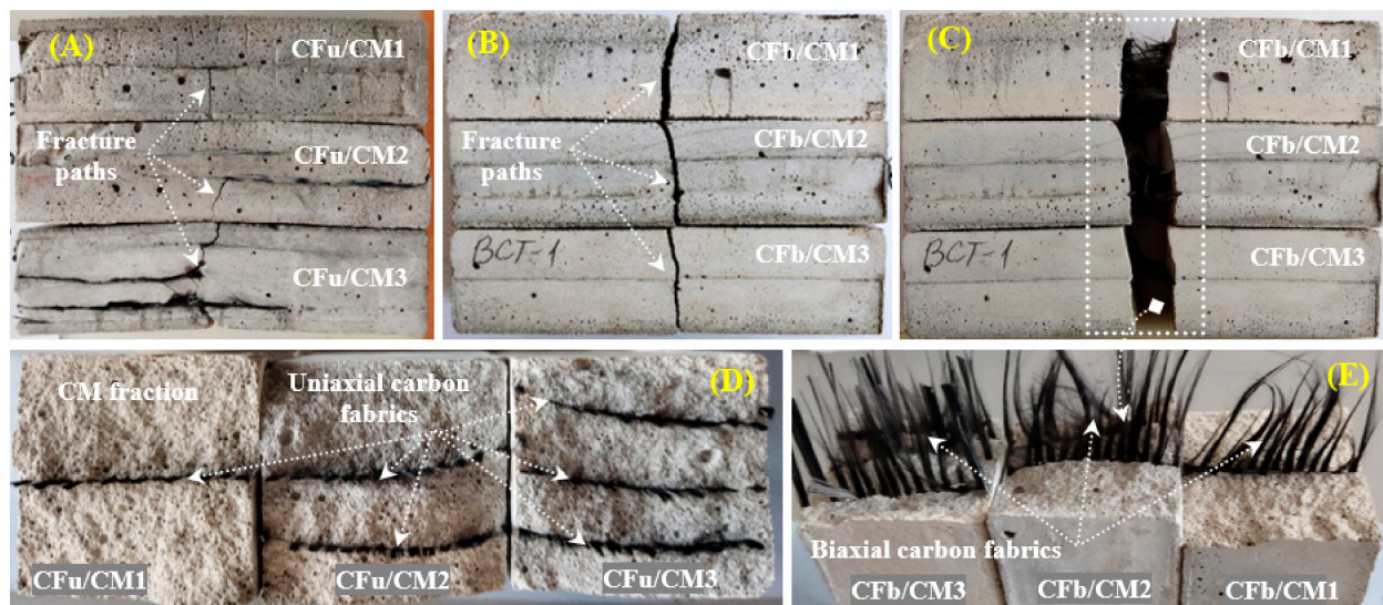
Figure 5. Photographs of (A–C) fracture paths of CF/CM specimens and (D,E) cross-section features of CF/CM specimens.
