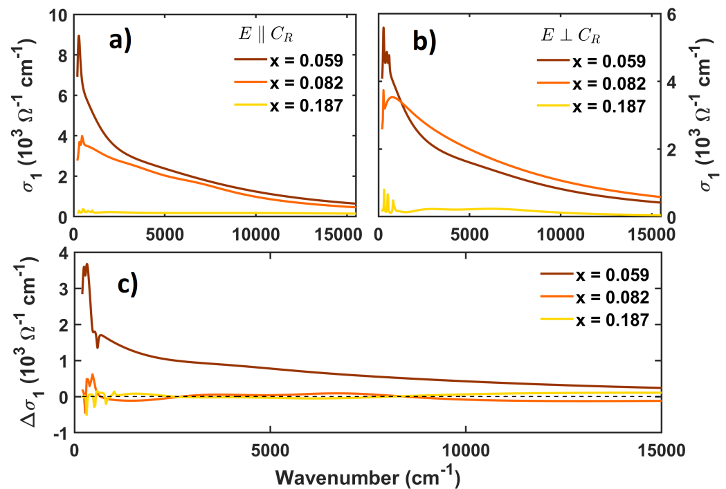
Figure 2. Real part of the optical conductivity of \text{Ti}_x\text{V}_{1-x}\text{O}_2 single crystals in the R phase obtained with polarization (a) parallel and (b) orthogonal to the growth axis, c_R . Brown, orange, and yellow lines denote Ti doping with x = 0.059 , x = 0.082 , and x = 0.187 , respectively. (c) Difference between the real part of the optical conductivities obtained with parallel and orthogonal polarization under fixed doping, as defined in Equation (1).
