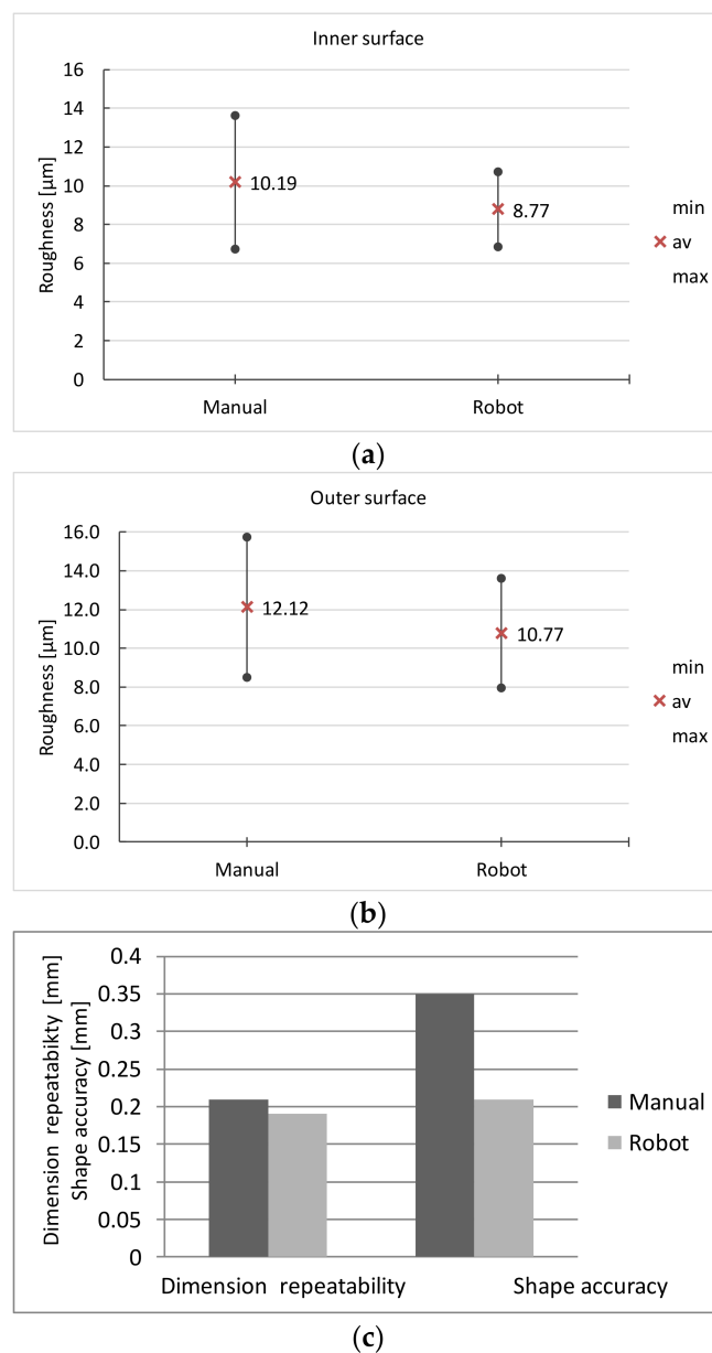
Figure 14. Comparison of: (a,b) surface roughness and (c) dimensional repeatability and shape accuracy obtained with manual and robot grinding.
