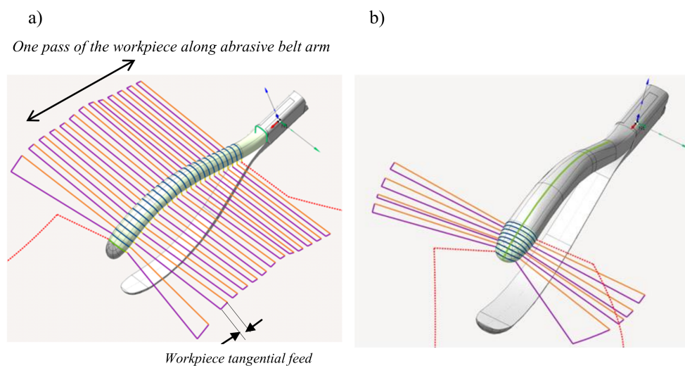
Figure 9. Grinding strategy: (a) of the outer surface; (b) of the tip of the workpiece.
