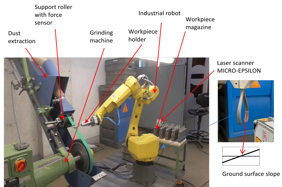
Figure 7. Research stand for belt grinding with the use of an industrial robot.
