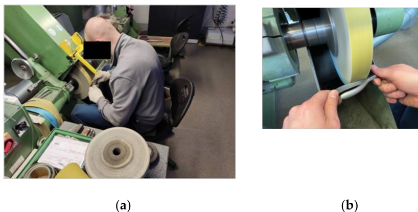
Figure 2. Manual belt grinding station: (a) overall view; (b) working area.
