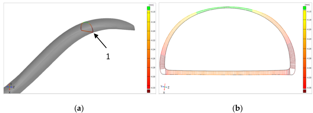
Figure 6. The idea of determining the shape deviation of the cross-section of the forceps arm: (a) location (1) of the cross-section along the length of the arm; (b) map of deviations between the reference profile (CAD profile) and the profile obtained after the grinding process.
