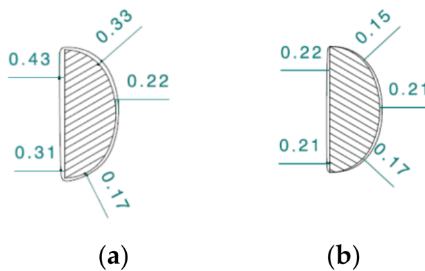
Figure 15. Shape error in cross-section of the forceps arm after: (a) manual grinding and (b) grinding with the use of robot.
