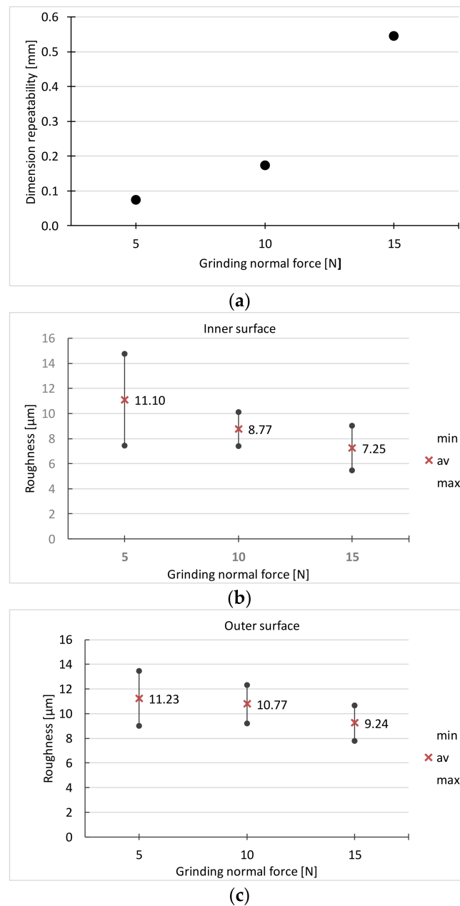
Figure 11. Dependence on the grinding force of: (a) dimensional repeatability, (b,c) surface roughness ( v_s = 26 m/s; v_f = 4 mm/s).
