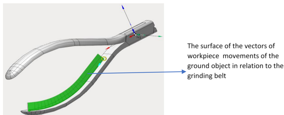
Figure 8. Grinding strategy of the inner surface of the workpiece.
