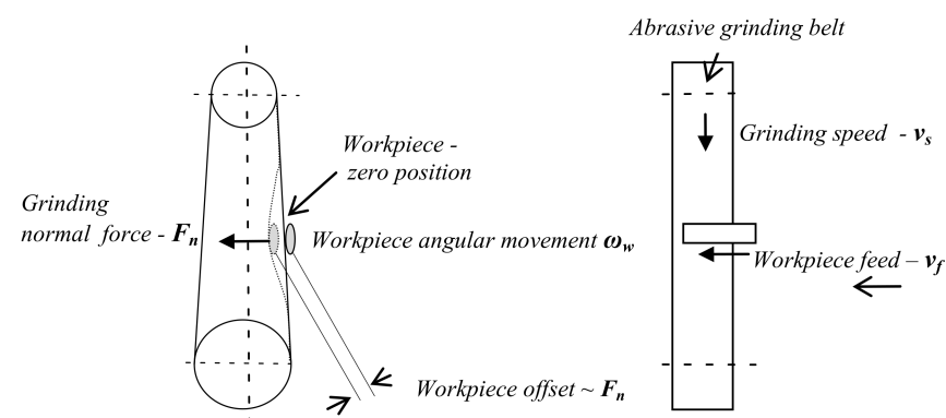
Figure 10. Robotic belt grinding parameters.
