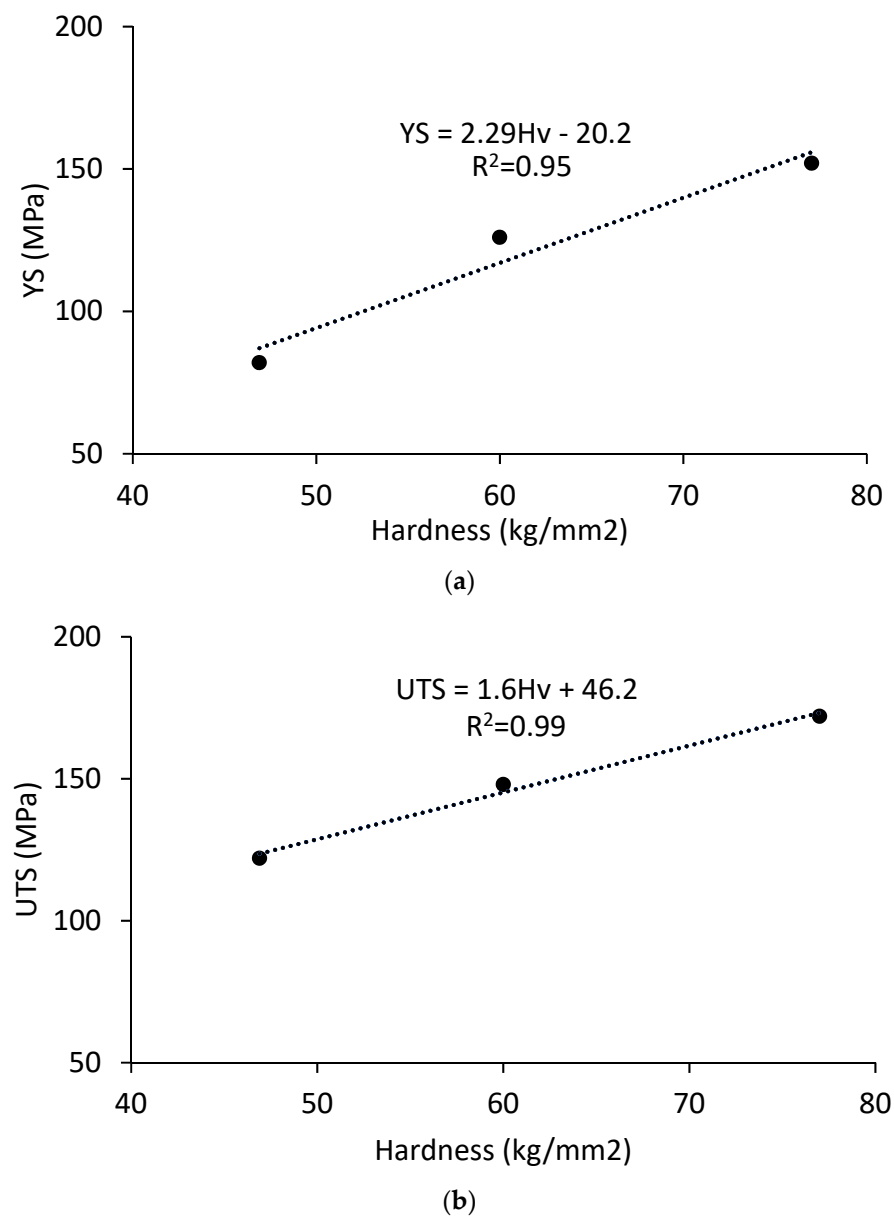
Figure 15. Correlations between hardness and (a) yield strength and (b) ultimate strength for the \text{Al}_3\text{Hf} -Al MMCs at room temperature in the unirradiated condition.
