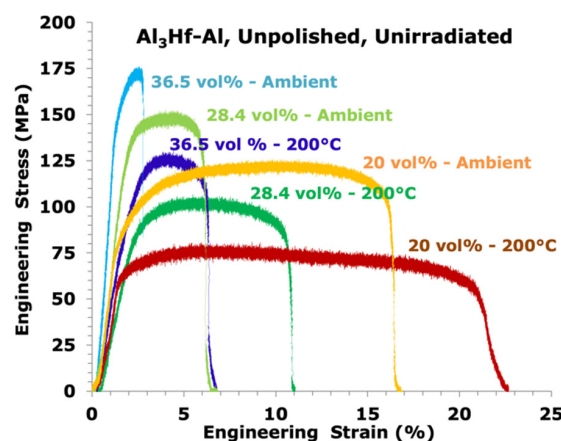
Figure 9. Engineering stress vs. strain curves of \text{Al}_3\text{Hf} -Al as a function of \text{Al}_3\text{Hf} volume fraction for the unirradiated specimens.
