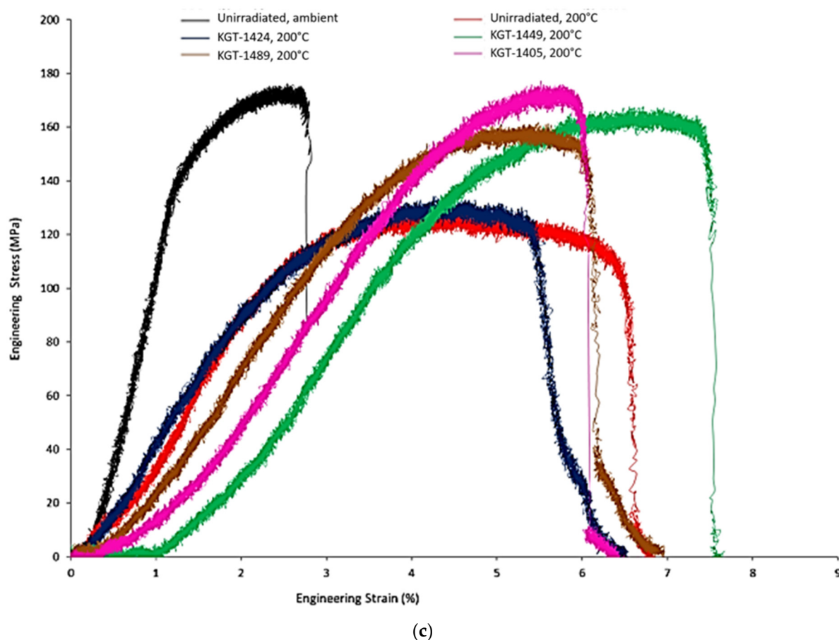
Figure 12. Engineering stress vs. strain curves of \text{Al}_3\text{Hf-Al} as a function of \text{Al}_3\text{Hf} volume fraction, test temperature and KGT identifier (a) 20.0 vol%, (b) 28.4 vol%, and (c) 36.5 vol%.
