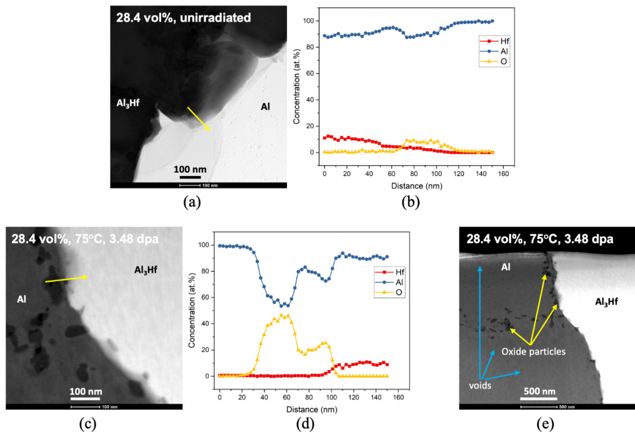
Figure 25. (a,b) BF STEM images and corresponding EDS linescans for unirradiated 28.4 vol% \text{Al}_3\text{Hf} -Al (arrow indicates direction of the linescan), (c,d) A STEM Z-contrast image and corresponding EDS linescan for irradiated 28.4 vol% \text{Al}_3\text{Hf} -Al from KGT-1404 (arrow indicates direction of the linescan), (e) A STEM Z-contrast image of irradiated \text{Al}_3\text{Hf} -Al to show all the features identified.
