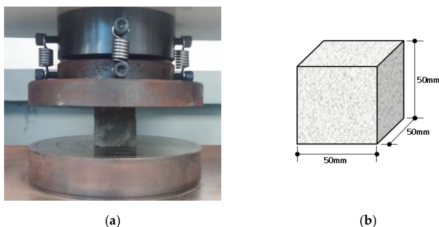
Figure 2. Slump-flow test: (a) Test setup; (b) Cube specimen.
