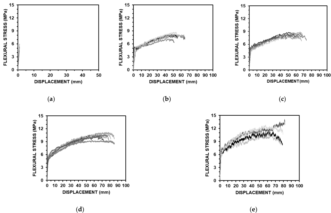
Figure 9. Flexural stress–displacement curves: (a) ASFC000 (PVA 0.00 vol.%); (b) ASFC100 (PVA 1.00 vol.%); (c) ASFC125 (PVA 1.25 vol.%); (d) ASFC150 (PVA 1.50 vol.%); (e) ASFC200 (PVA 2.00 vol.%).
