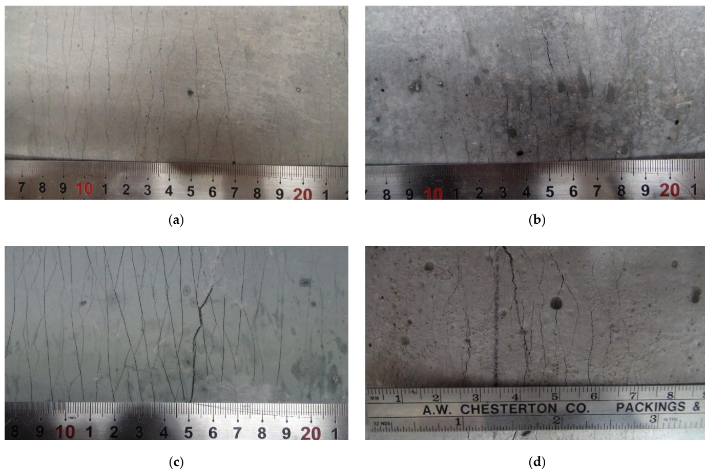
Figure 11. Multiple microcracks in bending panel: (a) ASFC100 (PVA 1.00 vol.%); (b) ASFC125 (PVA 1.25 vol.%); (c) ASFC150 (PVA 1.50 vol.%); (d) ASFC200 (PVA 2.00 vol.%).
