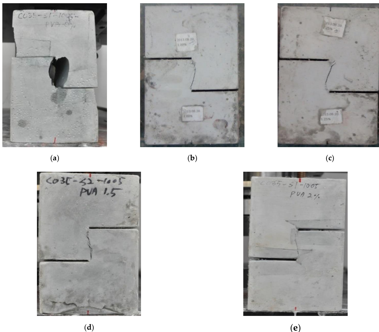
Figure 12. Failure of shear specimens: (a) ASFC000 (PVA 0.00 vol.%); (b) ASFC100 (PVA 1.00 vol.%); (c) ASFC125 (PVA 1.25 vol.%); (d) ASFC150 (PVA 1.50 vol.%); (e) ASFC200 (PVA 2.00 vol.%).
