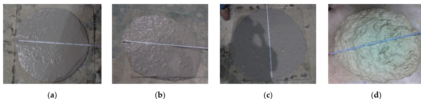
Figure 1. Slump-flow test: (a) ASFC100; (b) ASFC125; (c) ASFC150; (d) ASFC200.
