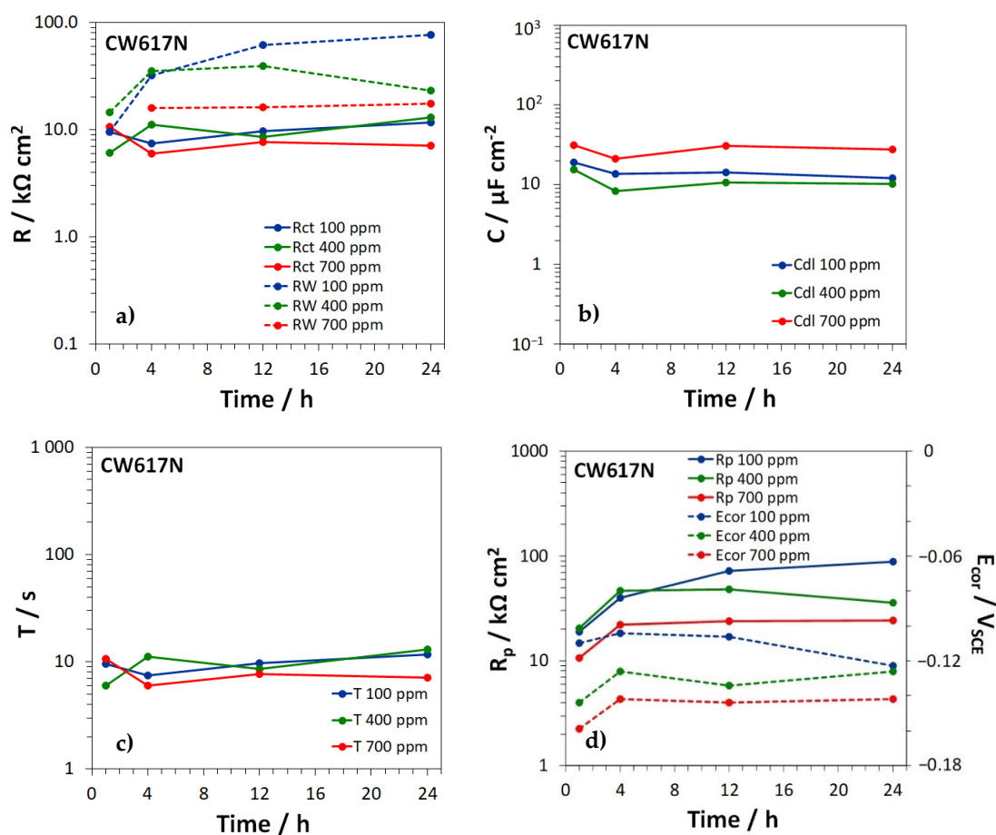
Figure 8. Time dependence of (a) the charge transfer and diffusion resistances ( R_{ct} and R_W ); (b) the double layer capacitance ( C_{dl} ); (c) the T parameter of the GFLW element; and (d) the polarization resistance ( R_p ) and corrosion potential values ( E_{cor} ), measured on CW617N during the immersion in SDW with three different chloride concentrations.
