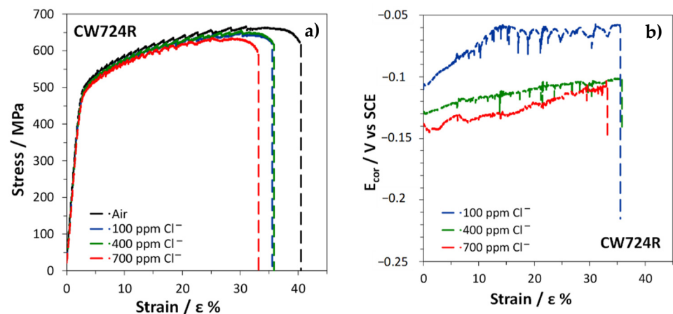
Figure 18. SSRT on CW724R: (a) stress vs. strain curves obtained in air and in SDW solutions and (b) E_{\text{cor}} values recorded in SDW solutions.
