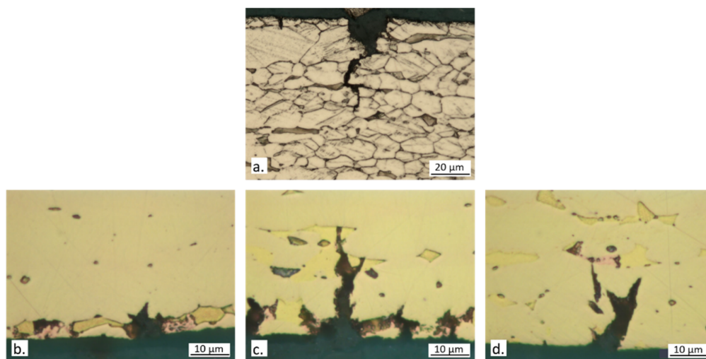
Figure 17. Optical micrographs of secondary cracks on CW602N section surfaces after SSRT in SDW solutions containing (a) 400 ppm (surface etching by acid \text{FeCl}_3 solution to evidence grain boundaries); (b) 100 ppm; (c) 400 ppm; and (d) 700 ppm chlorides.
