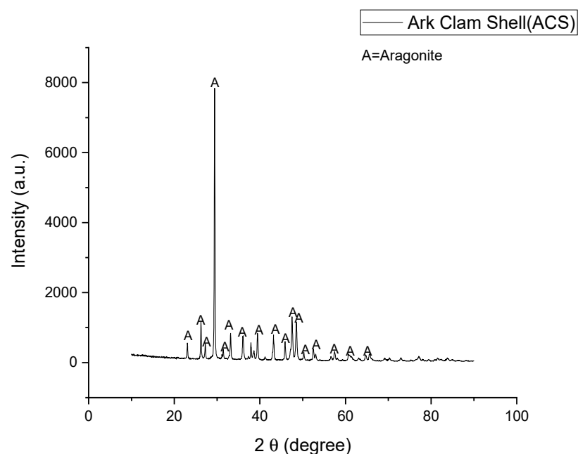
Figure 2. The XRD pattern of waste ACS powder at room temperature.
