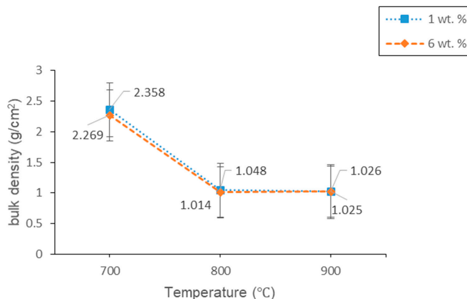
Figure 9. The bulk density of 1 and 6 wt% samples sintered at various temperatures for 60 min.
