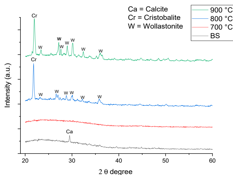
Figure 4. XRD pattern of foam glass-ceramics 1 wt% sintered at various temperatures for 60 min.
