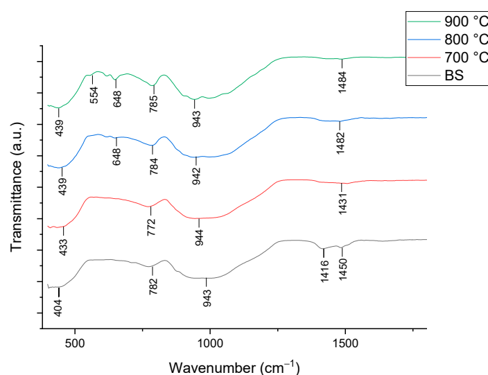
Figure 6. FTIR spectra of foam glass-ceramics 1 wt% sintered at various temperatures for 60 min.
