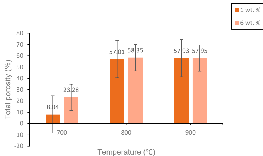
Figure 11. The total porosity of 1 and 6 wt% samples sintered at various temperatures for 60 min.
