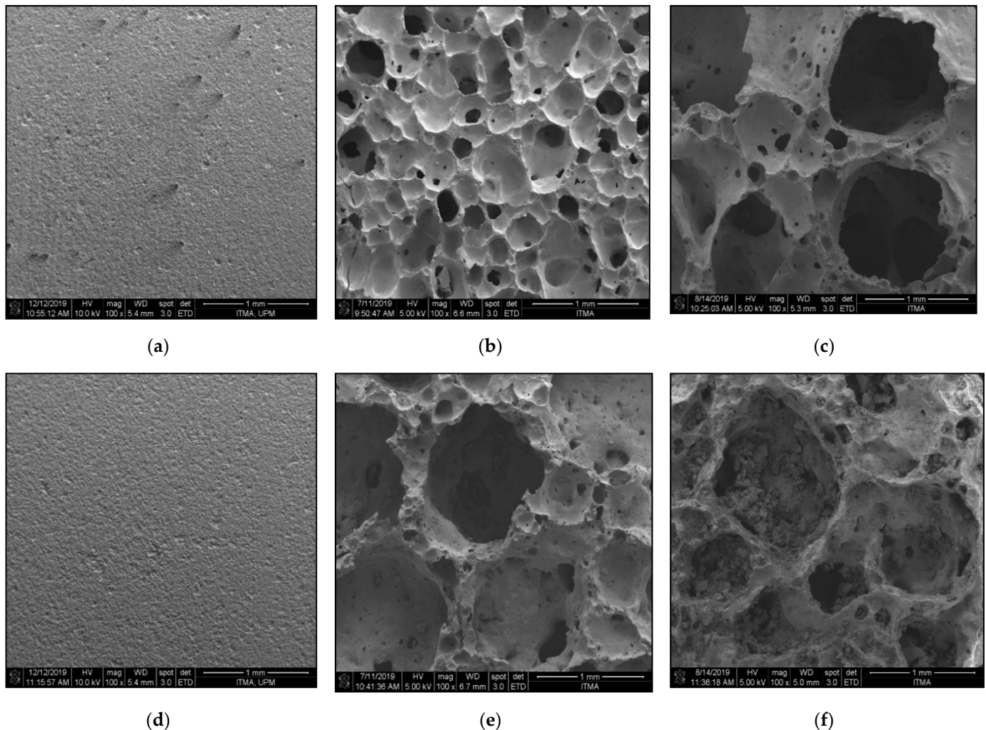
Figure 8. FESEM micrograph of foam glass-ceramics sintered for 60 min at various temperature (a) 1 wt% 700 °C, (b) 1 wt% 800 °C, (c) 1 wt% 900 °C, (d) 6 wt% 700 °C, (e) 6 wt% 800 °C, (f) 6 wt% 900 °C.
