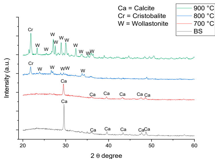
Figure 5. XRD pattern of foam glass-ceramics 6 wt% sintered at various temperatures for 60 min.
