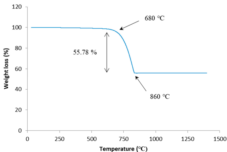
Figure 3. The TGA result of ACS weight loss against temperature.
