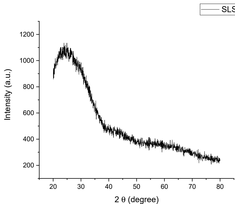
Figure 1. The XRD pattern of waste SLS glass powder at room temperature.
