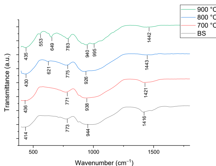
Figure 7. FTIR spectra of foam glass-ceramics 6 wt% sintered at various temperatures for 60 min.
