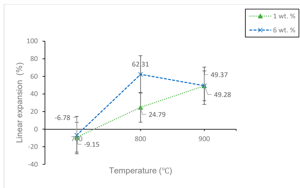
Figure 10. The linear shrinkage of 1 and 6 wt% samples sintered at various temperatures for 60 min.
