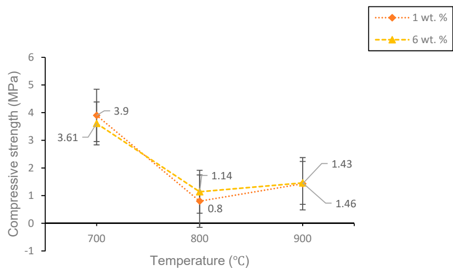
Figure 12. The compressive strength of 1 and 6 wt% samples sintered at various temperatures for 60 min.
