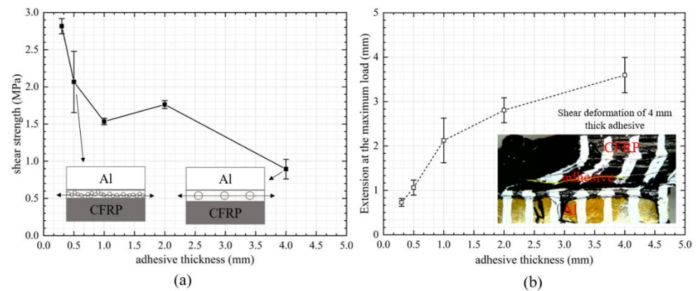
Figure 5. (a) Shear strength and (b) extension at the maximum load vs. thickness of the polyurethane adhesive. The inset pictures indicate the failure of the polyurethane joints. The figures in Figure 5a indicate the failure path in the sample, with the round circles representing the embedded glass bead. The figure in Figure 5b shows the shear deformation of the polyurethane joint with the 4 mm thick adhesive.
