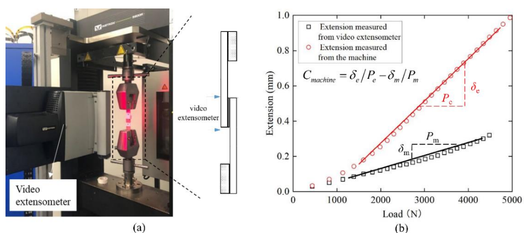
Figure 3. (a) Experimental setup with video extensometer; (b) extension vs. load relationship measured with video extensometer and machine, respectively. Units are in mm.
