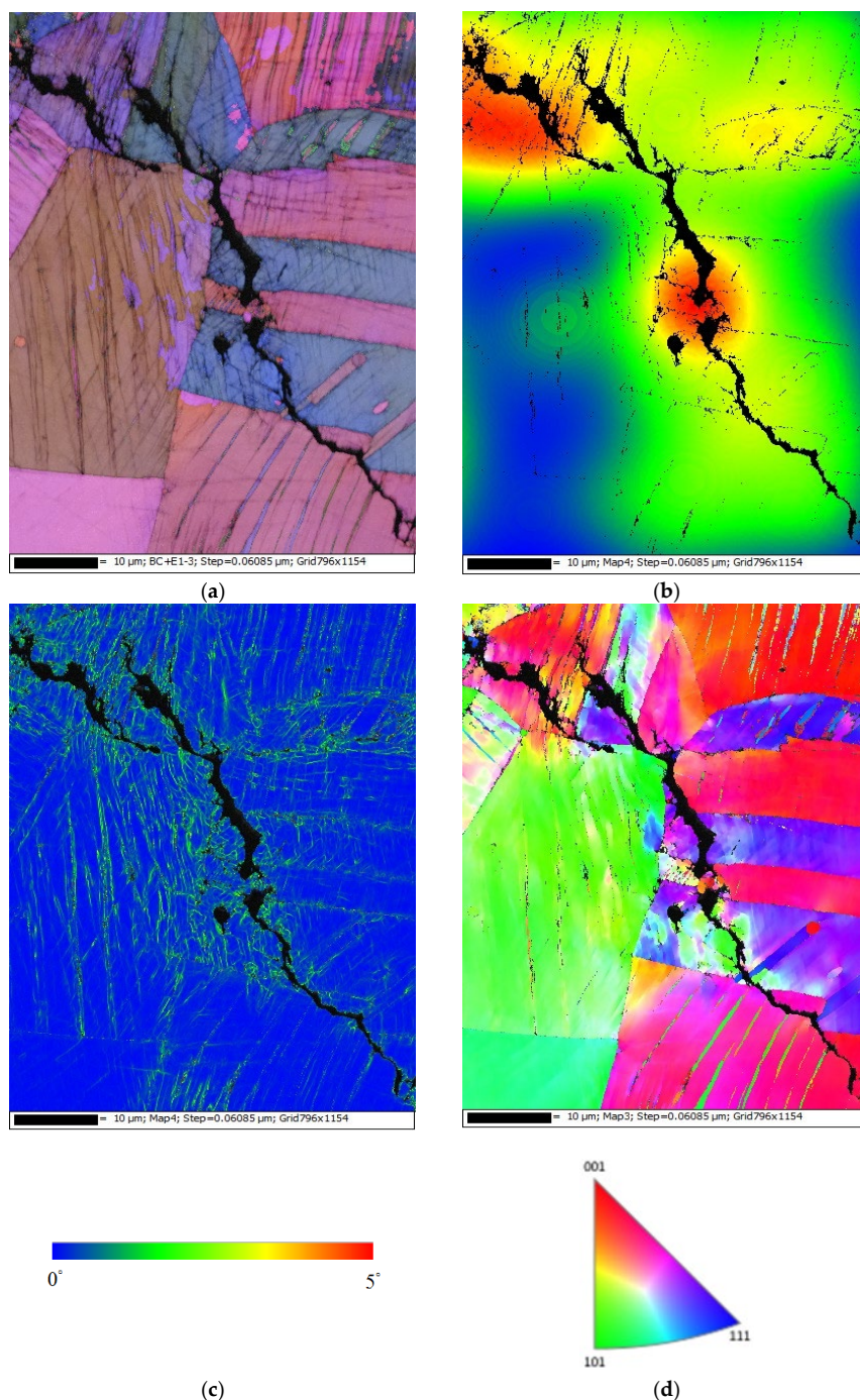
Figure 13. Electron back scatter diffraction (EBSD) maps for the crack region of the specimens deposited with a 1 g/m 2 chloride concentration tested for 7000 h at 70% RH: (a) Euler map, (b) strain counteracting map, (c) kernel average misorientation (KAM) map, and (d) inverse pole figure (IPF) map.
