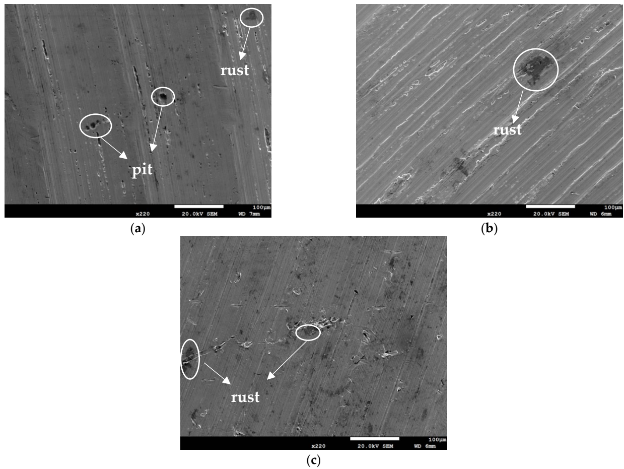
Figure 6. SEM micrographs of those specimens with a 0.1 g/m 2 chloride concentration at: (a) Relative humidity = 45%, (b) relative humidity = 55%, and (c) relative humidity = 70%.
