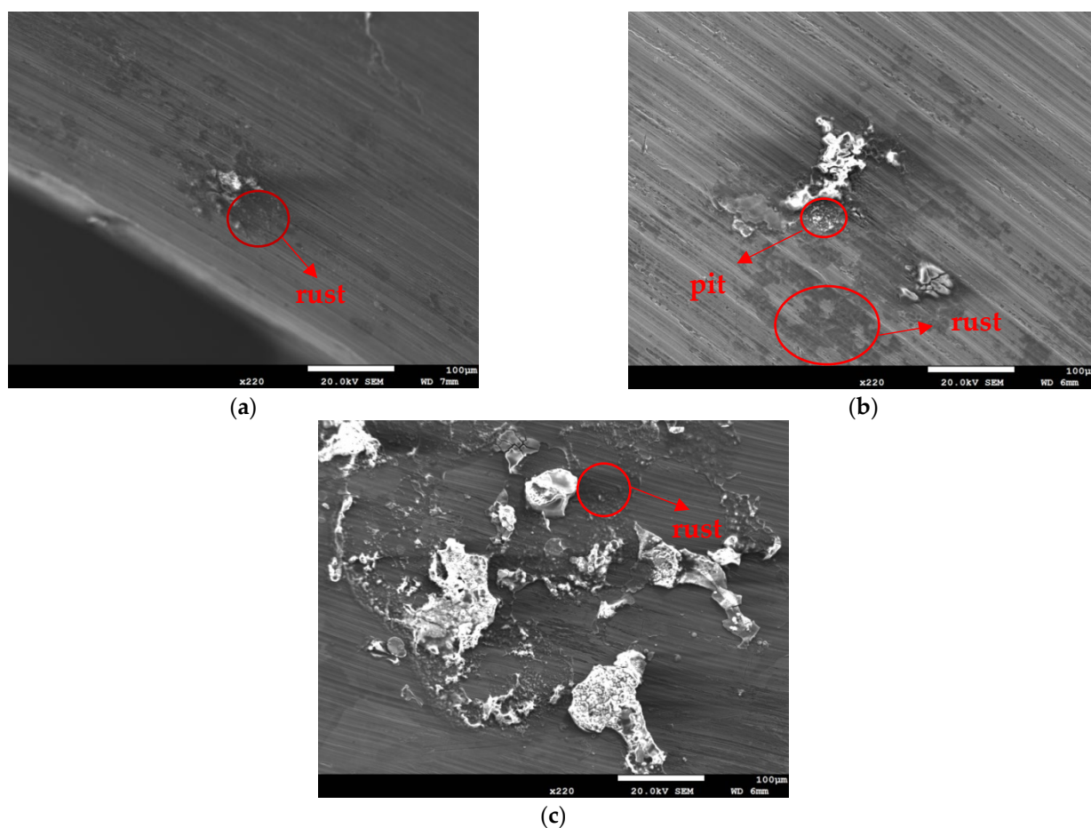
Figure 8. SEM micrographs of those samples with a chloride concentration of 1 g/m 2 after 7000 h of testing at: (a) RH = 45%, (b) RH = 55%, and (c) RH = 70%.
