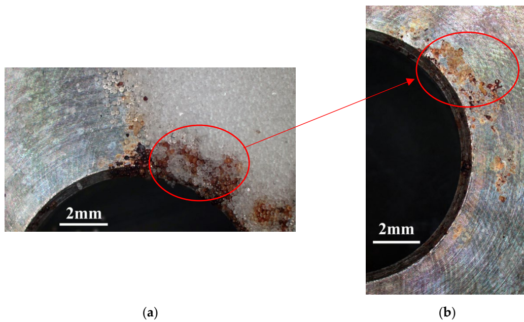
Figure 4. Macrographs of the corrosion regions of those samples with a chloride concentration of 1 g/m 2 at RH = 70%: (a) Specimen before cleaning and (b) specimen after cleaning.
