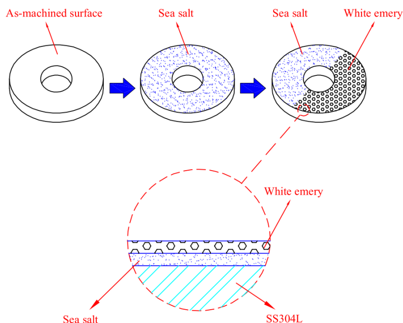
Figure 2. Schematic diagram of the specimen sprayed with synthetic sea water and white emery.
