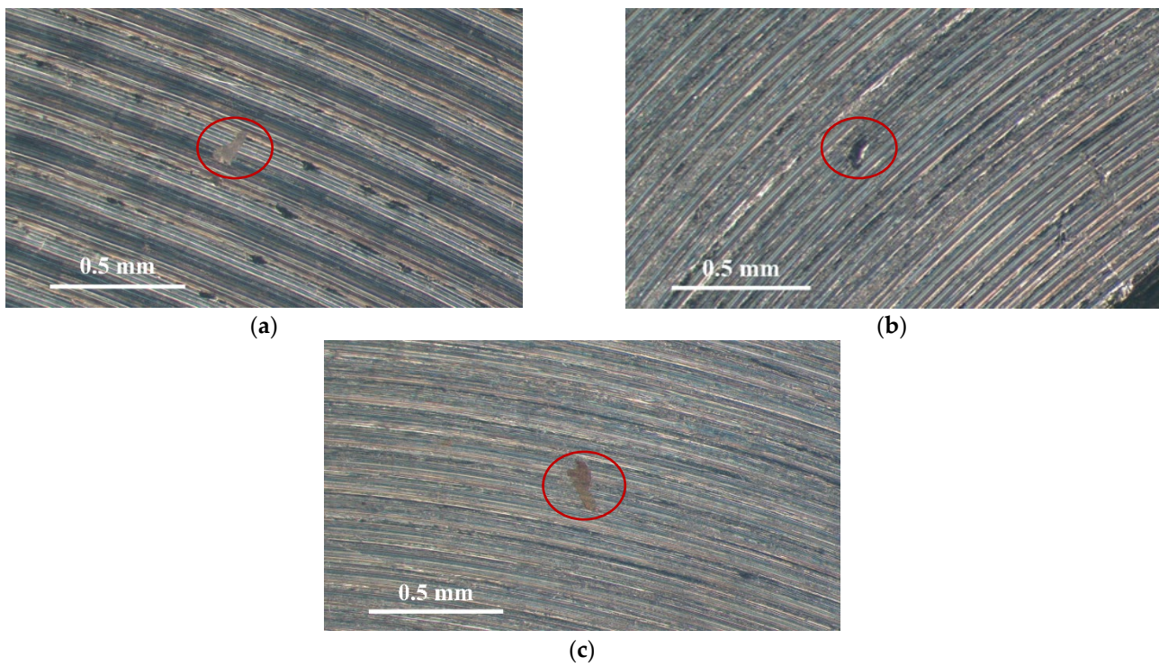
Figure 5. Macrographs of the corrosion regions of those samples with a 0.1 g/m 2 chloride concentration at: (a) Relative humidity = 45%, (b) relative humidity = 55%, and (c) relative humidity = 70%.
