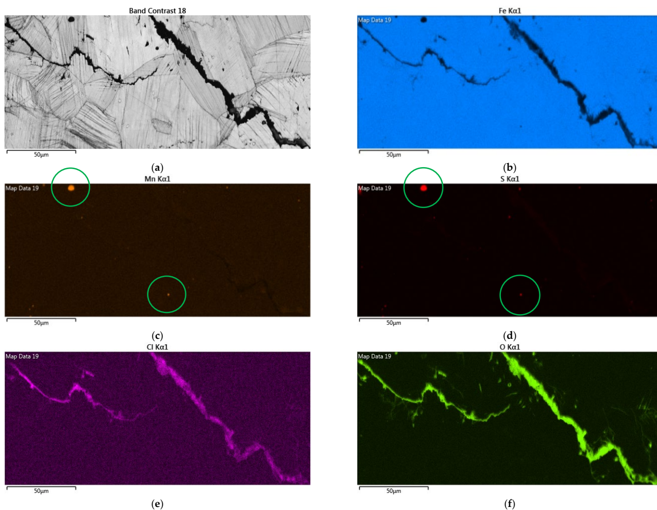
Figure 12. EDS mapping for the crack regions of those samples with a chloride concentration of 1 g/m 2 tested for 7000 h at a relative humidity of 70%: (a) Band contrast image, (b) Fe mapping, (c) Mn mapping, (d) S mapping, (e) Cl mapping, and (f) O mapping.
