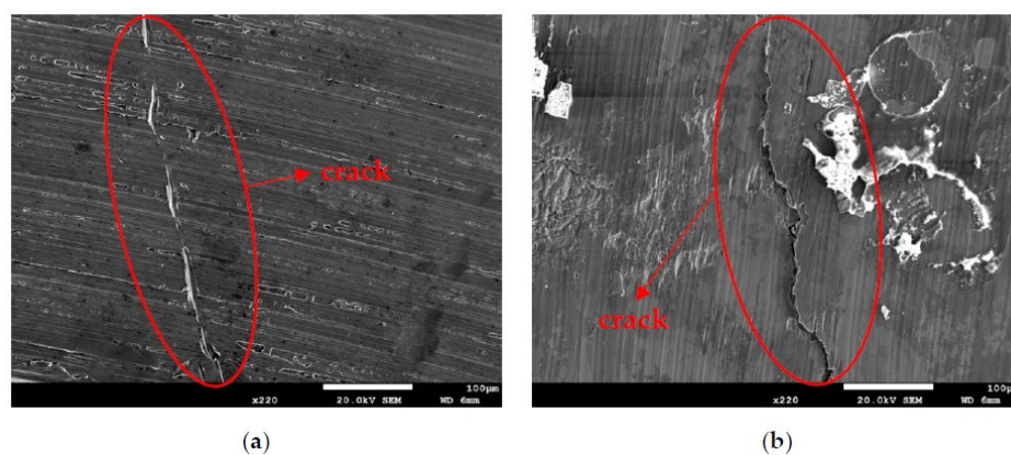
Figure 11. SEM morphology of the SCC in those samples with a chloride concentration of 1 g/m 2 after 7000 h of testing at: (a) RH = 55% and (b) RH = 70%.
