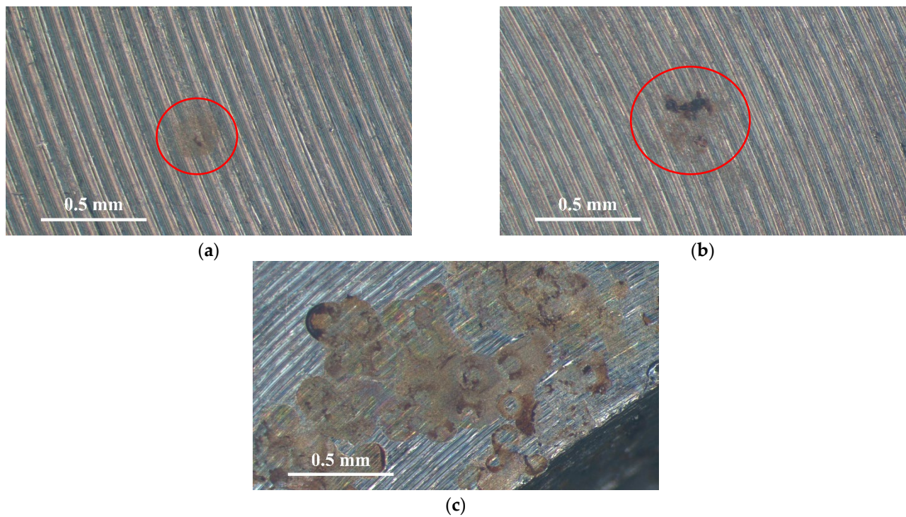
Figure 7. Macrographs of the corroded regions of those samples with a 1 g/m 2 chloride concentration at: (a) Relative humidity = 45%, (b) relative humidity = 55%, and (c) relative humidity = 70%.
