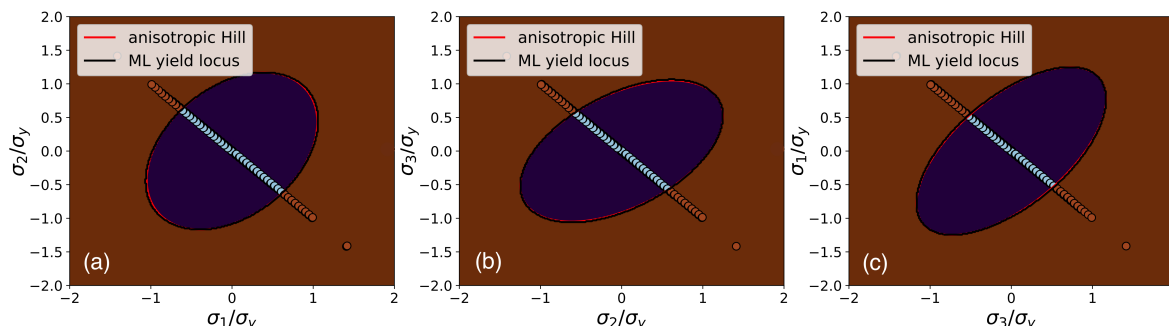
Figure 4. Color map of the trained SVC prediction of the yield function in slices through the principal stress space defined by plane-stress conditions: (a) \sigma_3 = 0 ; (b) \sigma_1 = 0 ; (c) \sigma_2 = 0 . Brown regions indicate values of “+1” (plasticity) and purple regions values of “-1” (elasticity). The ML yield locus, corresponding to the isoline for f_{SVC} = 0 , is represented as a black line; the yield locus of the Hill-like anisotropic reference material is indicated as a red line. The training data points are plotted with the same color code as in Figure 3.
