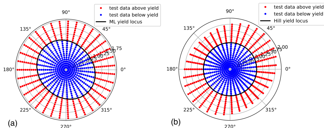
Figure 2. Polar plots of a subset of the training data produced from the anisotropic yield function of the reference material: (a) Von Mises (J2) equivalent stresses according to Equation (3) are used, such that the yield strength, rather than the equivalent stress, is a function of the polar angle \theta . (b) Equivalent stresses are calculated according to the Hill definition in Equation (5) to achieve a constant yield strength by mapping the equivalent stresses accordingly. In both figures, the yield locus is indicated by a solid black line, data points in the elastic regime are plotted in blue color and data in the plastic regime in red color. Both figures represent the same stress data, only mapped in a different way; all stresses are normalized with the reference yield strength \sigma_y .
