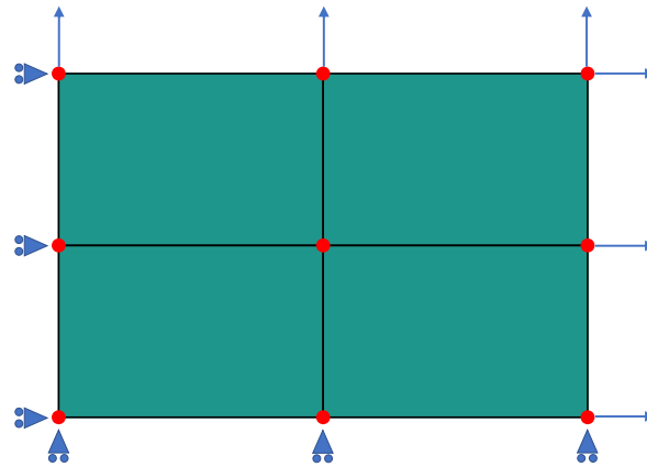
Figure 5. The finite element model on which four different load cases are studied consists of four quadrilateral elements (green) with linear shape function, and at total of nine nodes (red) situated at the corners of the elements. The bottom and left-hand-side boundary nodes are restricted to zero normal displacement (blue triangles), and the loading is applied on top and right-hand-side-nodes (blue arrows), as described in the text.
