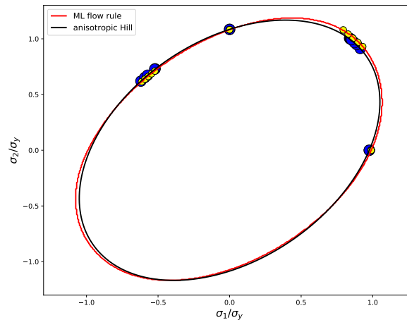
Figure 7. Stress states obtained for the four different plane-stress load cases are plotted in the \sigma_1 - \sigma_2 plane together with the yield loci of the trained ML flow rule and the Hill-like reference material. The flow stresses resulting from the ML yield function are plotted as small yellow circles and those from anisotropic Hill plasticity as large blue circles.
