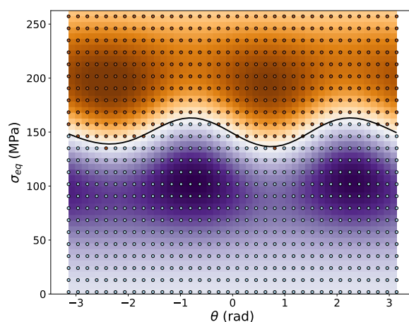
Figure 3. Field plot of the trained SVM decision function defined in Equation (18), where areas in purple color shades represent negative values and brown shades represent positive values. The numerical value of the decision function is not relevant because only its sign is taken into account in the flow rule. The isoline for f_{SVC} = 0 is represented as a black line. Training data are plotted in light blue color for data with negative values (elastic) and in brown color for positive values (plastic).
