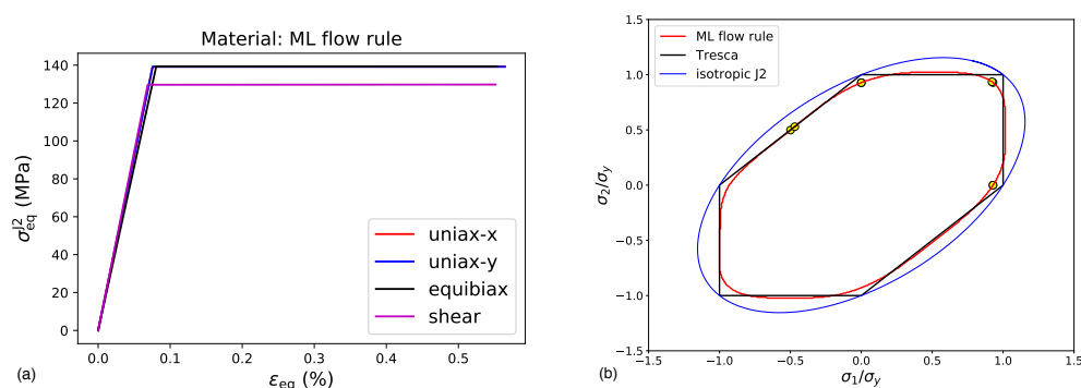
Figure 9. Results of FEA on the material with an ML flow rule trained with data obtained from a Tresca yield criterion: (a) Equivalent J2 stress plotted over the equivalent total strain, for the four different load cases given in Table 2. (b) Flow stresses obtained with the ML yield function plotted as yellow circles in the \sigma_1 - \sigma_2 principle stress space, together with the yield loci of the ML flow rule, the Tresca flow rule and an isotropic J2 flow rule.
