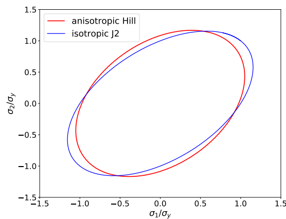
Figure 1. Yield locus for plane-stress conditions ( \sigma_3 = 0 ) and Hill-like anisotropy with parameters given in Table 1 (red line) and for an isotropic material with the same yield strength, but H_1 = H_2 = H_3 = 1 (blue line). The values of the principal stresses are normalized by the yield strength \sigma_y .
