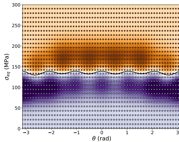
Figure 8. Field plot of the ML yield function trained with data generated from a reference material with a Tresca yield criterion, where areas in purple color shades represent negative values and brown shades represent positive values. The isoline, where the ML yield function is zero, is plotted as black line. The test data points are plotted as brown circles, for stresses in the plastic regime, and as light blue circles for stresses in the elastic regime.
