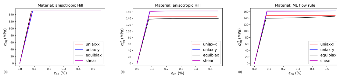
Figure 6. Stress strain curves obtained for elastic-ideal plastic material behavior under the loading conditions specified in the legend: (a) Equivalent total strain vs. equivalent Hill-stress, (b) equivalent total strain vs. equivalent J2-stress for Hill-like yield function, and (c) equivalent total strain vs. equivalent J2-stress for ML yield function.
