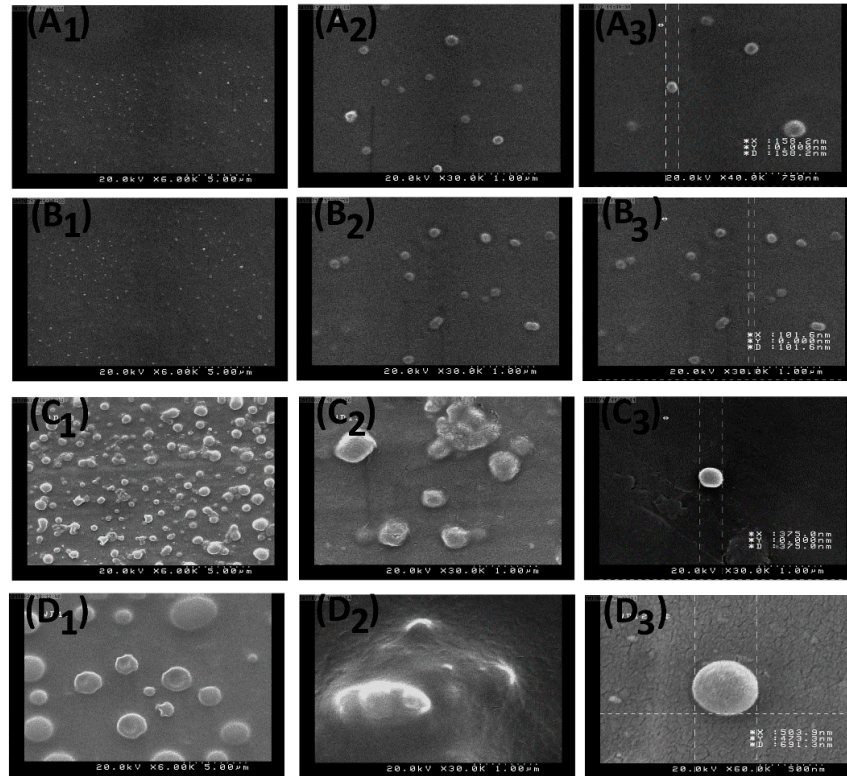
Figure 3. FE-SEM images of the nanoparticles (NPs) with different concentration ratios: (A 1 ) 0.1% of PLGA at 6000×, (A 2 ) 0.1% of PLGA at 30,000×, (A 3 ) a size representation of 0.1% of PLGA NP at 40,000×, (B 1 ) 0.2% of PLGA at 6000×, (B 2 ) 0.2% of PLGA at 30,000×, (B 3 ) a size representation of 0.2% of PLGA NP at 30,000×, (C 1 ) 0.3% of PLGA at 6000×, (C 2 ) 0.3% of PLGA at 30,000 X, (C 3 ) a size representation of 0.3% of PLGA NP at 30,000×, (D 1 ) 0.5% of PLGA at 6000×, (D 2 ) 0.5% of PLGA at 30,000× and (D 3 ) a size representation of 0.5% of PLGA NP at 60,000×.
