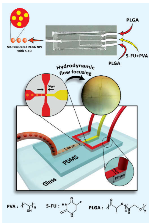
Figure 1. Schematic of microfluidic (MF) device setup.
