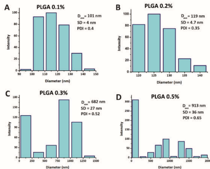
Figure 4. NPs size and their size distribution curves based on dynamic light scattering (DLS) at different PLGA concentrations: (A) 0.1 (% w/v), (B) 0.2 (% w/v), (C) 0.3 (% w/v) and (D) 0.5 (% w/v). (The p-value for all data was less than 0.05).
