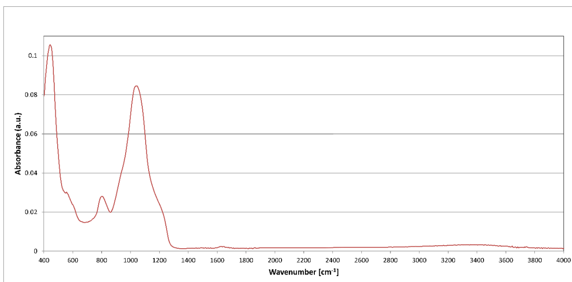
Figure S1. FTIR spectrum of ordered 5 wt% Cu-MSG.
