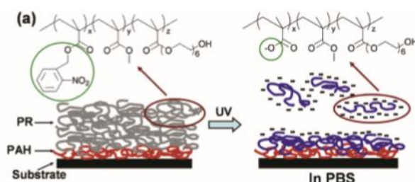
Figure 3. Chemical structure of Photoresist (PR) (a) spin-coated on Poly(allylamine) hydrochloride (PAH) and its mechanism for in situ polyelectrolyte bilayer formation (Reprinted with the permission from reference [79] Copyright 2004 American Chemical Society).
