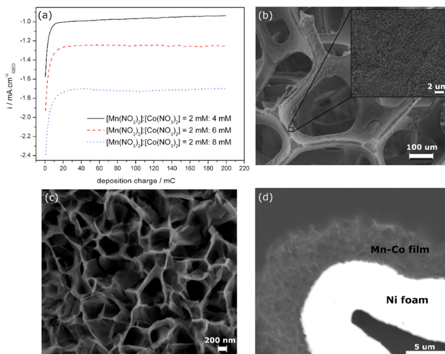
Figure 1. (a) Synthesis graphs recorded during the electrochemical synthesis of Mn/Co oxide/hydroxides at -1.1 \text{ V} vs. \text{Ag}/\text{AgCl} in an aqueous solution of differently concentrated \text{Mn}(\text{NO}_3)_2 \cdot 4\text{H}_2\text{O} and \text{Co}(\text{NO}_3)_2 \cdot 6\text{H}_2\text{O} with the deposition time limited by a charge of 200 mC; (b–d) SEM images of Mn-Co film deposited on nickel foam in a solution of Mn/Co (2 mM/8 mM) for 200 mC with different magnifications (b,c—surfaces, d—polished cross-section).
