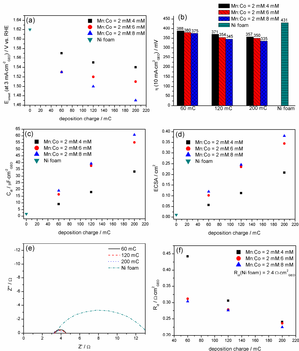
Figure 6. Evolution of the (a) onset potential, (b) overpotential determined at 10 \text{ mA} \cdot \text{cm}^{-2} , (c) double-layer capacitance, (d) electroactive surface area (ECSA), (e) electrochemical impedance spectra (EIS) measured at 0.7 \text{ V} vs. Ag/AgCl, and (f) R_{\text{ct}} of the oxygen evolution reaction (OER) as a function of the deposition charge for the Mn-Co film synthesised under different conditions on nickel foam.
