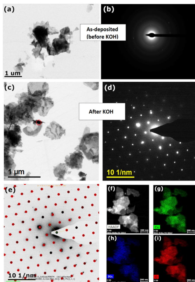
Figure 3. (a) Bright Field (BF) TEM image, and (b) corresponding experimental Selected Area Diffraction (SAED) pattern of Mn-Co film before alkaline treatment; (c) BF-TEM image, area of SAED
