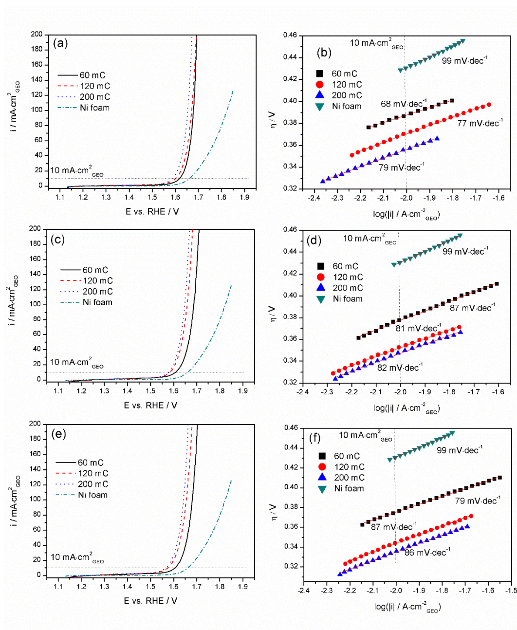
Figure 5. Linear sweep voltammetry profiles and corresponding Tafel plots for Mn-Co film synthesised in the presence of (a,b) Mn/Co 2 mM/4 mM, (c,d) 2 mM/6 mM, and (e,f) 2 mM/8 mM on nickel foam measured in Ar-purged 1 M KOH.
