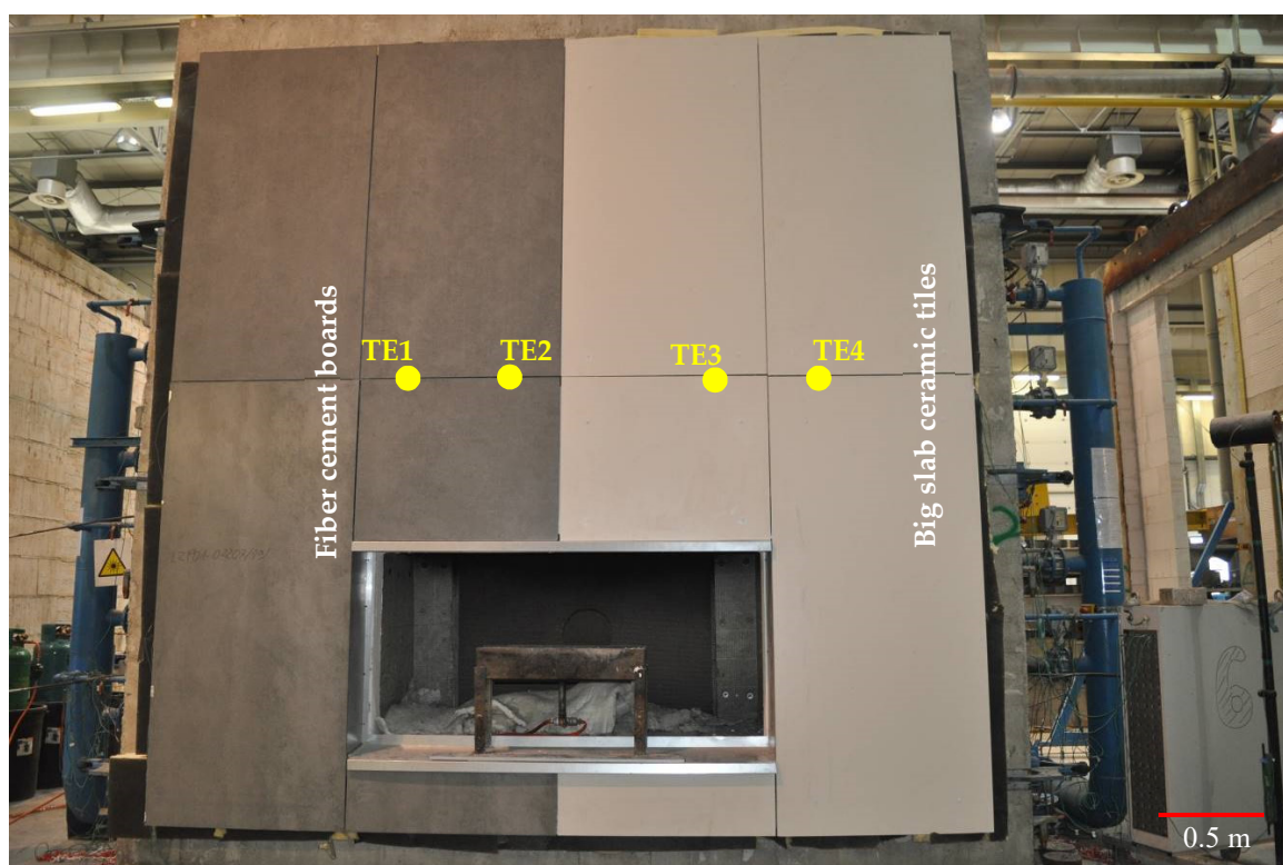
Figure 3. Ventilated facade model with location of thermocouples.
