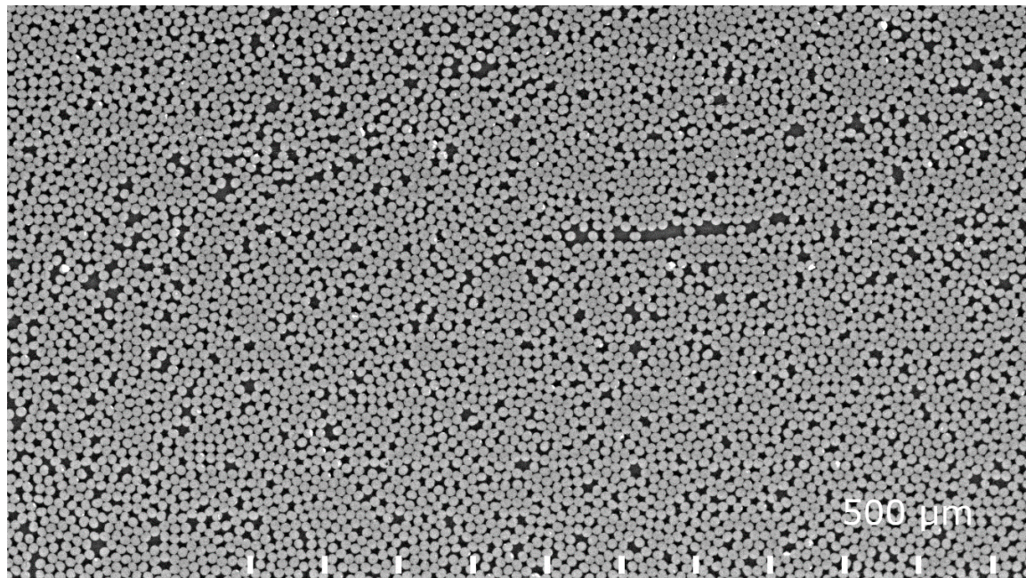
Figure 5. Electron backscatter image distinguishes between fiber and matrix due to a difference in average atomic number (Z contrast).
