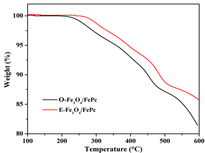
Figure S3. TGA curves of the Fe 3 O 4 /FePc hybrid microspheres before and after etching.
