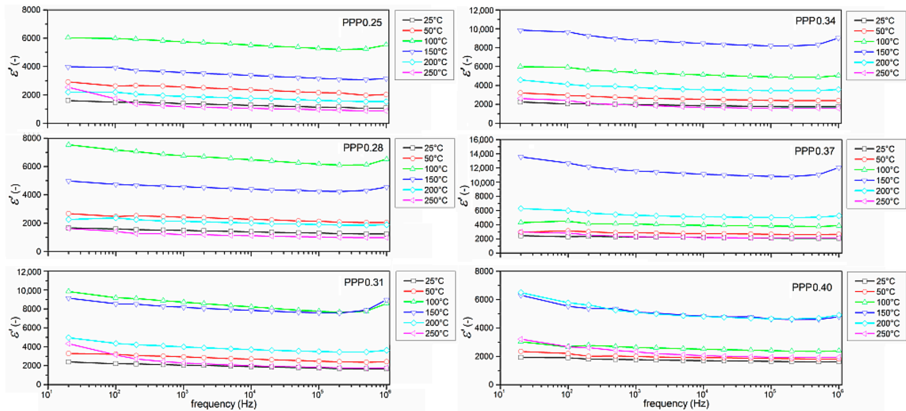
Figure 6. Frequency dependence of the real part of dielectric permittivity for PMN-PT-PS ceramics with various x at different temperatures.
