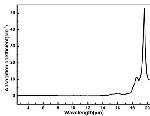
Figure S2. Calculated absorption coefficient of GaSe crystals
