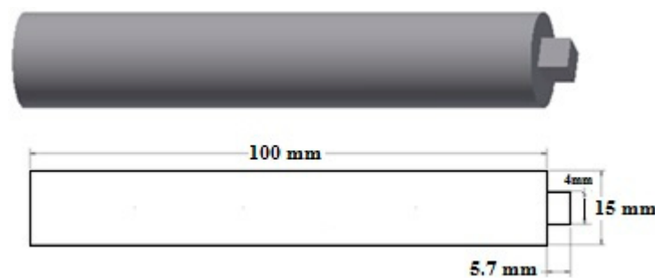
Figure 1. Geometry of the tool design.
