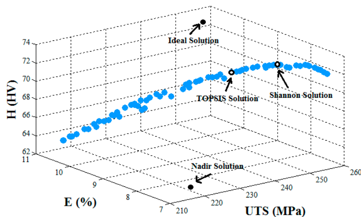
Figure 4. Pareto frontier for the triple objective ( UTS-E-H ).
