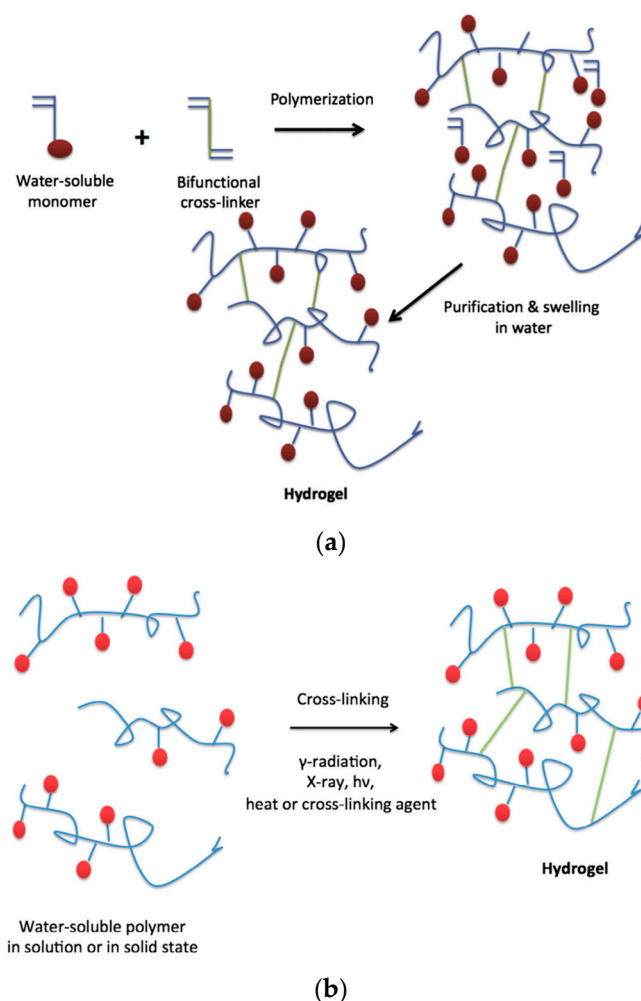
Figure 3. (a) Synthesis of hydrogels by polymerization of monomers and crosslinking agent. (b) Synthesis of hydrogels by cross-linking of pre-polymerized water-soluble polymers. Reproduced with permission from [16].
