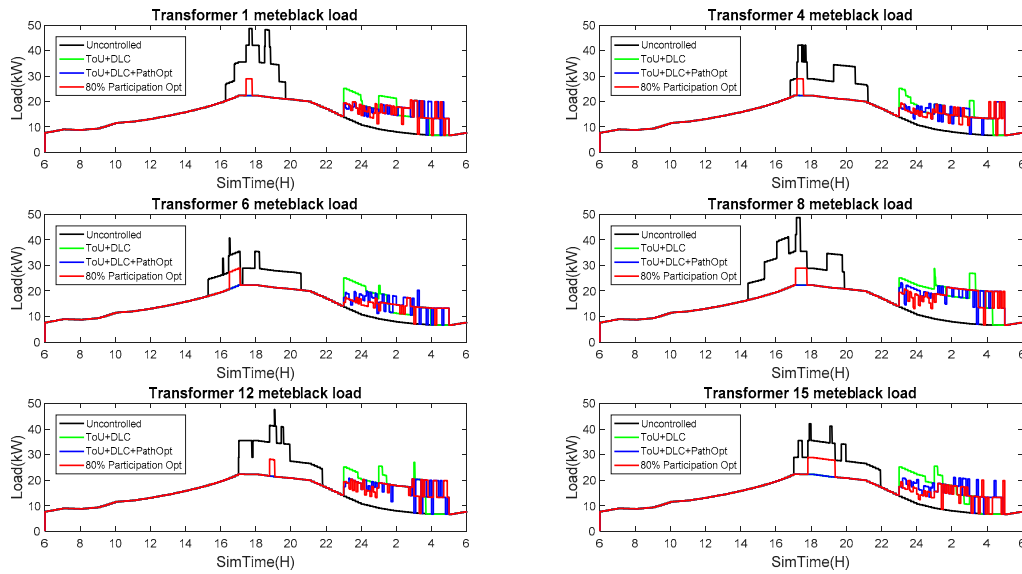
Figure 8. Transformer-level load profile for transformers in phase C with uncontrolled PEV charging, ToU + DLC charging, ToU + DLC + optimal control charging, and 80% participation rate of ToU + DLC + optimal control charging.
