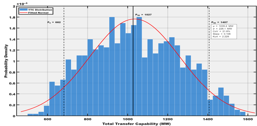
Figure 6. Empirical TTC distribution for the IEEE 39-bus Area 1 → Area 2 corridor under peak load conditions ( N = 1000 LHS scenarios). The histogram shows the scenario-based TTC density; the red curve is a fitted normal distribution. Vertical lines indicate P_5 , P_{50} , and P_{95} , highlighting the non-Gaussian, mixed-regime TTC behavior under simultaneous thermal and voltage constraints.
