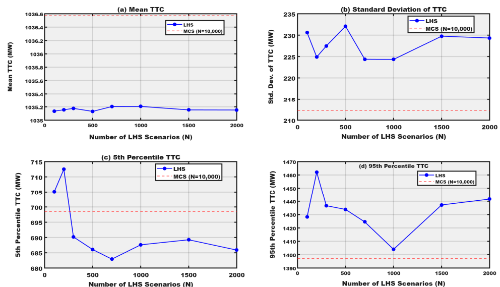
Figure 5. LHS convergence of TTC statistics for the IEEE 39-bus Area 1 \rightarrow Area 2 transfer corridor under stressed loading (peak demand \approx 6097 MW): (a) mean TTC, (b) standard deviation, (c) 5th percentile TTC, and (d) 95th percentile TTC versus number of LHS scenarios. Red dashed lines indicate the MCS reference values ( N = 10,000 ).
