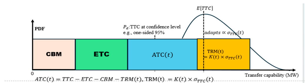
Figure 2. Probabilistic ATC formulation with dynamic TRM.
