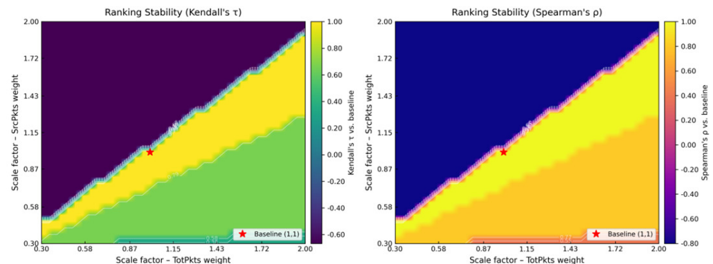
Figure 4. Sensitivity heat map of PROMETHEE ranking stability under AHP weight perturbations. Due to high ranking stability, correlation values are concentrated within a narrow range, resulting in limited color variation.
