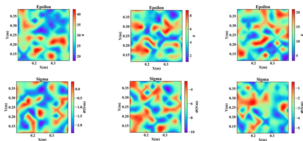
Figure 22. 2D inversion results in the starting stage of the water flooding oil experiment done in a laboratory rock core. The first row shows the variations in the electric permittivity distribution in different slices of the core, and the second row shows the variations in the conductivity distribution in different slices of the core.
