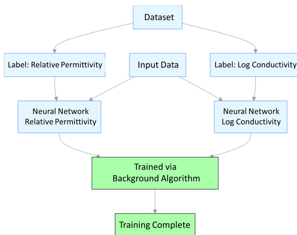
Figure 7. Inversion neural network training flowchart.
