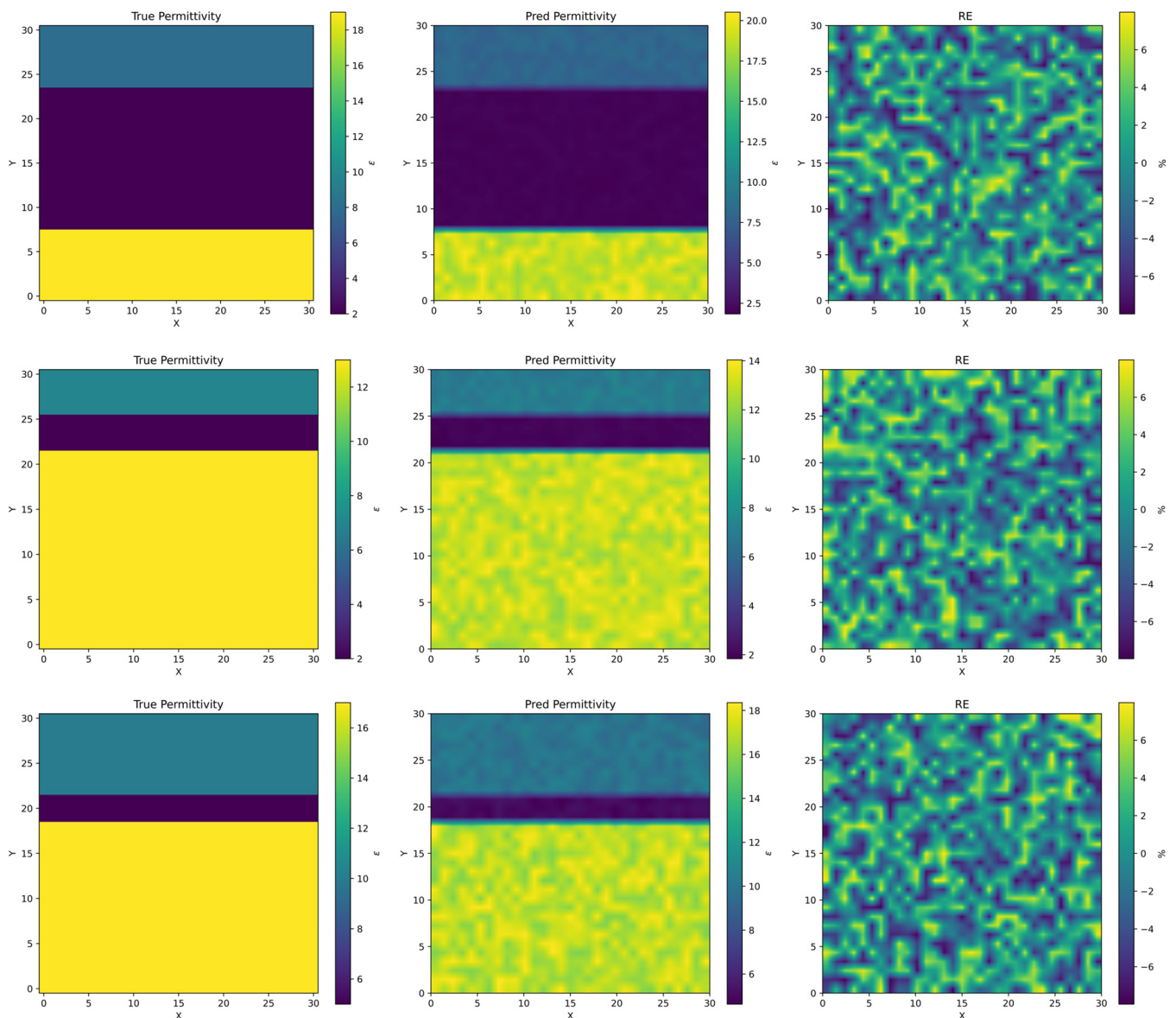
Figure 10. 2D dielectric constant inversion results of three randomly selected synthetic models, where the first, second, and third layer is from three models, and the first, second, and third column is the true dielectric constant, inversion results, and the relative errors, respectively.
