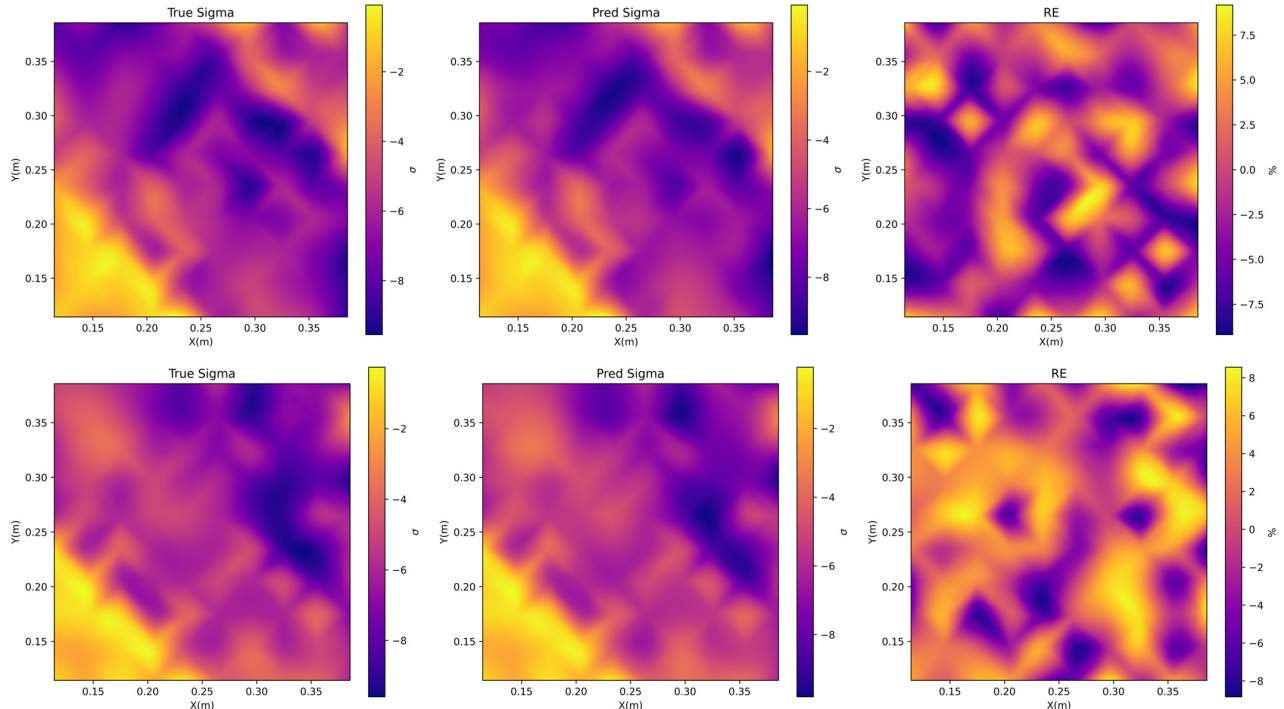
Figure 19. 2D inversion results for another random model. Each row of three images represents the inversion results for different models. The left image shows the true distribution, the middle image shows the inverted distribution, and the right image shows the relative error distribution of the inversion results. The first row is about the distributions of permittivity, and the second row is about the conductivity distributions.
