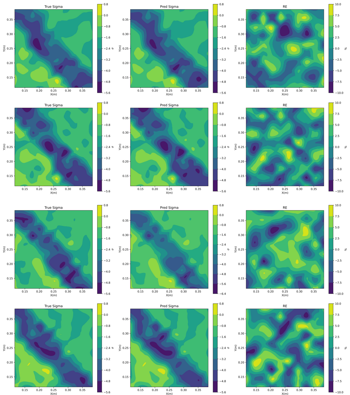
Figure 14. 2D conductivity inversion results for the model. Each row of three images represents the inversion results for different models. The left column image shows the true conductivity distribution, the middle column image shows the inverted conductivity distribution, and the right column image shows the relative error distribution of the inversion results.
