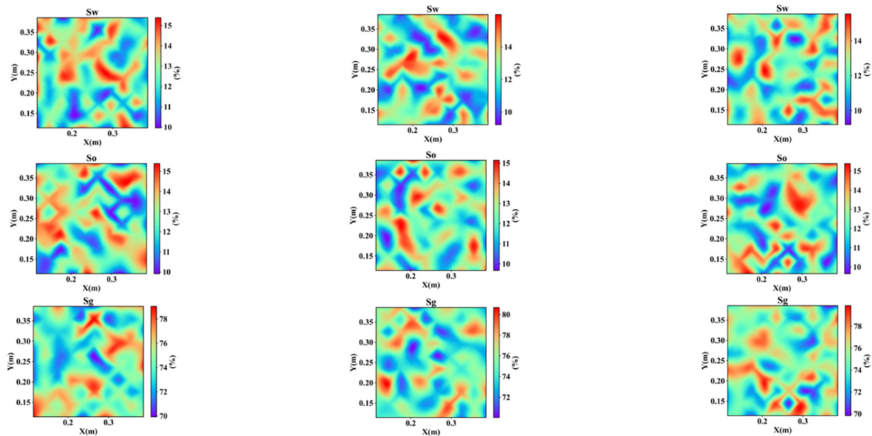
Figure 27. 2D saturation results in the end stage of the gas flooding water experiment done in a laboratory rock core. The first row shows the water saturation distribution in different slices of the core, the second row shows the oil saturation distribution in different slices of the core, and the third row shows the gas saturation distribution in different slices of the core.
