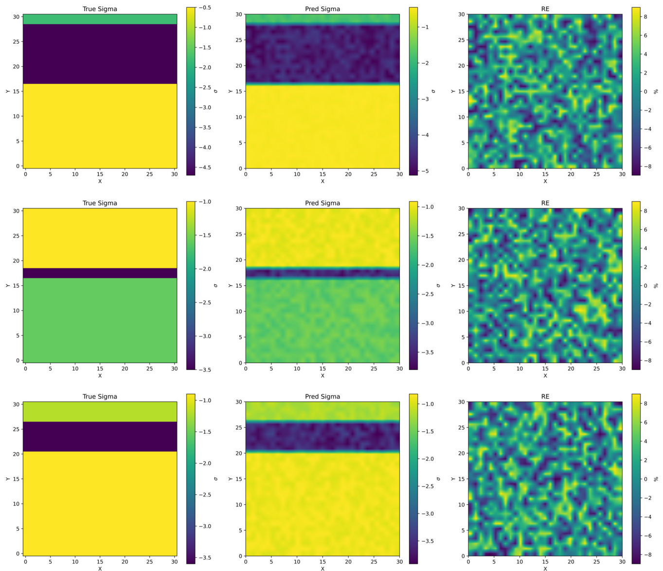
Figure 11. 2D conductivity inversion results for the model of three randomly selected synthetic models, where the first, second, and third layer are from three models, and the first, second, and third column is the true conductivity, inversion results, and the relative errors, respectively.
