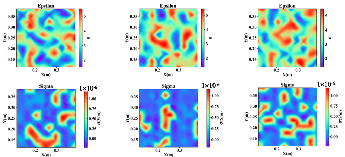
Figure 26. 2D inversion results at the end of the air flooding water experiment done in a laboratory rock core. The first row shows the variations in the electric permittivity distribution in different slices of the core, and the second row shows the variations in the conductivity distribution in different slices of the core.
