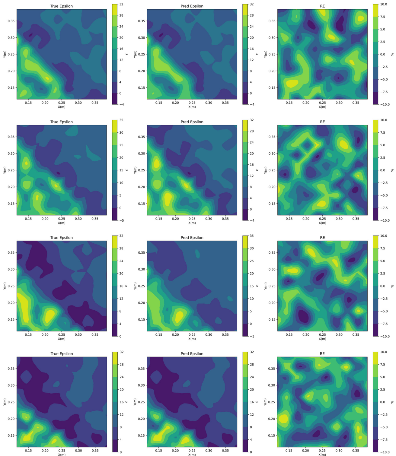
Figure 13. 2D dielectric constant inversion results for the model. Each row of three images represents the inversion results for different models. The left column image shows the true dielectric constant distribution, the middle column image shows the inverted dielectric constant distribution, and the right column image shows the relative error distribution of the inversion results.
