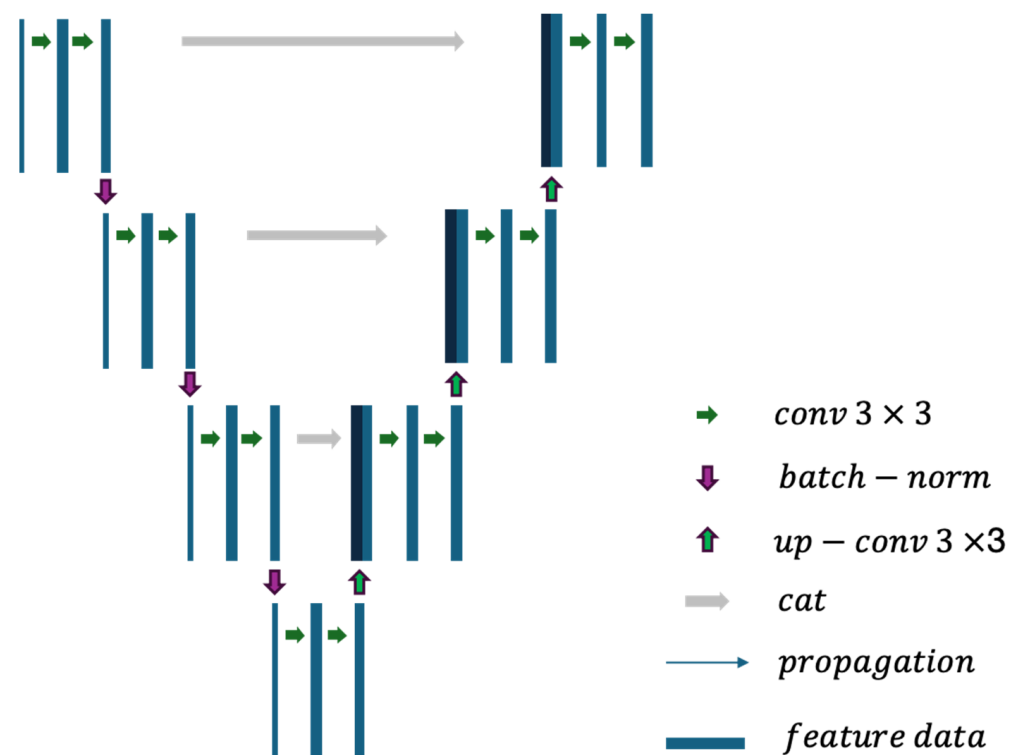
Figure 6. Schematic diagram of the U-Net neural network structure.
