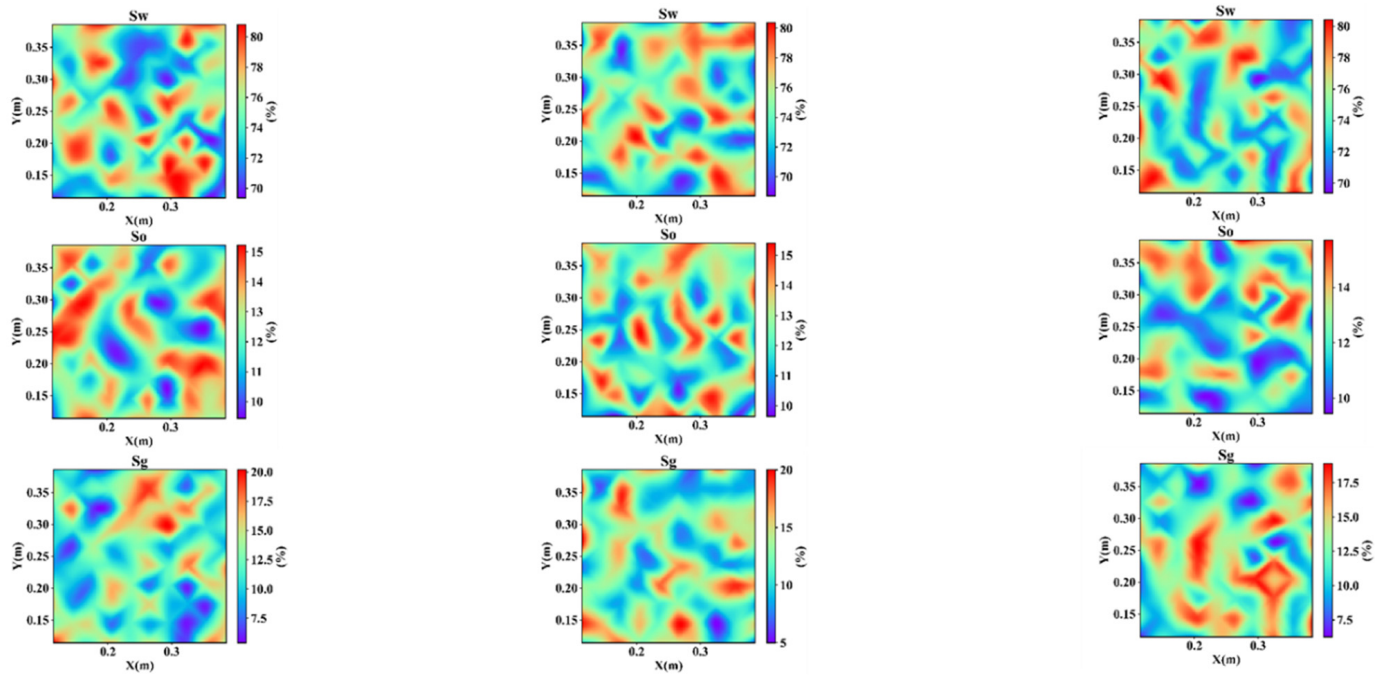
Figure 25. 2D saturation results in the starting stage of the air flooding water experiment done in a laboratory rock core. The first row shows the water saturation distribution in different slices of the core, the second row shows the oil saturation distribution in different slices of the core, and the third row shows the gas saturation distribution in different slices of the core.
