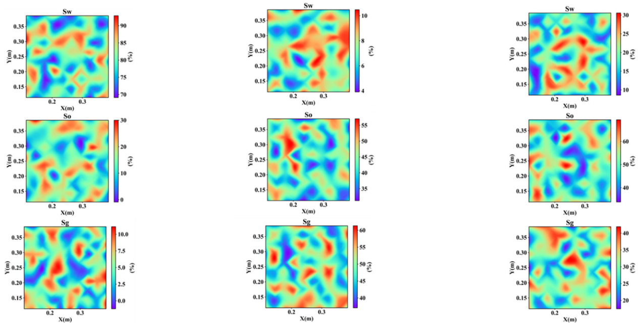
Figure 23. 2D saturation results in the starting stage of the water flooding oil experiment done in a laboratory rock core. The first row shows the water saturation distribution in different slices of the core, the second row shows the oil saturation distribution in different slices of the core, and the third row shows the gas saturation distribution in different slices of the core.
