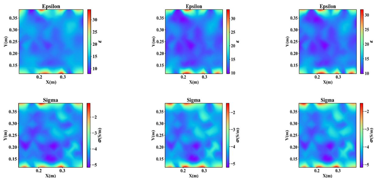
Figure 24. 2D inversion results at the beginning of the air flooding water experiment done in a laboratory rock core. The first row shows the variations in the electric permittivity distribution in different slices of the core, and the second row shows the variations in the conductivity distribution in different slices of the core.
