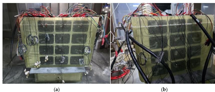
Figure 21. The observation system of the physical core flooding experiment. (a) 12 transmitters distributed on one side of the core, (b) 12 receivers distributed on another side of the core.
