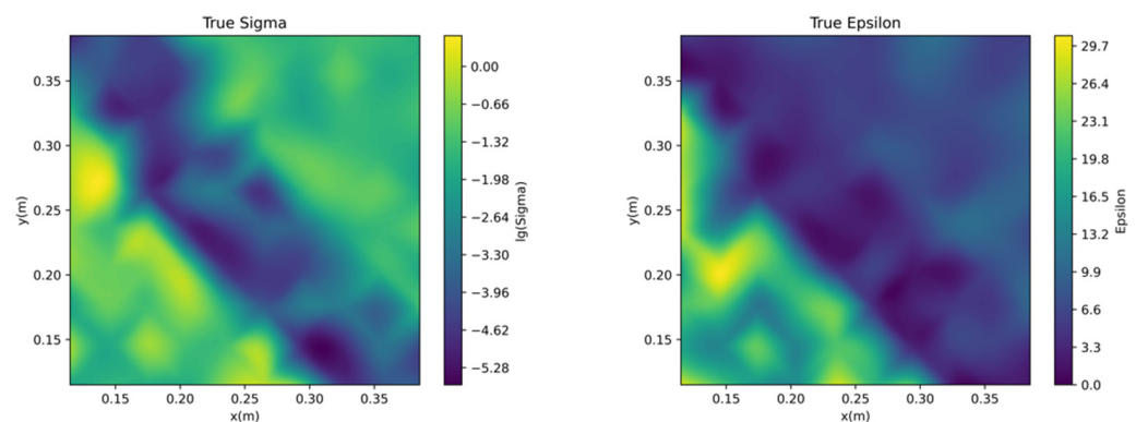
Figure 5. The conductivity and dielectric constant distribution map, where the (left panel) is about the logarithmic conductivity distribution and the (right panel) shows the dielectric constant distribution.
