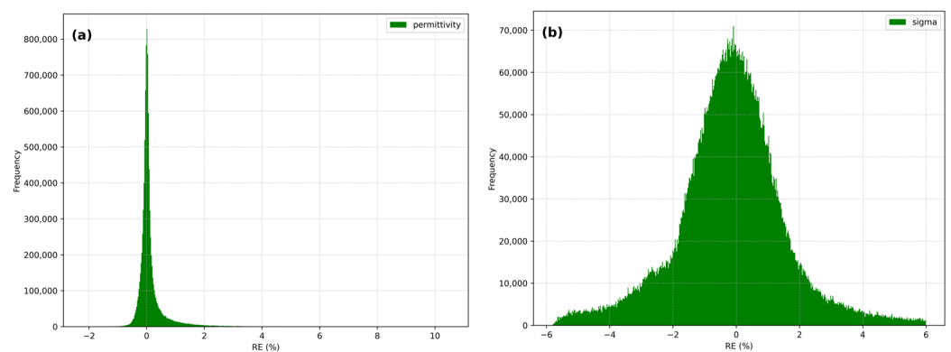
Figure 12. Relative error distribution of the test set: (a) permittivity; (b) conductivity.
