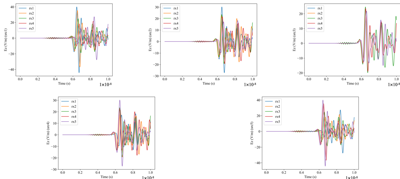
Figure 2. Forward simulation results from the gprMax software, where src1, src2, src3, src4, and src5 represent the first to the fifth transmitter antennas, and rx1, rx2, rx3, rx4, and rx5 represent the first to the fifth receiver antennas.
