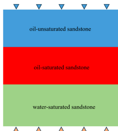
Figure 3. Distribution of different media states at different stages of flooding. The blue triangle represents the transmitter and the orange triangle indicates the receivers.
