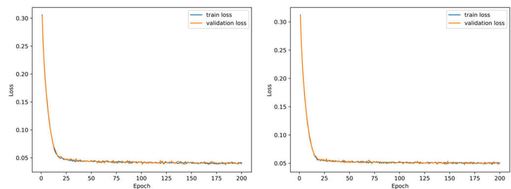
Figure 9. Loss function decay curves for Dataset 2. The ( left graph ) shows the decay curve for the dielectric constant inversion network, and the ( right graph ) shows the decay curve for the resistivity inversion network.
