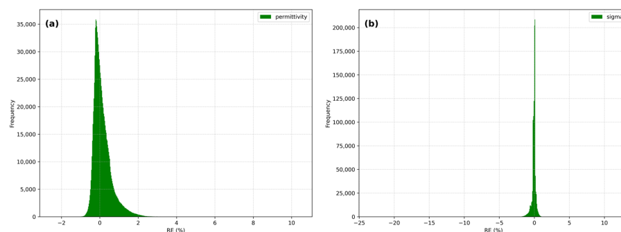
Figure 20. Relative error distribution of the test set: (a) permittivity; (b) conductivity.
