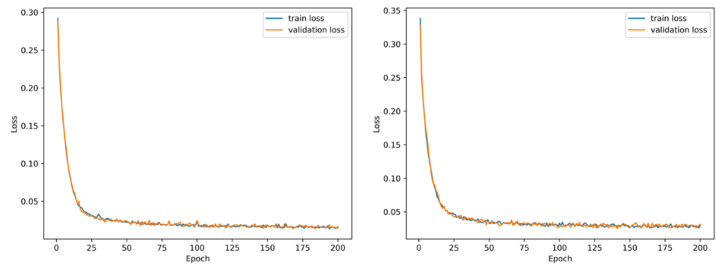
Figure 8. Loss function decay curves for Dataset 1. The ( left graph ) shows the decay curve for the dielectric constant inversion network, and the ( right graph ) shows the decay curve for the resistivity inversion network.
