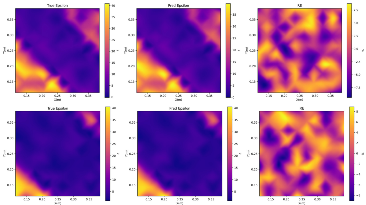
Figure 18. 2D inversion results for a random model. Each row of three images represents the inversion results for different models. The left image shows the true distribution, the middle image shows the inverted distribution, and the right image shows the relative error distribution of the inversion results. The first row is about the distributions of permittivity, and the second row is about the conductivity distributions.
