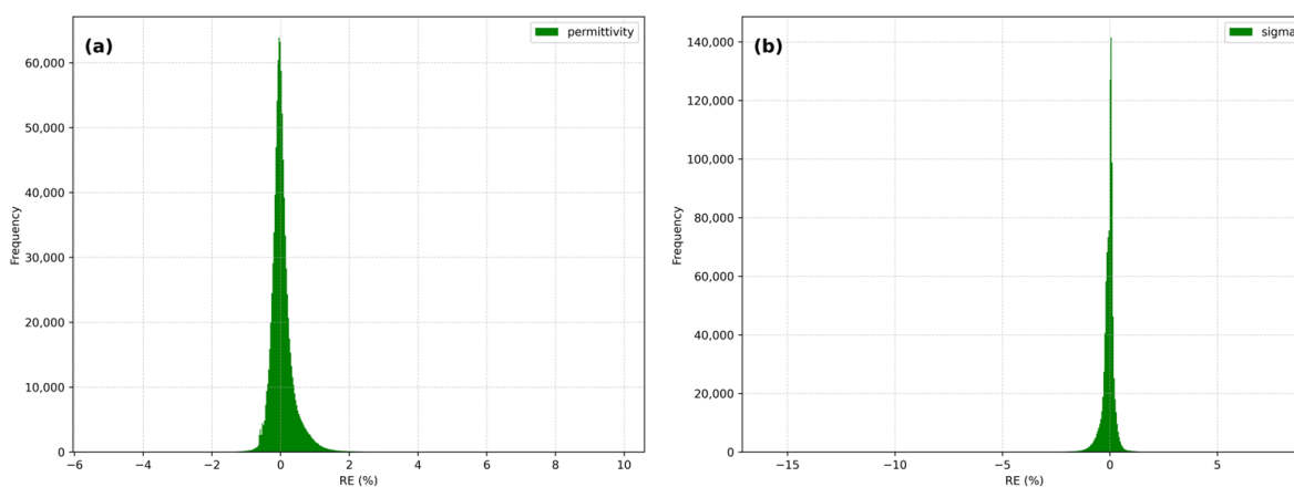
Figure 16. Relative error distribution of the test set: (a) permittivity; (b) conductivity.
