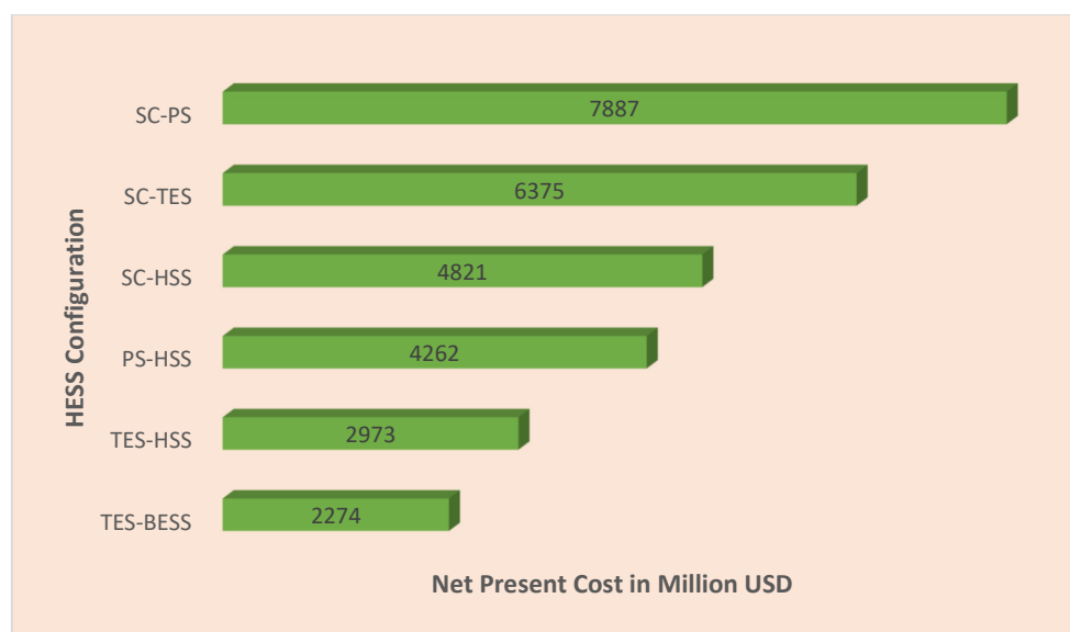
Figure 13. Comparative net present cost (NPC) of HESS configurations [156].
