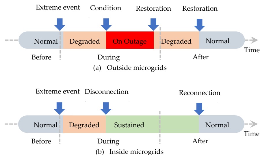
Figure 6. Operating conditions of MG during critical events: (a) outside MG (b) inside MG [53].
