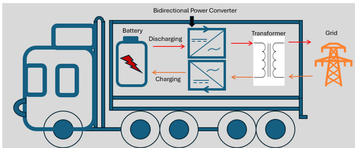
Figure 10. A typical vehicle-mounted MESS [114].
