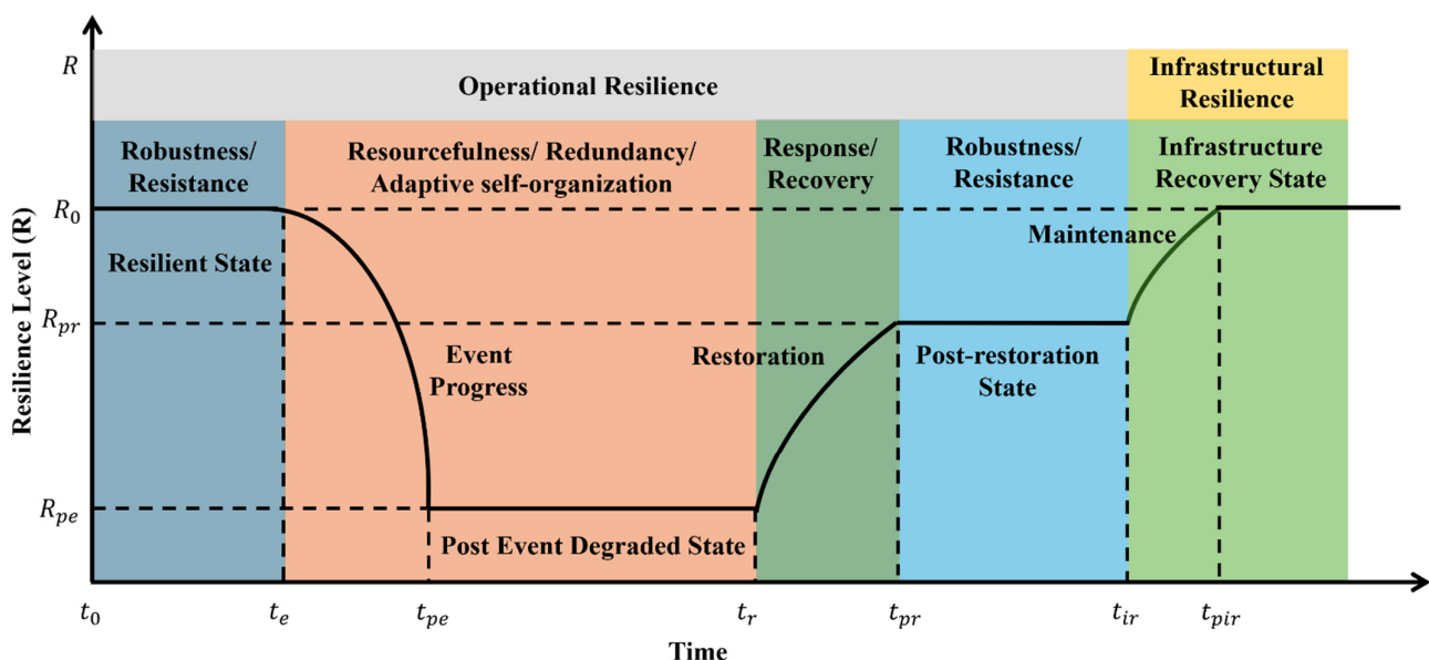
Figure 3. Resilience vs. time curve [38].
