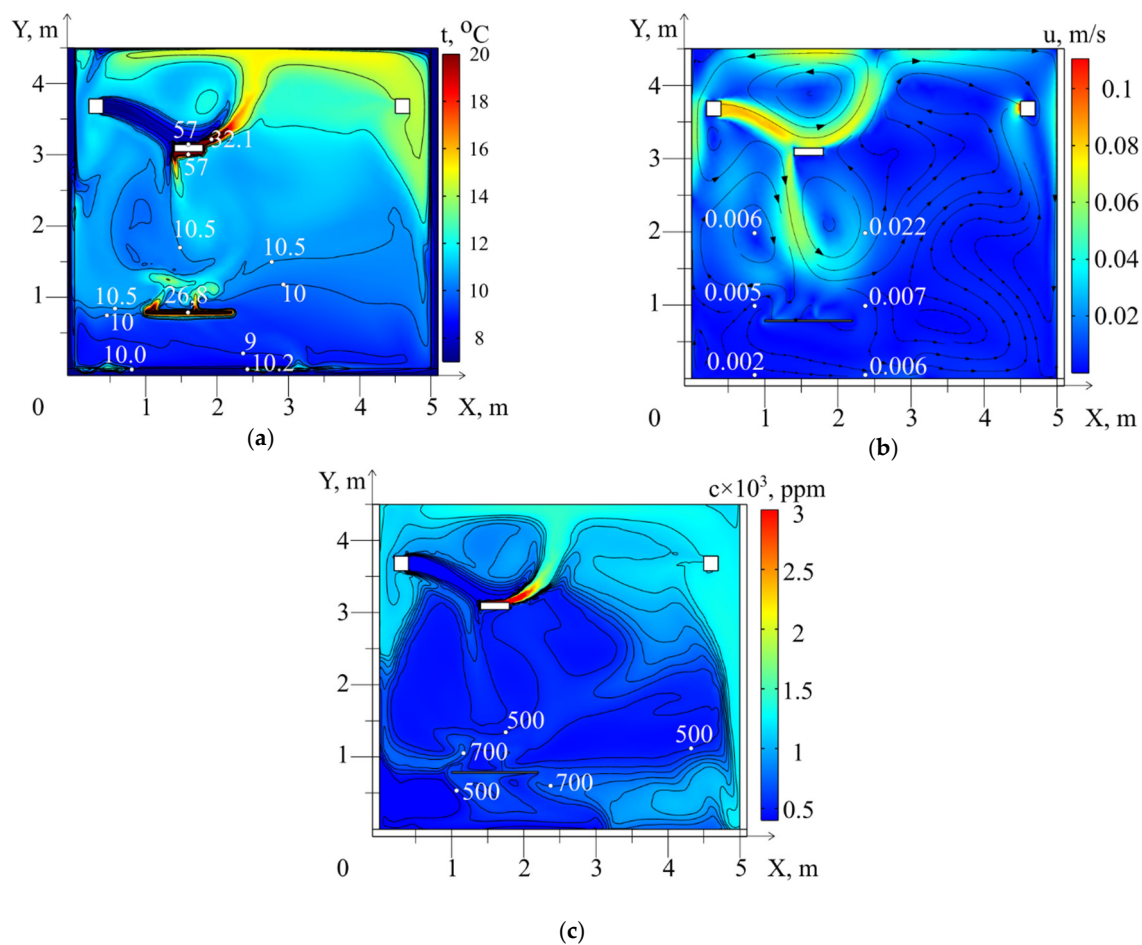
Figure 5. Fields of temperatures (a), air velocities (b) and CO 2 concentrations (c), formed by the 60th minute of the GIH operation at an airflow rate of 0.02 kg/s ( 9.09 \times 10^{-5} kg/(s \times m 3 )).
