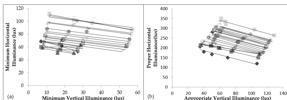
Figure 7. Variation of (a) minimum horizontal illuminance and (b) proper horizontal illuminance with vertical illuminance. Each line represents the value of adjusted horizontal illumination for each subject.
