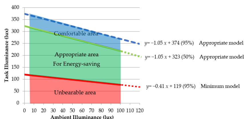
Figure 9. Energy-saving area for task illuminance in different ambient lighting space.
