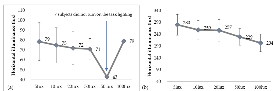
Figure 6. Horizontal illuminance varied with surrounding illuminance: (a) minimum horizontal illuminance and (b) appropriate horizontal illuminance.
