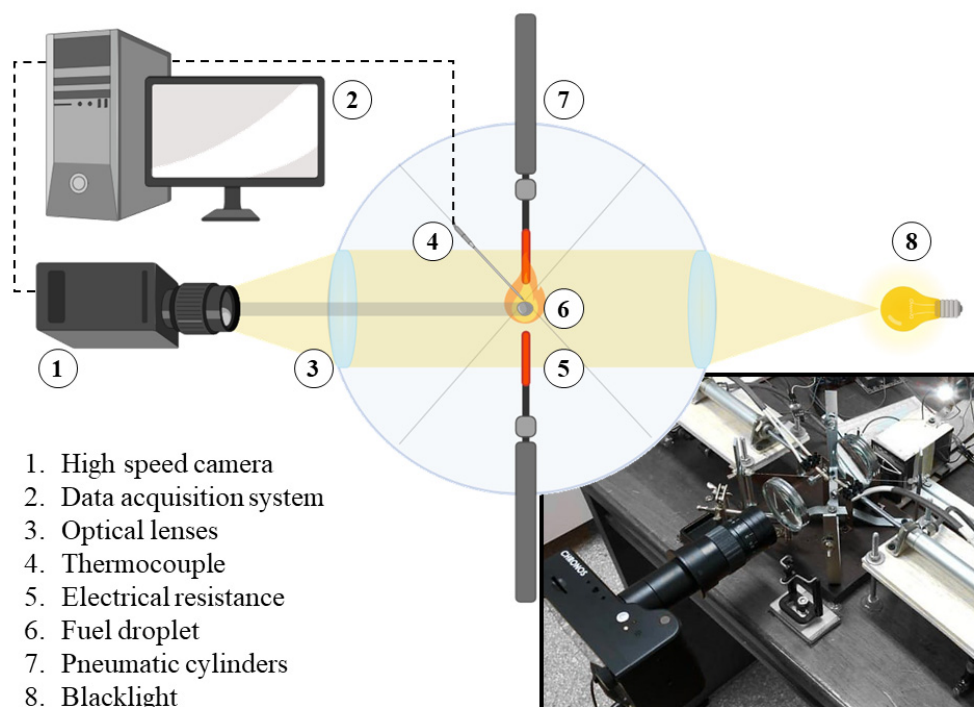
Figure 3. Schematic representation and experimental setup of droplet combustion.
