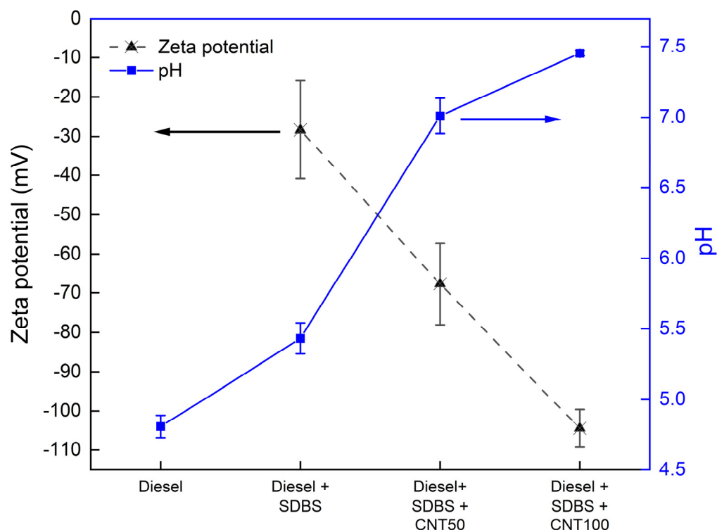
Figure 5. Zeta potential and pH measurements after nanofuels preparation at a CNT concentration of 100 ppm.
