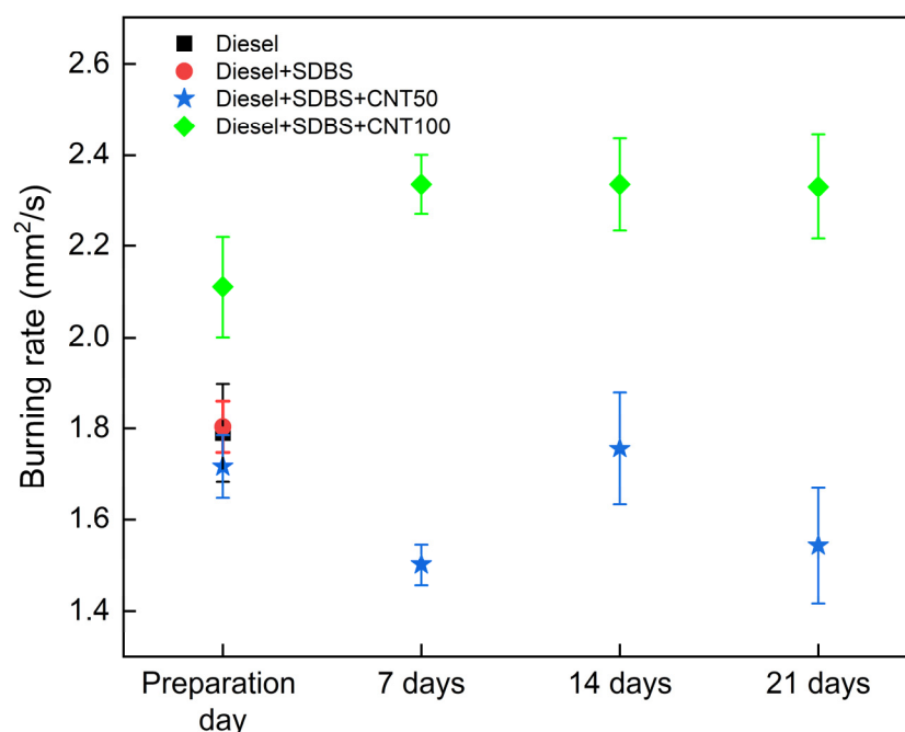
Figure 10. Effect of the CNT and SDBS nanofuels' temporal stability on the diesel droplet burning rate at CNT concentrations of 50 ppm and 100 ppm.
