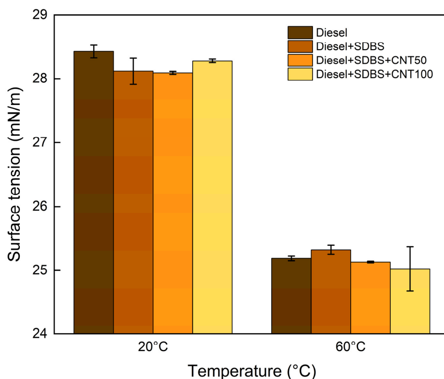
Figure 7. Surface tension of nanofuels at 20 °C and 60 °C after preparation with CNTs at 50 ppm and 100 ppm stabilized with SDBS.
