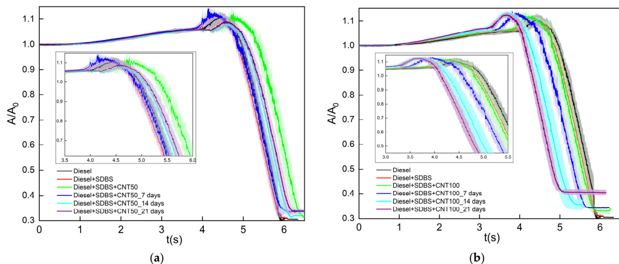
Figure 8. Evolution of the normalized area of nanofuels during droplet combustion with diesel, SDBS, and CNTs at concentrations of (a) 50 ppm and (b) 100 ppm.
