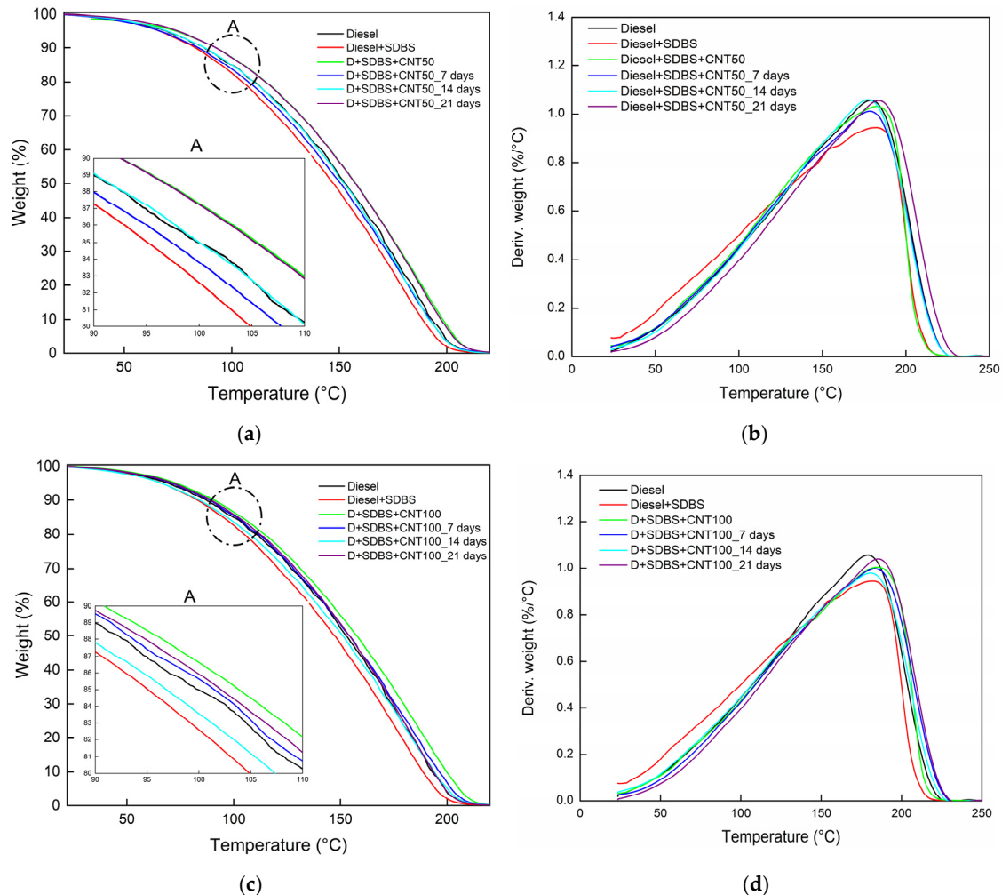
Figure 11. Temporal thermogravimetric analysis of diesel, SDBS, and CNT blends at concentrations of 50 ppm (a,b) and 100 ppm (c,d). Circle A (in (a,c)) indicates an expanded region in the miniature detail graphs.
