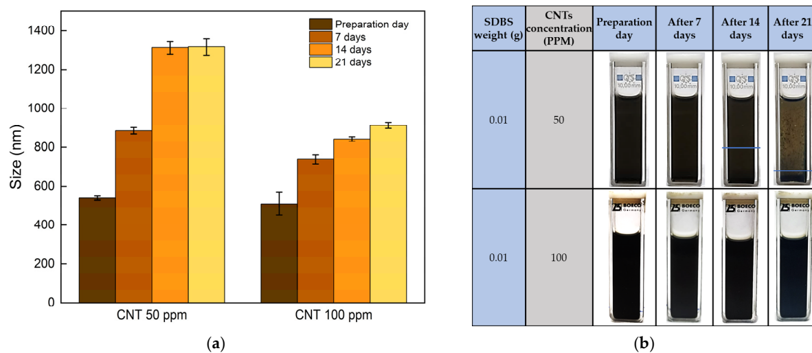
Figure 4. Characterization of the hydrodynamic size of CNTs in the nanofuels. (a) DLS results and (b) visual inspection for different days after nanofuels preparation. The size increases because CNT nanomaterials were agglomerating inside the fuel over the days, which causes sedimentation.
