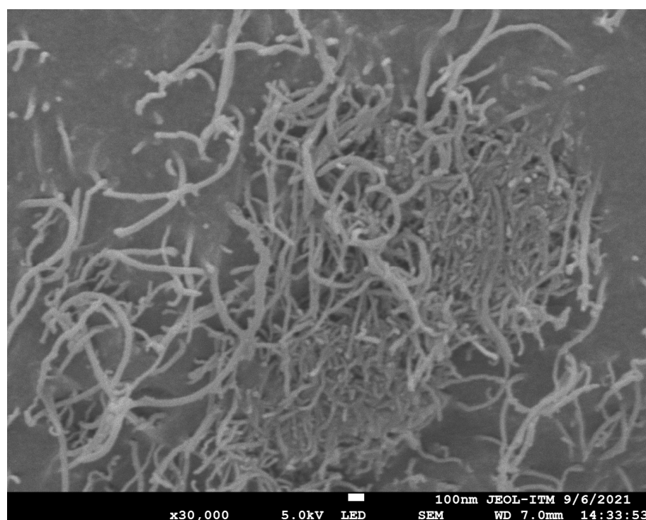
Figure 1. SEM images of CNT nanoparticles.
