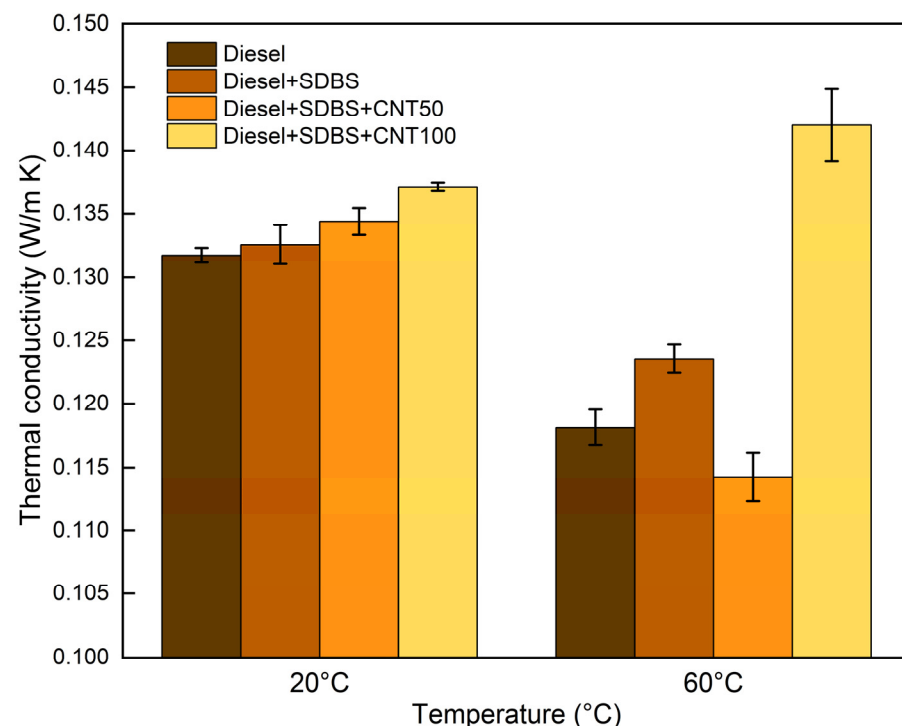
Figure 6. Thermal conductivity of nanofuels at 20 °C and 60 °C after preparation with CNTs at 50 ppm and 100 ppm, stabilized with SDBS.
