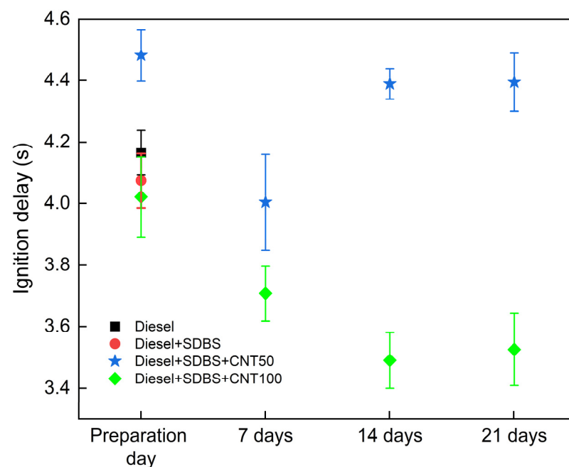
Figure 9. Temporal analysis of the ignition delay of nanofuels during droplet combustion with diesel, SDBS, and CNTs at concentrations of 50 ppm and 100 ppm.
