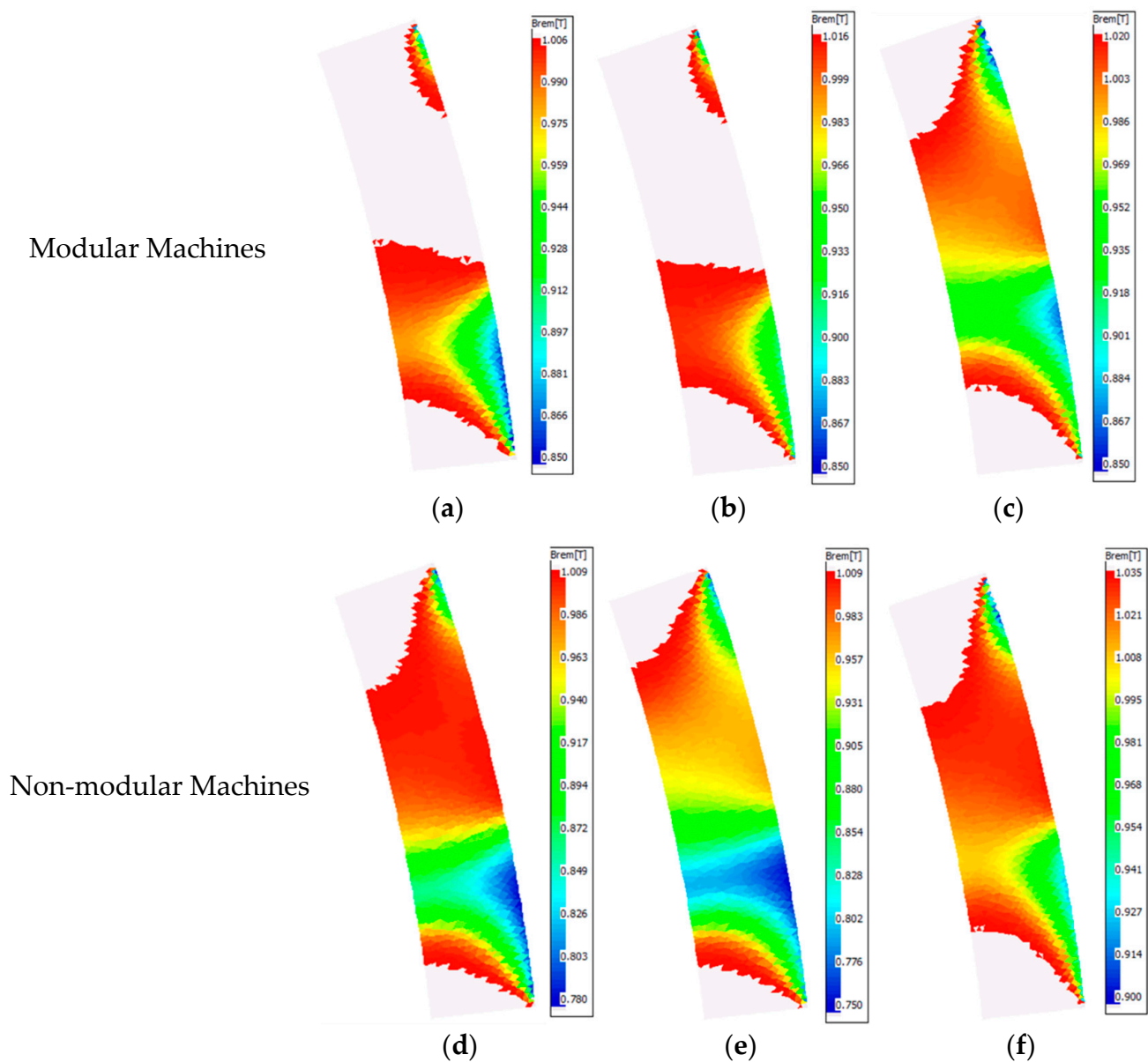
Figure 18. Remanence distribution of the PM obtained using the coupled EM-thermal model of Motor-CAD for (a) condition 1, T_{m'} = 160\text{ }^{\circ}\text{C} ; (b) condition 2, T_{m'} = 153\text{ }^{\circ}\text{C} ; (c) condition 3, T_{m'} = 150\text{ }^{\circ}\text{C} ; (d) condition 1, T_{m'} = 158\text{ }^{\circ}\text{C} ; (e) condition 2, T_{m'} = 148\text{ }^{\circ}\text{C} ; and (f) condition 3, T_{m'} = 140\text{ }^{\circ}\text{C} .
