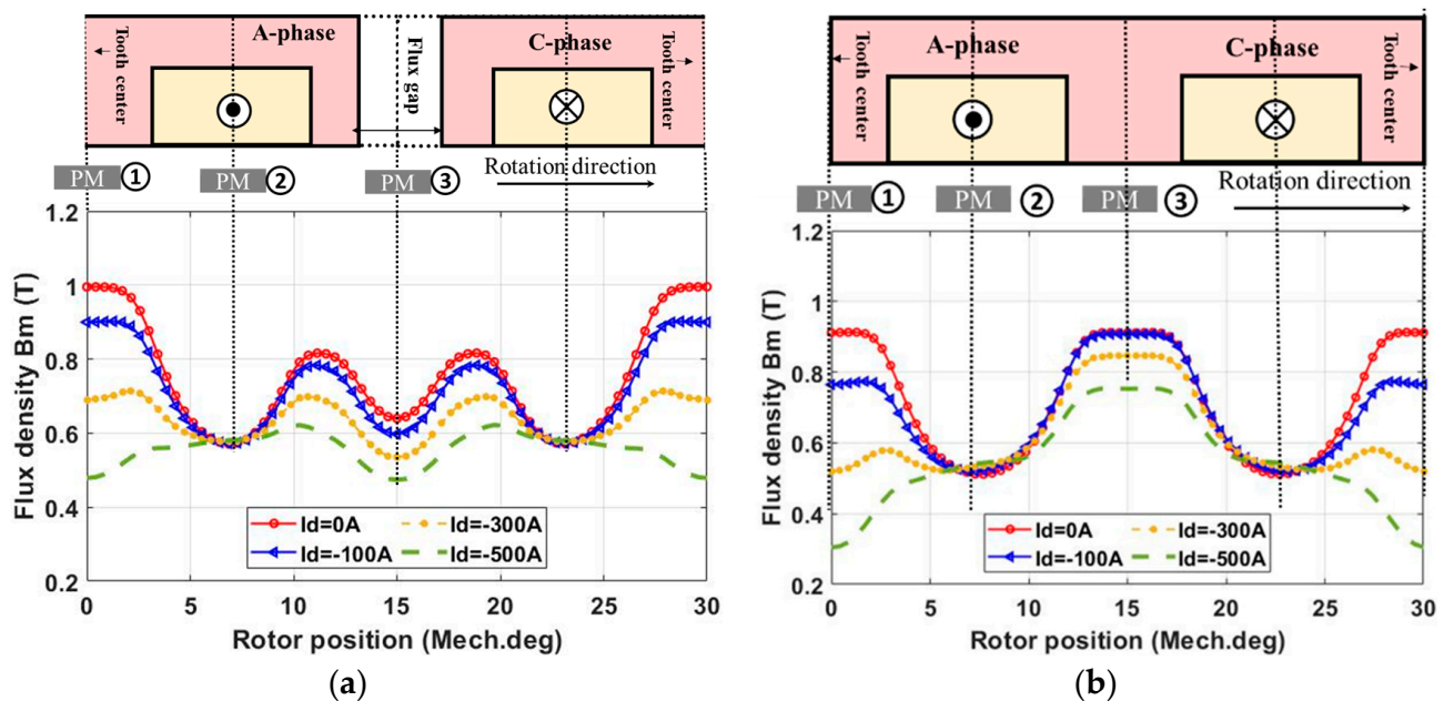
Figure 8. Magnet flux density (radial component) at 20 °C at point A for the (a) modular and (b) non-modular machines.
