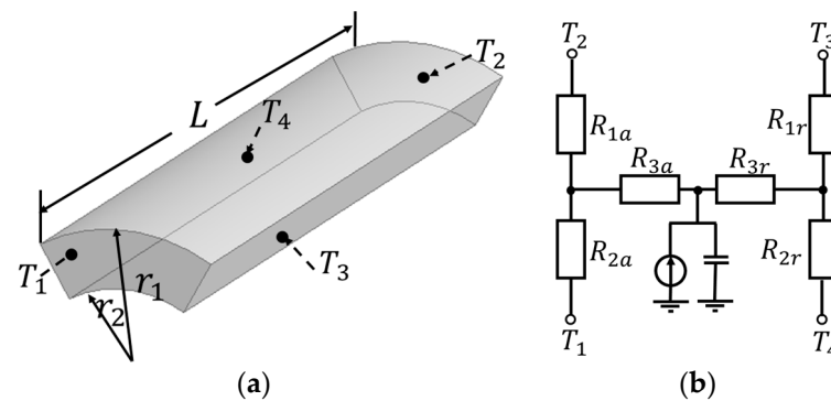
Figure 15. (a) Cylindrical components in electrical machines with angular spans \alpha and (b) its equivalent thermal network. T_1 , T_2 , T_3 and T_4 are the temperatures of the front, rear, outer and inner surfaces, respectively.
