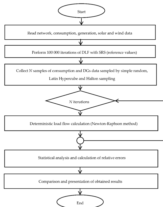
Figure 8. Scheme of probabilistic load flow algorithm.
