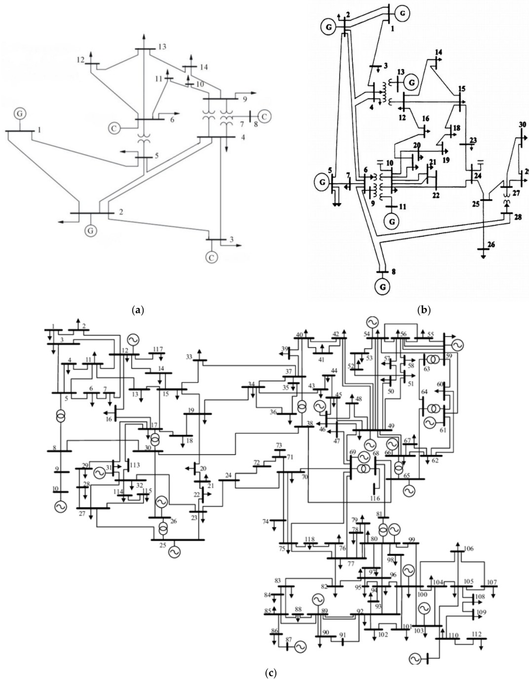
Figure 3. Configuration of IEEE (a) 14 bus system; (b) 30 bus system; and (c) 118 bus system.
