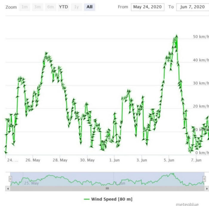
Figure 4. Wind speed graph for the chosen time period.
