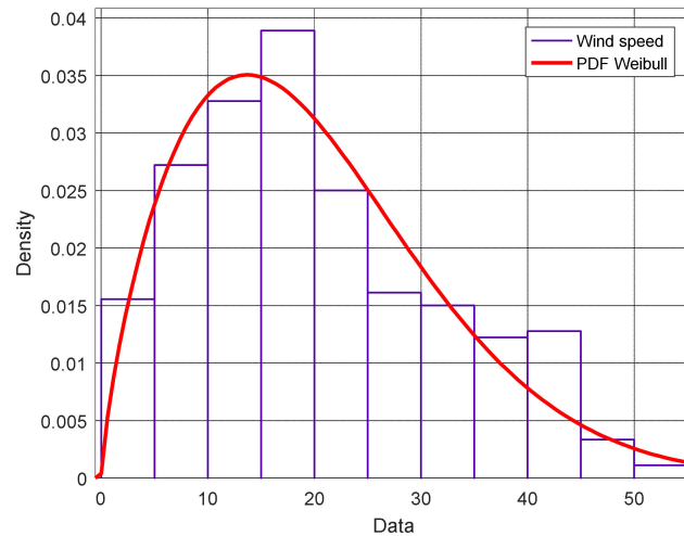
Figure 5. Histogram and modelled wind speed probability density distribution function.
