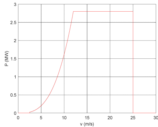
Figure 7. The dependence of output power of wind generator on wind speed.
