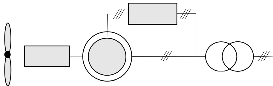
Figure 6. Wind turbine with doubly fed induction generator.
