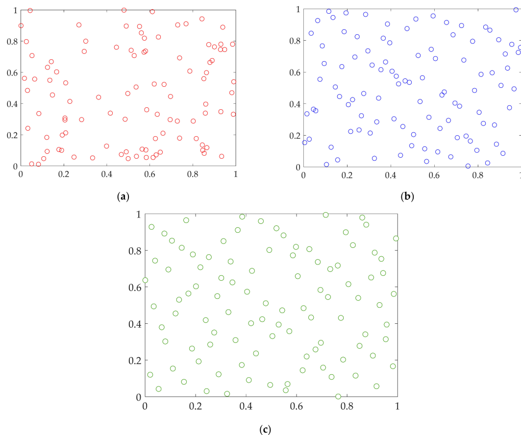
Figure 2. Comparison of 100 samples obtained by: (a) simple random sampling; (b) Latin Hypercube sampling; and (c) Halton quasi-random sampling.
