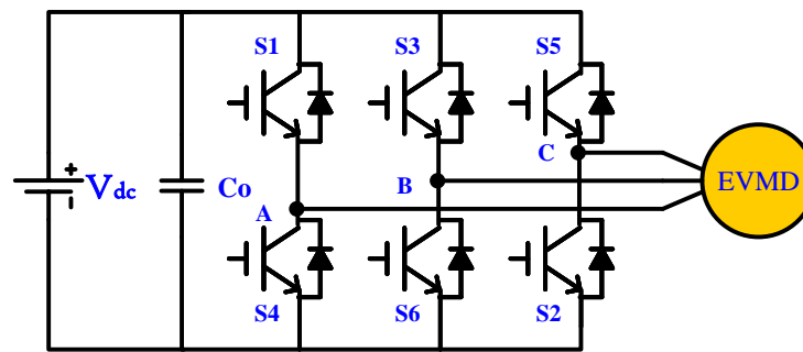
Figure 2. Three-Phase Two-Level Inverter (TLI) Topology for EV Motor Drive.
