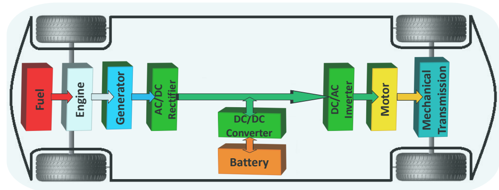
Figure 1. Various types of power electronics converters used in a typical series hybrid vehicle design system.
