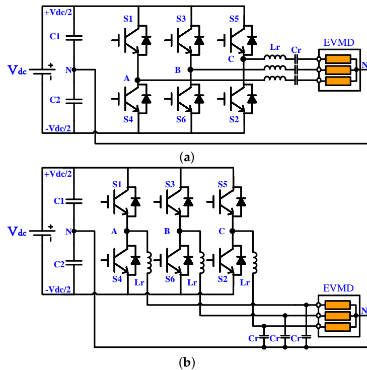
Figure 14. Load resonant DC-AC inverter (LRI) topology for EV motor drive. (a) Series-load resonant DC-AC inverter, and (b) Parallel-load resonant DC-AC inverter.
