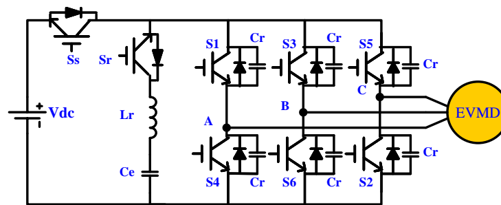
Figure 18. Three-phase quasi-resonant DC-AC inverter topology for EV motor drive.
