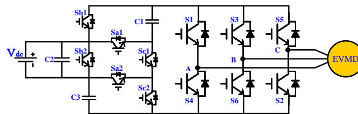
Figure 25. Three-phase seven-level switched-capacitor PWM inverter using series-parallel (SCI-S/P) conversion.
