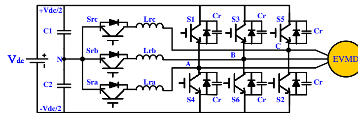
Figure 17. Three-phase resonant snubber (ZVT) DC-AC inverter topology for EV motor drive.
