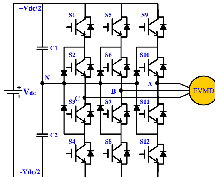
Figure 19. Three-phase three-level diode-clamped multilevel inverter (DC-MLI) for EV motor drive.
