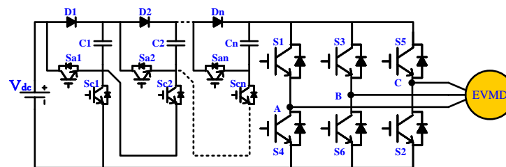
Figure 26. Three-phase hybrid multilevel inverter (HMLI-SC) using switched-capacitor for EV motor drive.
