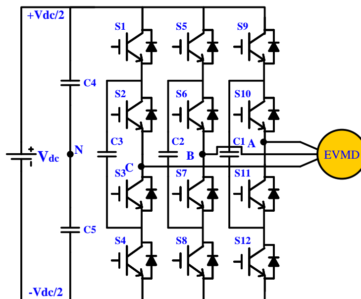
Figure 20. Three-phase three-levels flying-capacitor multilevel inverter (FC-MLI) topology for EV motor drive.
