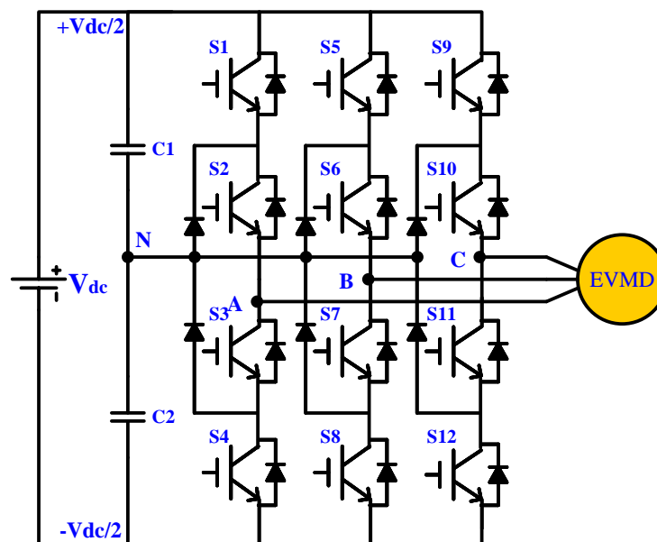
Figure 3. Three-phase three-Level topology of neutral point clamped multilevel inverter (NPC-MLI) for EV motor drive.
