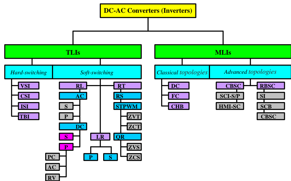
Figure 4. Classifications of the DC-AC inverters.
