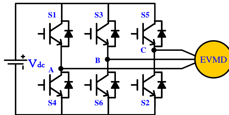
Figure 5. Three-phase voltage source inverter (VSI) topology.
