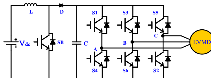
Figure 6. Three-phase current source inverter (CSI) topology.
