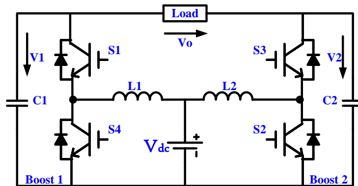
Figure 8. Single-phase two boost inverter (TBI) topology.
