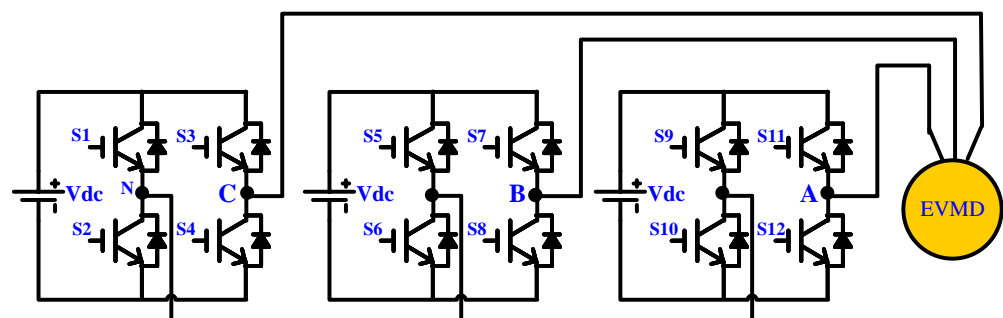
Figure 21. Three-phase three-level topology of cascaded H-bridge multilevel inverter (CHB-MLI) for EV motor drive.
