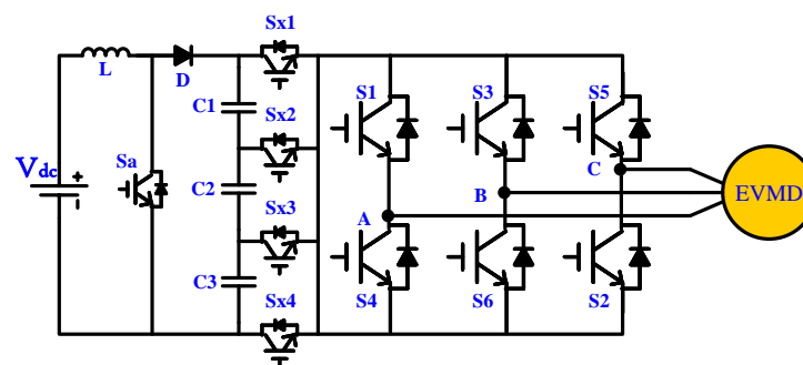
Figure 23. Three-phase seven-level switched-inductor multilevel inverter (SI-MLI) for EV motor drive.
