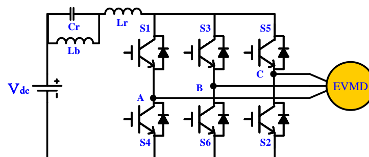
Figure 10. Series Resonant DC-link Inverter (SRDCLI) Topology for EV Motor Drive.
