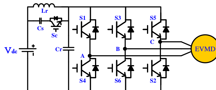
Figure 12. Active Clamp Resonant DC-Link Inverter (ACRDCLI) Topology for EV Motor Drive.
