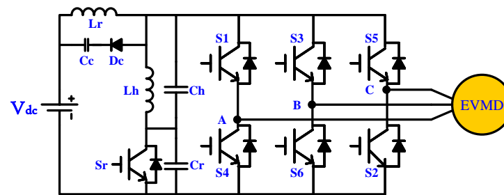
Figure 13. Reduced voltage resonant DC-link inverter (RVRDCLI) for EV motor drive.
