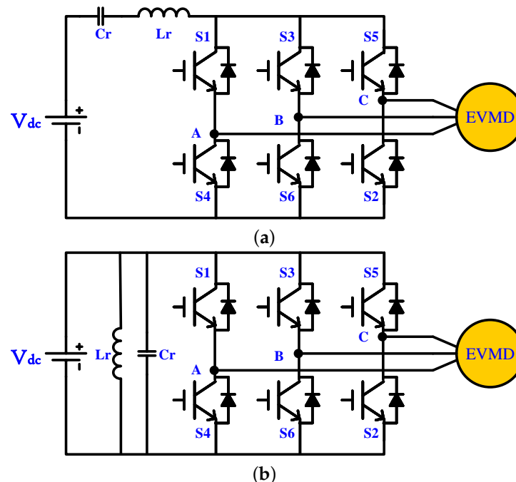
Figure 9. Resonant AC-link inverter for EV motor drive. (a) Series resonant AC-link, (b) Parallel resonant AC-link.
