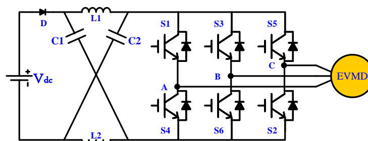
Figure 7. Three-phase impedance source inverter (ISI) topology.
