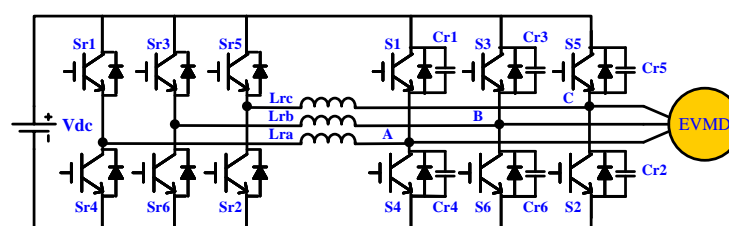
Figure 15. Three-phase zero voltage transition (ZVT) inverter topology for EV motor drive.
