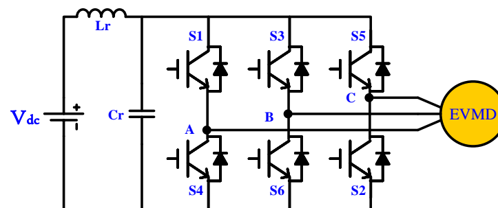
Figure 11. Parallel resonant DC-link inverter (PRDCLI) topology for EV motor drive.
