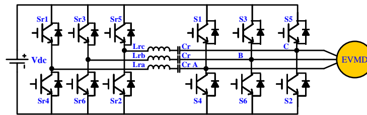
Figure 16. Three-phase zero-current transition (ZCT) inverter topology for EV motor drive.
