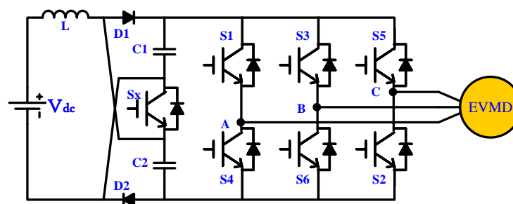
Figure 22. Three-phase five-level cascaded switched-capacitor multilevel boost inverter (CBSC-MLI) for EV motor drive.
