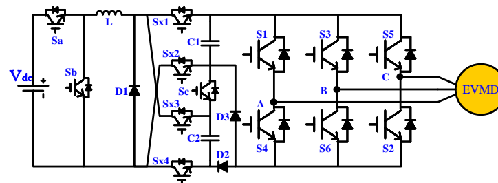
Figure 24. Three-phase thirteen-level switched-capacitor multilevel boost inverter (SCB-MLI) with partial charging.
