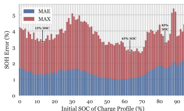
Figure 9. MAE and MAX values of SOH estimation performed over charge profiles beginning at various SOC values. The partial charge profiles are obtained from the NASA prognostics repository and are about 43 min long. The stated ranges of the partial profiles are ranges of the new battery cell before it has aged.
