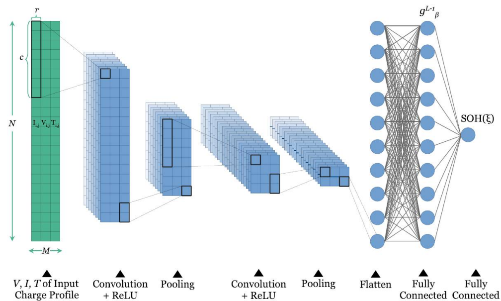
Figure 1. Architecture of a convolutional neural network (CNN) where each layer is composed of a convolution and pooling component and with the last two layers being fully connected. The input data is given by \Psi(\xi) \in \mathbb{R}^{N \times M} where N = 256 and M = 3 since \Psi(\xi) = [I(\xi); V(\xi); T(\xi)] where I, V and T represent the current, voltage and temperature of the charge curve. The output of the CNN is the estimated SOH.
