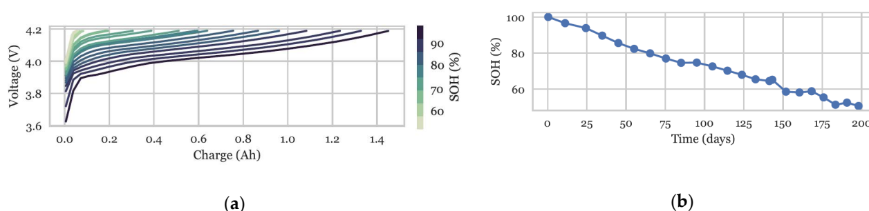
Figure 2. (a) CC segment of charge profile of a Li-ion cell throughout randomized usage aging process; color spectrum of profiles indicate SOH. (b) Recorded capacity-based SOH for each of the charge profiles in (a).
