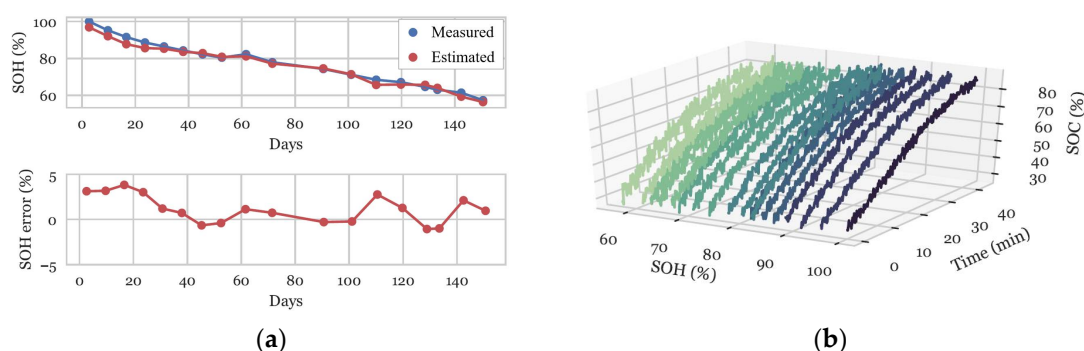
Figure 7. (a) CNN SOH estimation and error for partial charge curve input beginning at 30% SOC and ending at about 85% SOC. (b) Partial charge profiles beginning at 30% SOC and ending at about 85% SOC.
