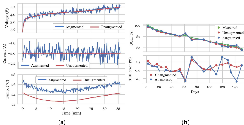
Figure 6. (a) Augmented and unaugmented voltage, current and temperature signals of validation dataset. (b) Estimation accuracy and error for augmented and unaugmented battery validation data. Please see Table 4 for detailed results.
