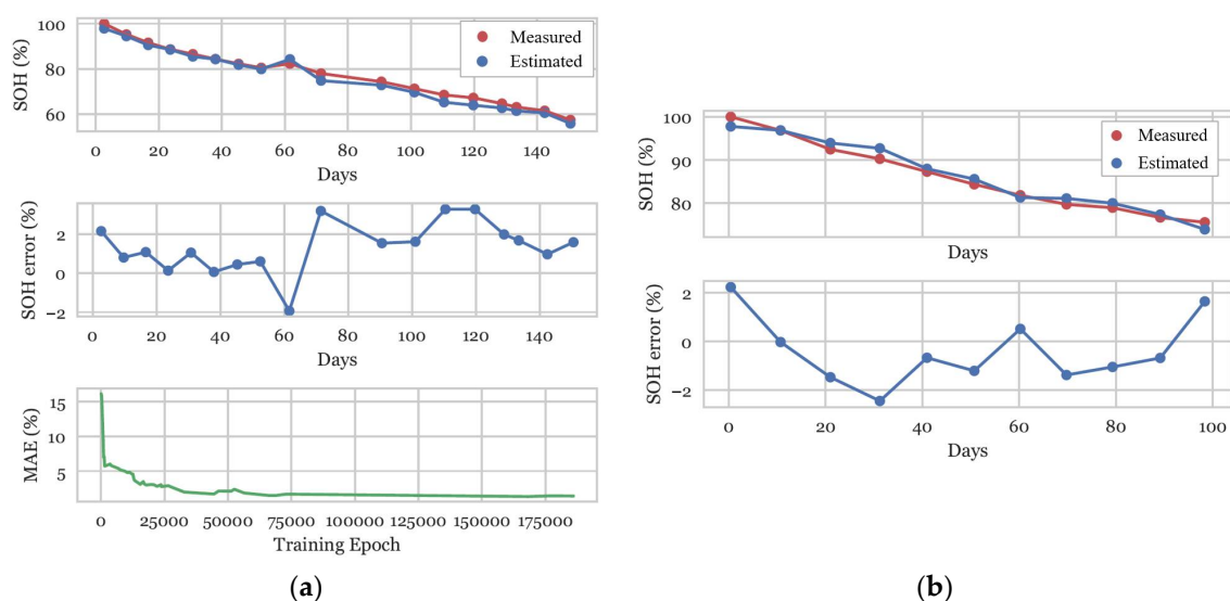
Figure 4. (a) From top to bottom, CNN estimation accuracy, estimation error over the 25 °C validation dataset and the mean absolute error as a function of training epochs. (b) Estimation accuracy and estimation error over 40 °C validation dataset.
