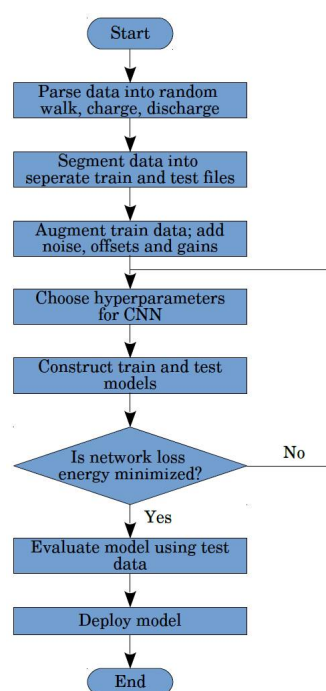
Figure 3. Flowchart describing data preprocessing, data augmentation and model training steps. Each of the datasets are constructed by extracting the reference charge profiles from the raw data. After preprocessing, the 28 datasets are split into train and testing datasets. The train set is then augmented as described in Section 3 before training begins. Please refer to text for more details.
