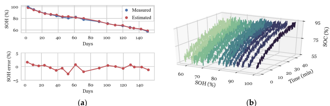
Figure 8. (a) CNN SOH estimation and error for partial charge curve input beginning at 60% SOC and ending at about 92% SOC. (b) Partial charge profiles beginning at 60% SOC and ending at about 92% SOC.
